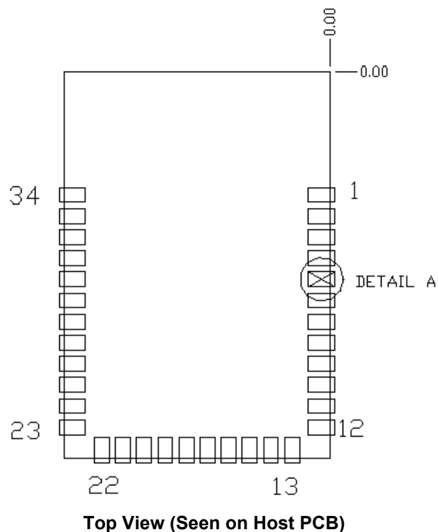
Figure 7. Solder Pad Reference Location
