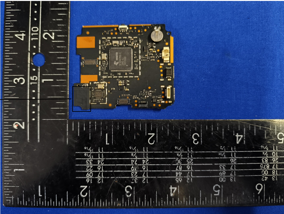
WIFI PCB antenna
