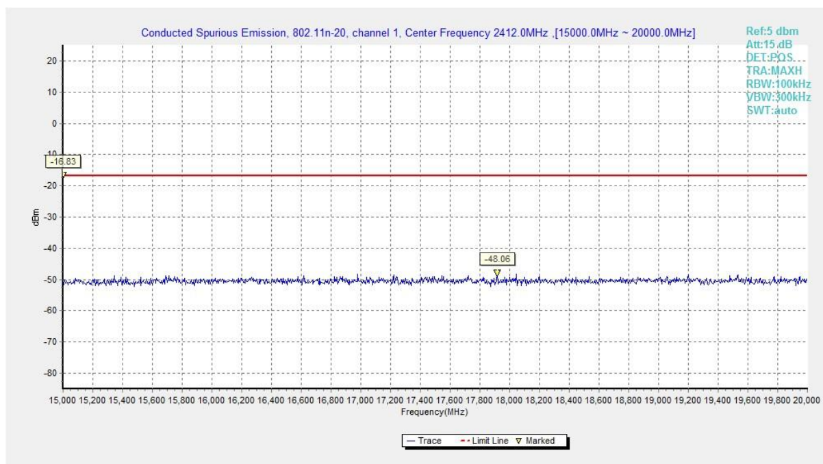
Fig.A.6.1.87 Conducted Spurious Emission (802.11n-HT20, Ch1, 15 GHz-20 GHz)
