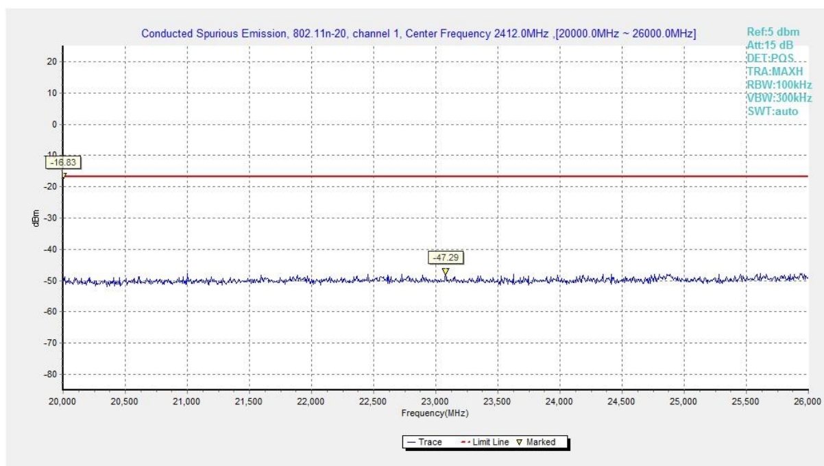
Fig.A.6.1.88 Conducted Spurious Emission (802.11n-HT20, Ch1, 20 GHz-26 GHz)
