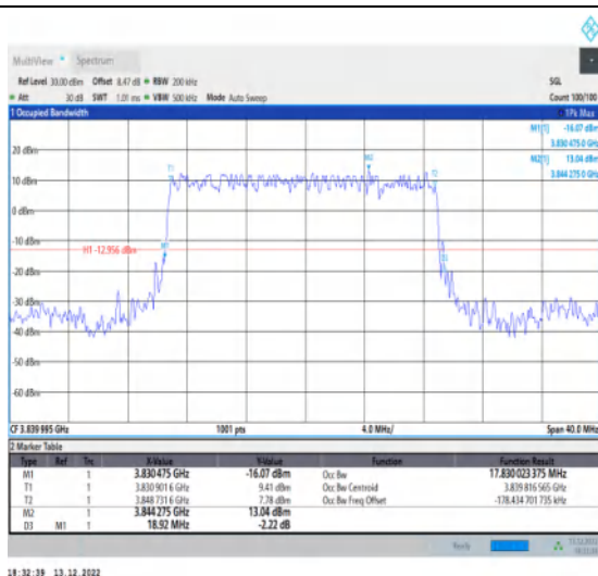
1-N77-3700-3980-30-20-M-2-DFT-PI2BPSK-Outer_F ull-50@0-Ant1-17.83-18.920-≤20-PASS
