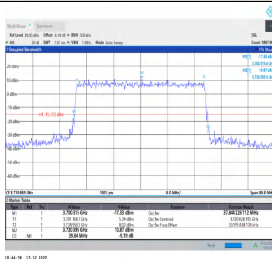
1-N77-3700-3980-30-40-L-8-CP-64QAM-Outter_Full-106@0-Ant1-37.844-39.840-≤40-PASS
