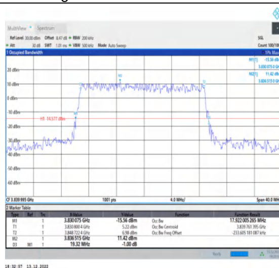
1-N77-3700-3980-30-20-M-3-DFT-16QAM-Outer_Ful l-50@0-Ant1-17.922-19.320-≤20-PASS
