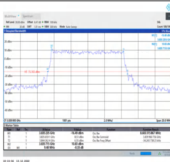
1-N77-3700-3980-30-10-M-3-DFT-16QAM-Outer_Full -24@0-Ant1-8.603-9.480-≤10-PASS
