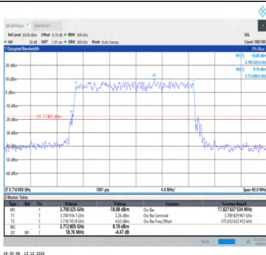
1-N77-3700-3980-30-20-L-5-DFT-256QAM-Outer_Fu II-50@0-Ant1-17.828-18.760-≤20-PASS
