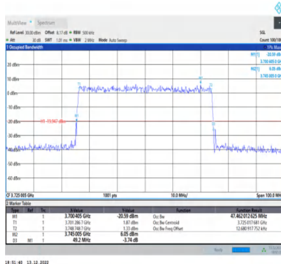
1-N77-3700-3980-30-50-L-9-CP-256QAM-Outer_Full-133@0-Ant1-47.462-49.200-≤50-PASS
