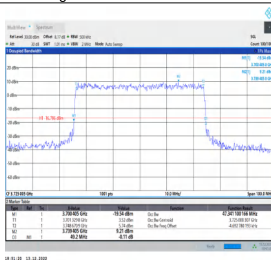
1-N77-3700-3980-30-50-L-7-CP-16QAM-Outer_Full-133@0-Ant1-47.341-49.200-≤50-PASS
