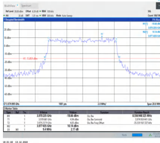
1-N77-3700-3980-30-10-H-4-DFT-64QAM-Outer_Ful I-24@0-Ant1-8.557-9.400-≤10-PASS
