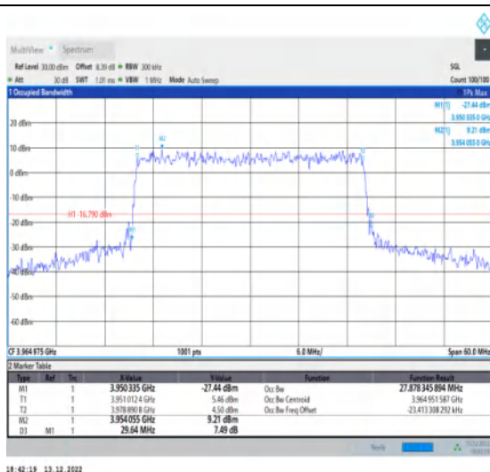
1-N77-3700-3980-30-30-H-6-CP-QPSK-Outer_Full-7 8@0-Ant1-27.878-29.640-≤30-PASS
