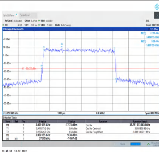
1-N77-3700-3980-30-40-H-5-DFT-256QAM-Outer_F ull-100@0-Ant1-35.751-37.920-≤40-PASS
