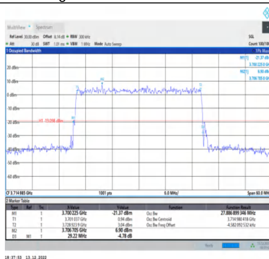
1-N77-3700-3980-30-30-L-9-CP-256QAM-Outer_Full-78@0-Ant1-27.887-29.220-≤30-PASS
