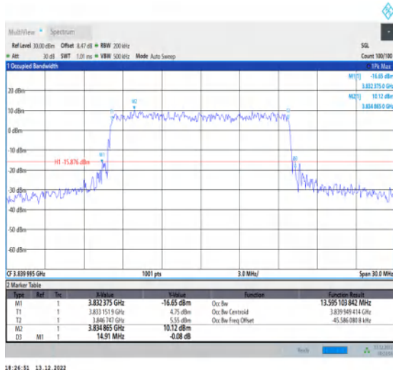
1-N77-3700-3980-30-15-M-7-CP-16QAM-Outer_Full-38@0-Ant1-13.595-14.910-≤15-PASS
