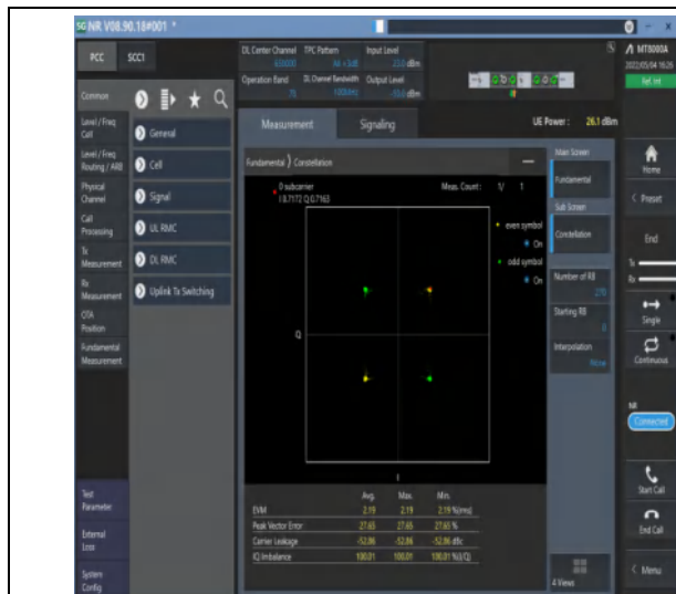
1-N78-3700-3800--30-100-M-1-DFT-PI2BPSK-Outertest_Full-270@0-Ant1-see graph-PASS
