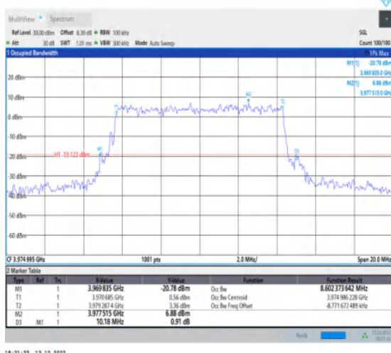
1-N77-3700-3980-30-10-H-5-DFT-256QAM-Outer_F ull-24@0-Ant1-8.602-10.180-≤10-PASS
