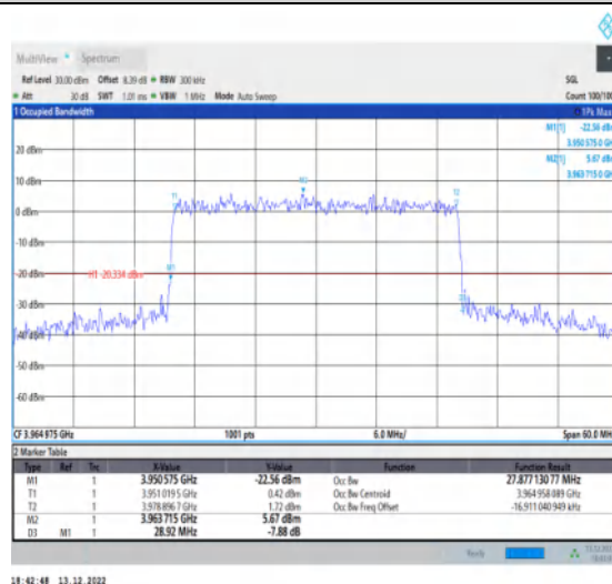
1-N77-3700-3980-30-30-H-9-CP-256QAM-Outer_Full-78@0-Ant1-27.877-28.920-≤30-PASS
