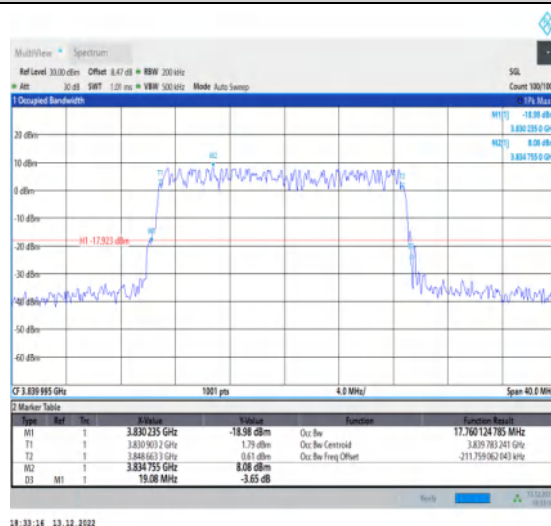
1-N77-3700-3980-30-20-M-5-DFT-256QAM-Outer_F ull-50@0-Ant1-17.76-19.080-≤20-PASS
