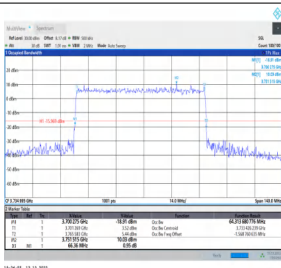
1-N77-3700-3980-30-70-L-4-DFT-64QAM-Outer_Full -180@0-Ant1-64.314-66.360-≤70-PASS
