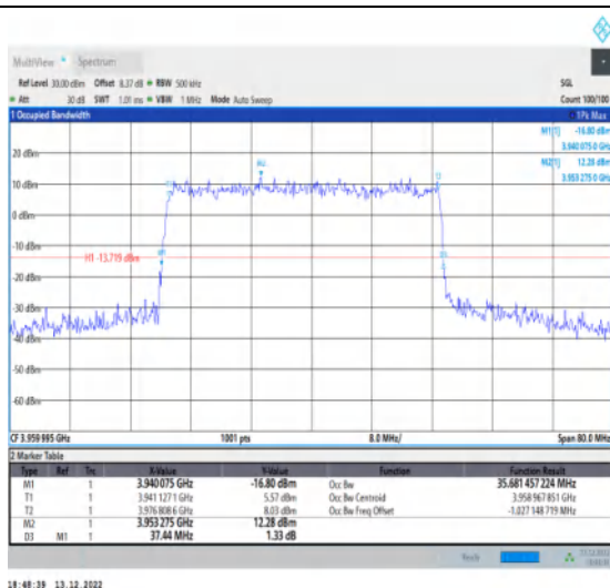
1-N77-3700-3980-30-40-H-3-DFT-16QAM-Outer_Ful I-100@0-Ant1-35.681-37.440-≤40-PASS
