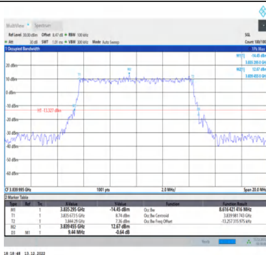
1-N77-3700-3980-30-10-M-2-DFT-PI2BPSK-Outer_Full -24@0-Ant1-8.616-9.440-≤10-PASS
