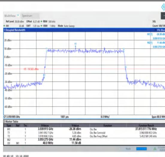
1-N77-3700-3980-30-40-H-6-CP-QPSK-Outer_Full-1 06@0-Ant1-37.816-40.000-≤40-PASS
