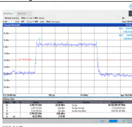
1-N77-3700-3980-30-70-L-5-DFT-256QAM-Outer_Full -180@0-Ant1-64.182-66.220-≤70-PASS
