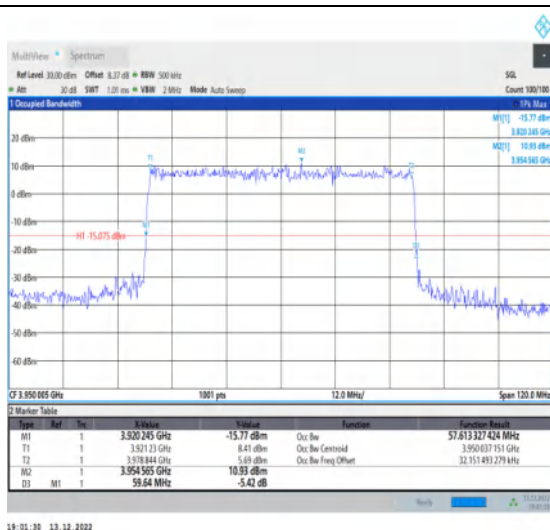
1-N77-3700-3980-30-60-H-1-DFT-QPSK-Outer_Full-162@0-Ant1-57.613-59.640-≤60-PASS
