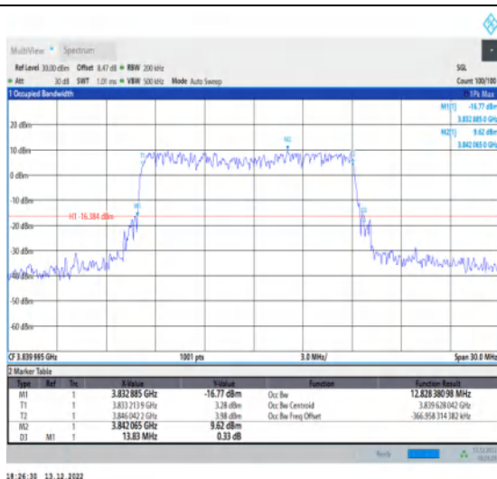
1-N77-3700-3980-30-15-M-5-DFT-256QAM-Outer_Full-36@0-Ant1-12.828-13.830-≤15-PASS
