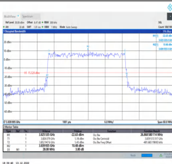
1-N77-3700-3980-30-30-M-5-DFT-256QAM-Outer_F ull-75@0-Ant1-26.869-28.080-≤30-PASS
