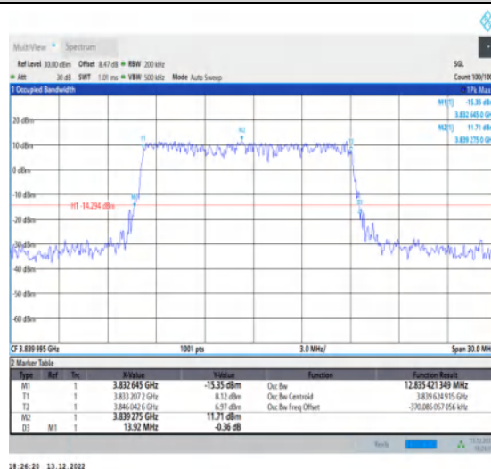
1-N77-3700-3980-30-15-M-4-DFT-64QAM-Out_FulI-36@0-Ant1-12.835-13.920-≤15-PASS
