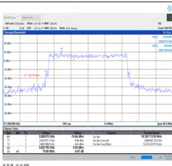
1-N77-3700-3980-30-20-M-6-CP-QPSK-Outter_Full-5 1@0-Ant1-18.183-19.680-≤20-PASS
