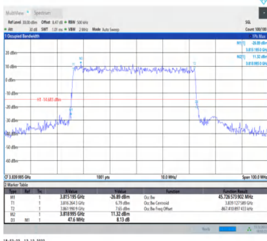
1-N77-3700-3980-30-50-M-3-DFT-16QAM-Outer_Full-128@0-Ant1-45.727-47.600-≤50-PASS
