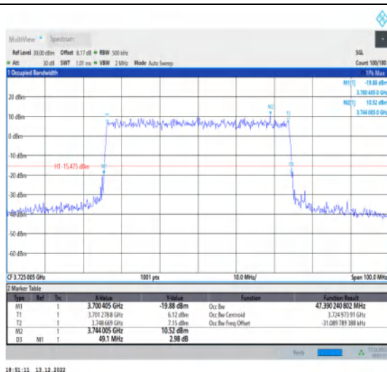
1-N77-3700-3980-30-50-L-6-CP-QPSK-Outer_Full-133@0-Ant1-47.39-49.100-≤50-PASS
