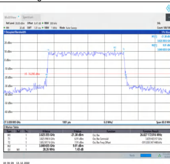
1-N77-3700-3980-30-30-M-4-DFT-64QAM-Outer_Ful I-75@0-Ant1-26.827-28.260-≤30-PASS
