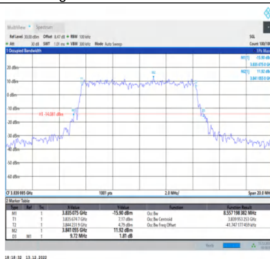
1-N77-3700-3980-30-10-M-1-DFT-QPSK-Outer_Full -24@0-Ant1-8.557-9.720-≤10-PASS
