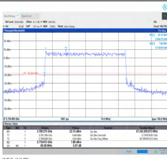
1-N77-3700-3980-30-70-L-6-CP-QPSK-Outer_Full-1 89@0-Ant1-67.342-69.580-≤70-PASS
