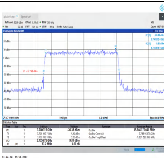
1-N77-3700-3980-30-40-L-5-DFT-256QAM-Outter_Fu II-100@0-Ant1-35.546-37.200-≤40-PASS
