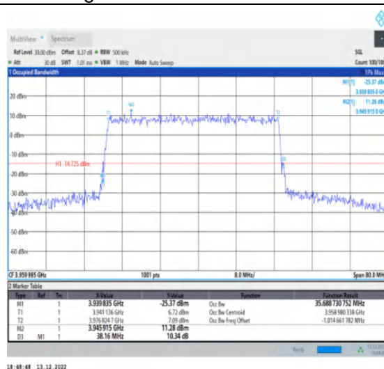
1-N77-3700-3980-30-40-H-4-DFT-64QAM-Outer_Ful I-100@0-Ant1-35.689-38.160-≤40-PASS
