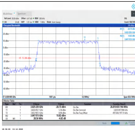
1-N77-3700-3980-30-30-M-3-DFT-16QAM-Outer_Ful I-75@0-Ant1-26.811-28.560-≤30-PASS
