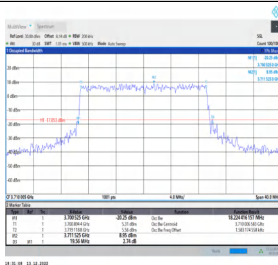
1-N77-3700-3980-30-20-L-6-CP-QPSK-Outer_Full-5 1@0-Ant1-18.224-19.560-≤20-PASS
