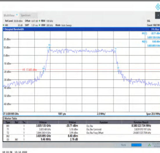
1-N77-3700-3980-30-10-M-6-CP-QPSK-Outer_Full-24@0-Ant1-8.58-9.460-≤10-PASS
