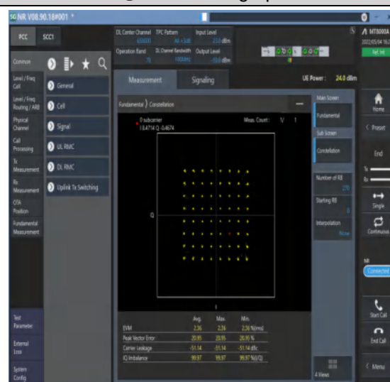
1-N78-3700-3800--30-100-M-4-DFT-64QAM-Outertest_Full-270@0-Ant1-see graph-PASS
