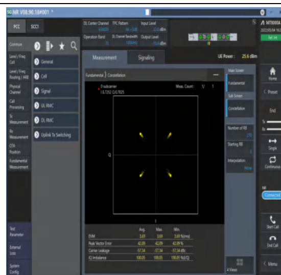
1-N78-3700-3800--30-100-M-2-DFT-QPSK-Outertest_Full-270@0-Ant1-see graph-PASS
