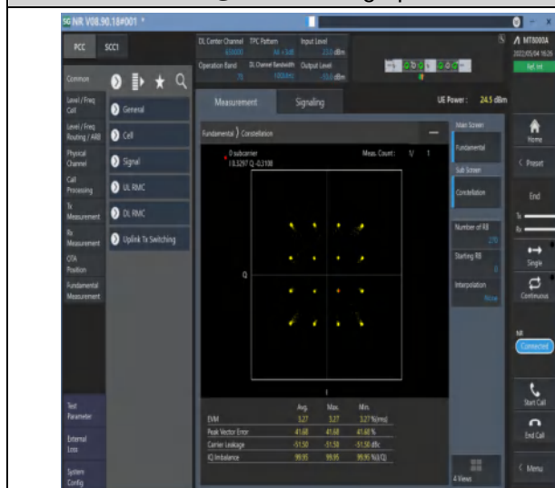
1-N78-3700-3800--30-100-M-3-DFT-16QAM-Outertest_Full-270@0-Ant1-see graph-PASS
