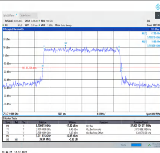
1-N77-3700-3980-30-40-L-7-CP-16QAM-Outter_Full-106@0-Ant1-37.905-39.840-≤40-PASS
