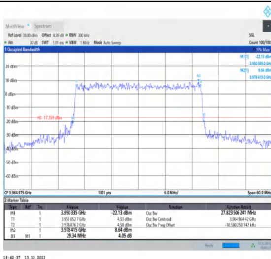
1-N77-3700-3980-30-30-H-8-CP-64QAM-Outer_Full-78@0-Ant1-27.824-29.340-≤30-PASS
