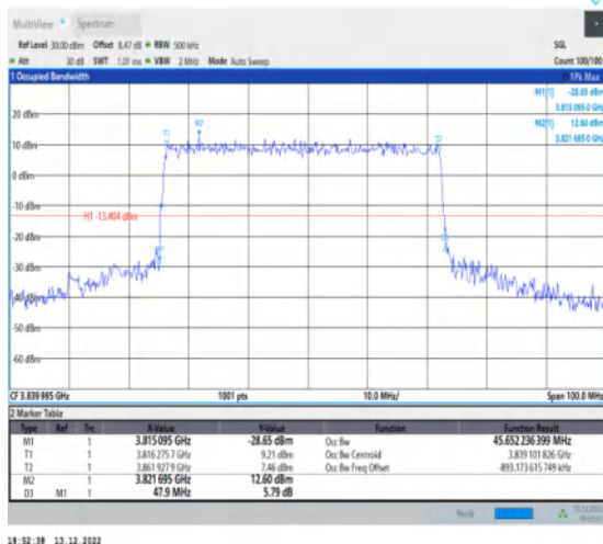
1-N77-3700-3980-30-50-M-1-DFT-QPSK-Outer_Full-128@0-Ant1-45.652-47.900-≤50-PASS
