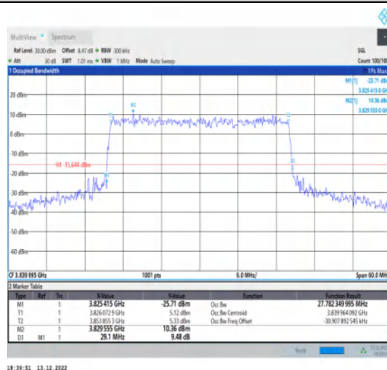
1-N77-3700-3980-30-30-M-6-CP-QPSK-Outer_Full-7 8@0-Ant1-27.782-29.100-≤30-PASS
