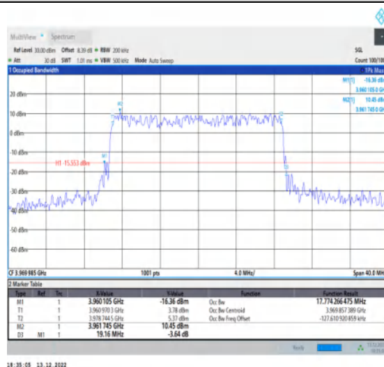
1-N77-3700-3980-30-20-H-4-DFT-64QAM-Outter_Full-50@0-Ant1-17.774-19.160-≤20-PASS
