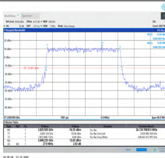
1-N77-3700-3980-30-30-M-2-DFT-PI2BPSK-Outer_Full-75@0-Ant1-26.725-27.900-≤30-PASS
