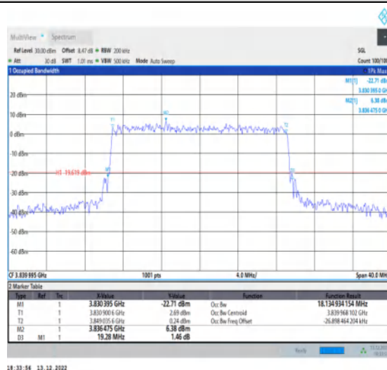
1-N77-3700-3980-30-20-M-9-CP-256QAM-Outter_Fu II-51@0-Ant1-18.135-19.280-≤20-PASS
