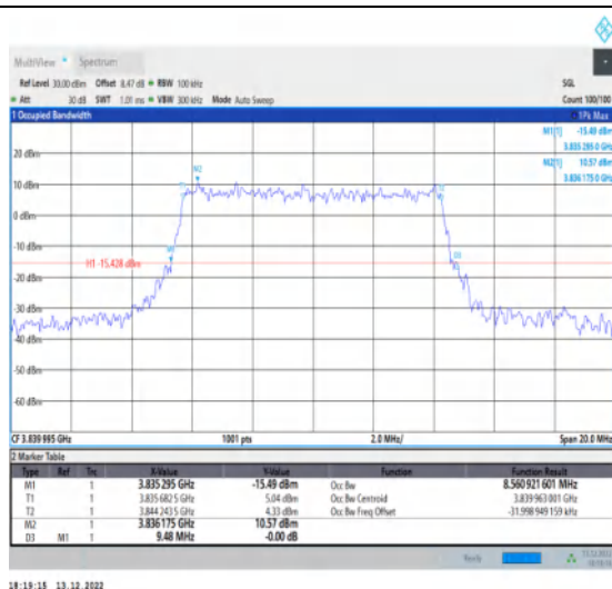
1-N77-3700-3980-30-10-M-4-DFT-64QAM-Outer_Full-I-24@0-Ant1-8.561-9.480-≤10-PASS
