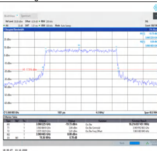
1-N77-3700-3980-30-20-H-6-CP-QPSK-Outer_Full-51@0-Ant1-18.216-19.360-≤20-PASS
