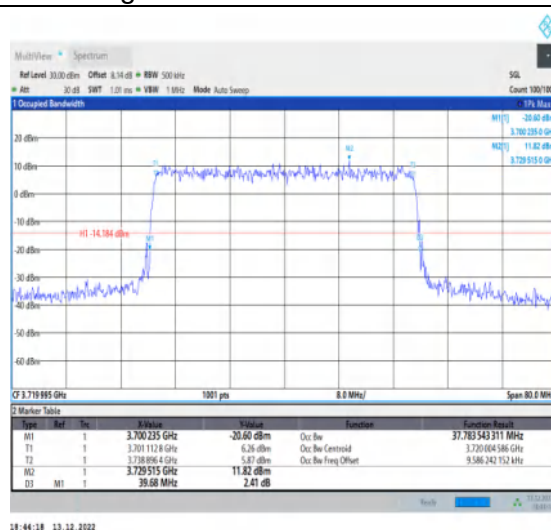
1-N77-3700-3980-30-40-L-6-CP-QPSK-Outter_Full-1 06@0-Ant1-37.784-39.680-≤40-PASS
