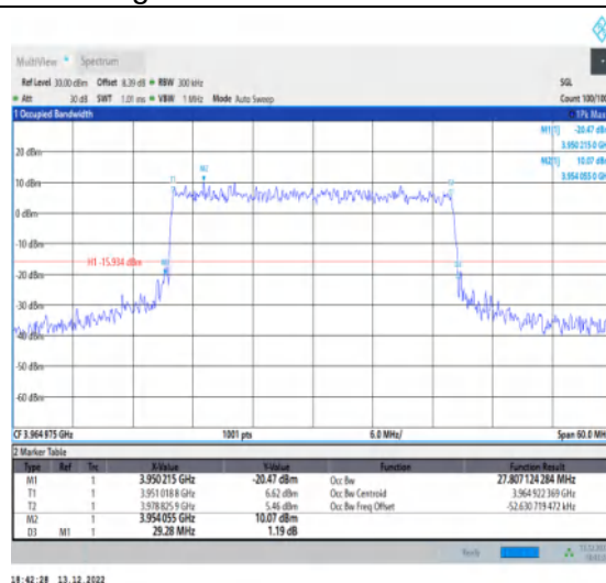
1-N77-3700-3980-30-30-H-7-CP-16QAM-Outer_Full-78@0-Ant1-27.807-29.280-≤30-PASS
