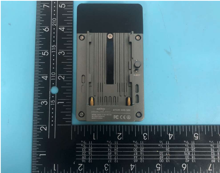
Photo 7 (Transmitter)
