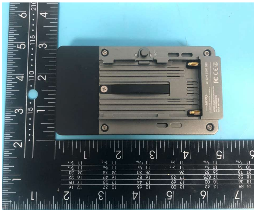
Photo 2 (Transmitter)
