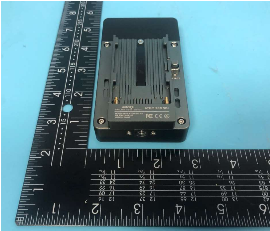
Photo 8 (Transmitter)
