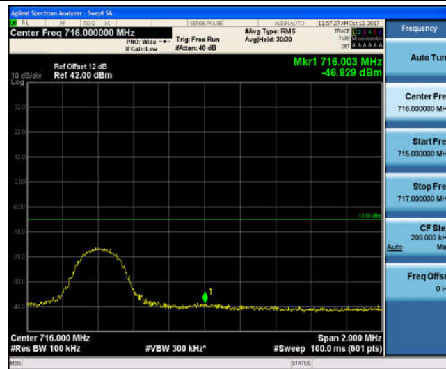
Band17_10MHz_QPSK_23800_50RB#0_-29.02_PASS
