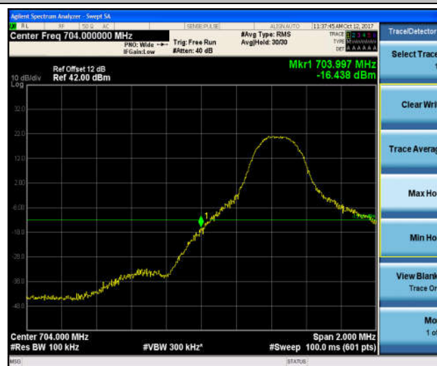
Band17_5MHz_16QAM_23755_1RB#0_-16.90_PASS
