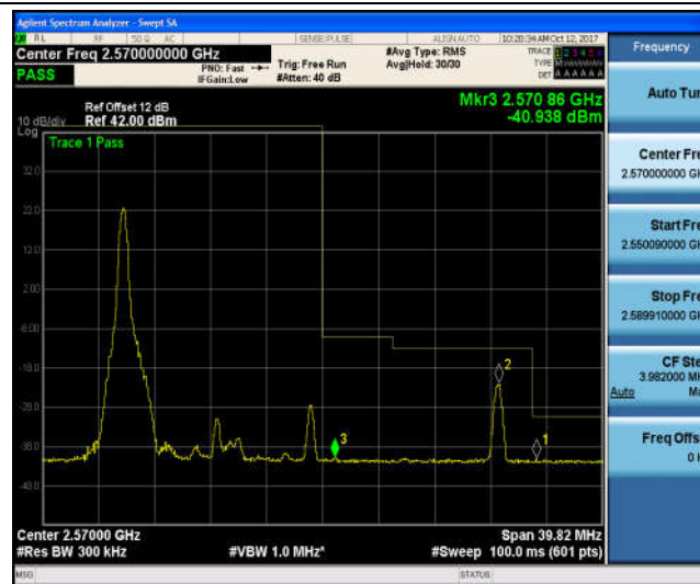
Band7_15MHz_QPSK_21375_75RB#0_-37.34,-21.82,-16.83_PASS
