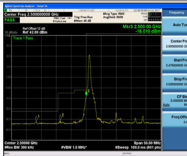
Band7_20MHz_16QAM_20850_1RB#0_-41.08,-38.21,-17.21_PASS
