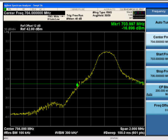
Band17_5MHz_QPSK_23755_25RB#0_-20.05_PASS
