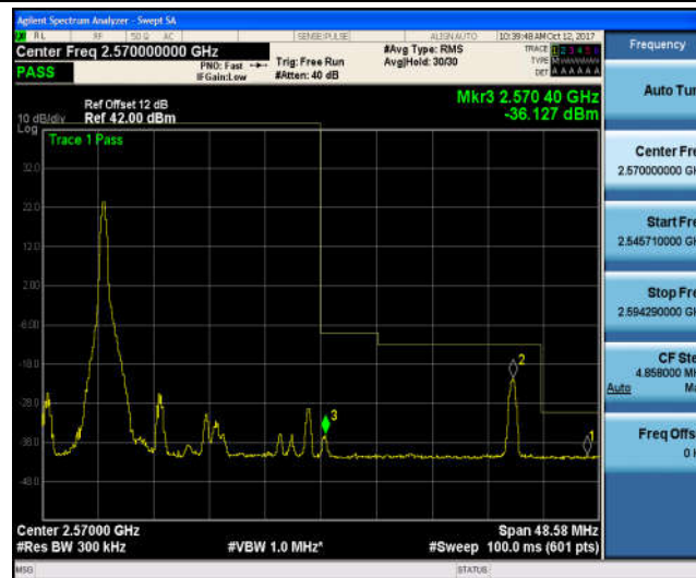
Band7_20MHz_16QAM_21350_1RB#0_-40.80,-22.19,-37.65_PASS
