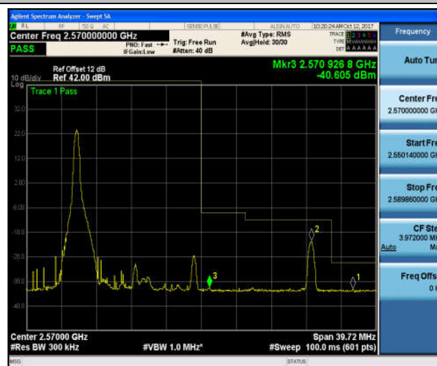
Band7_15MHz_16QAM_21375_1RB#0_-41.12,-22.08,-40.94_PASS
