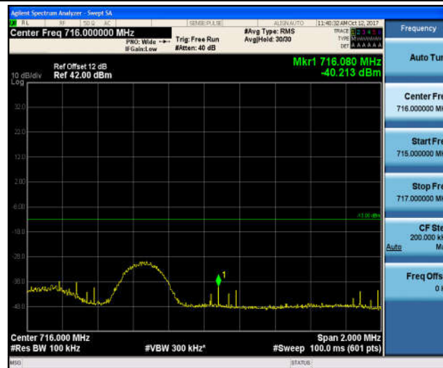
Band17_5MHz_QPSK_23825_25RB#0_-22.62_PASS
