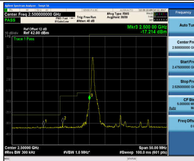
Band7_20MHz_QPSK_20850_100RB#0_-31.40,-27.72,-25.99_PASS
