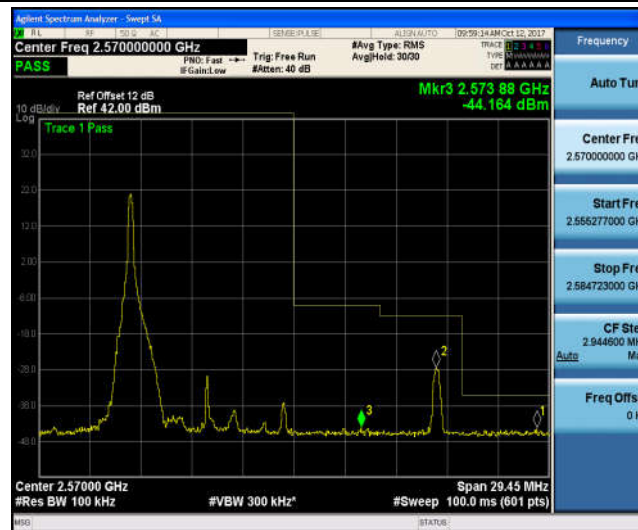
Band7_10MHz_QPSK_21400_50RB#0_-40.14,-32.13,-24.94_PASS
