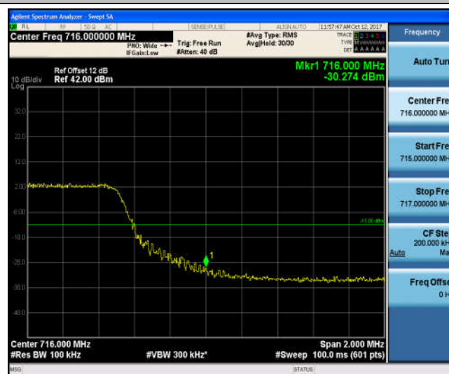
Band17_10MHz_16QAM_23800_50RB#0_-30.27_PASS
