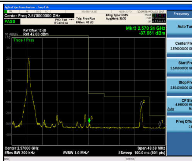
Band7_20MHz_QPSK_21350_100RB#0_-40.26,-27.94,-25.02_PASS
