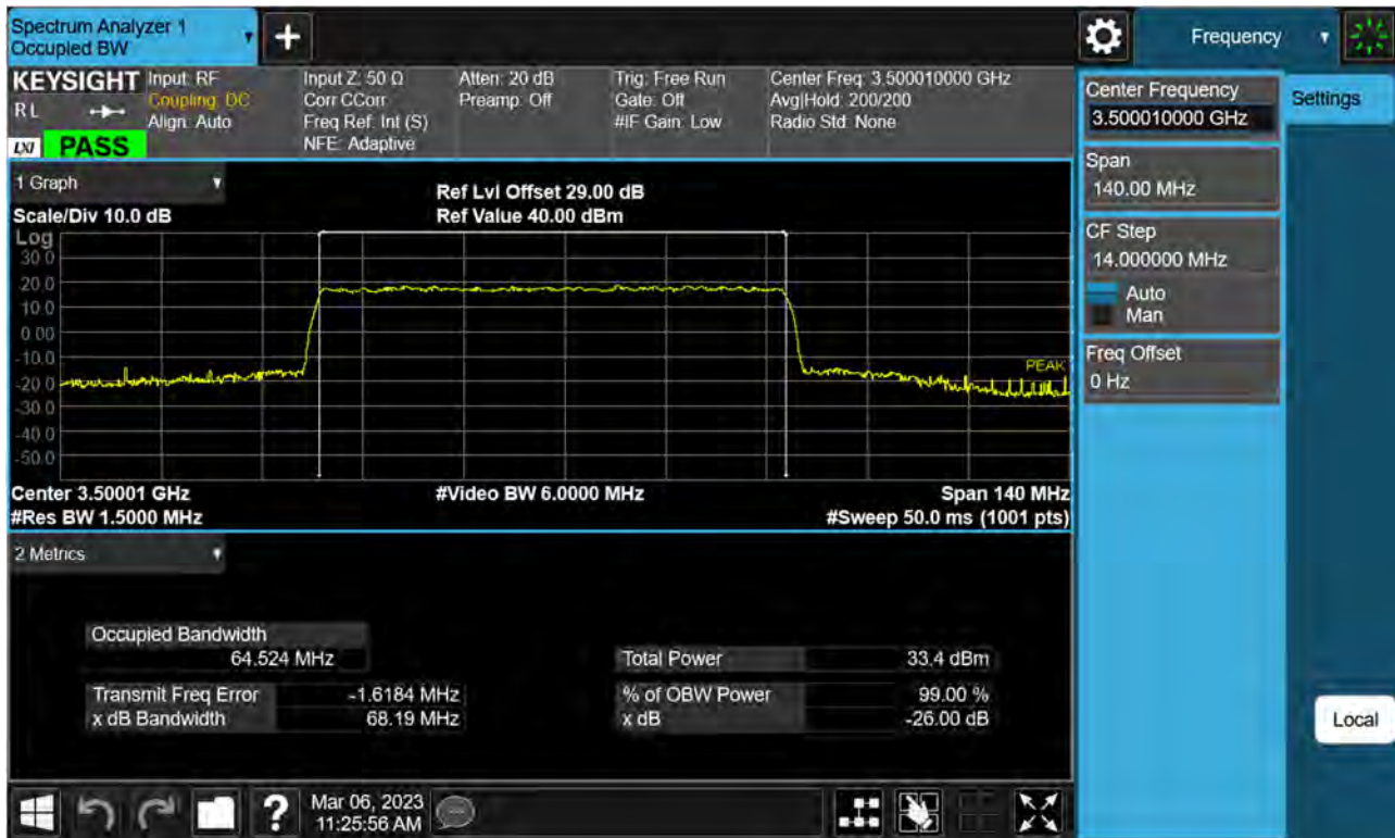
Sub6 n77(78). Occupied Bandwidth Plot (70 M BW Ch.633334 QPSK)
