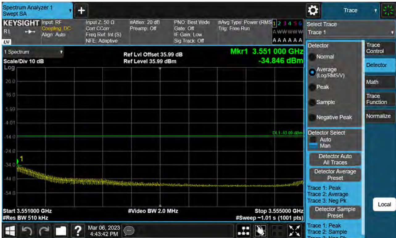
Sub6 n77(78). High Band Edge Plot (30 M BW Ch.635666 BPSK 1RB)(2)
