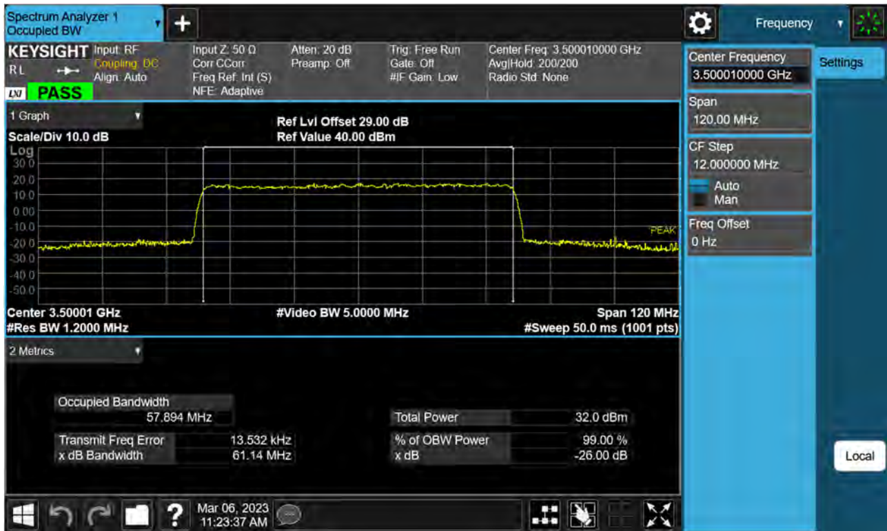
Sub6 n77(78). Occupied Bandwidth Plot (60 M BW Ch.633334 64QAM )
