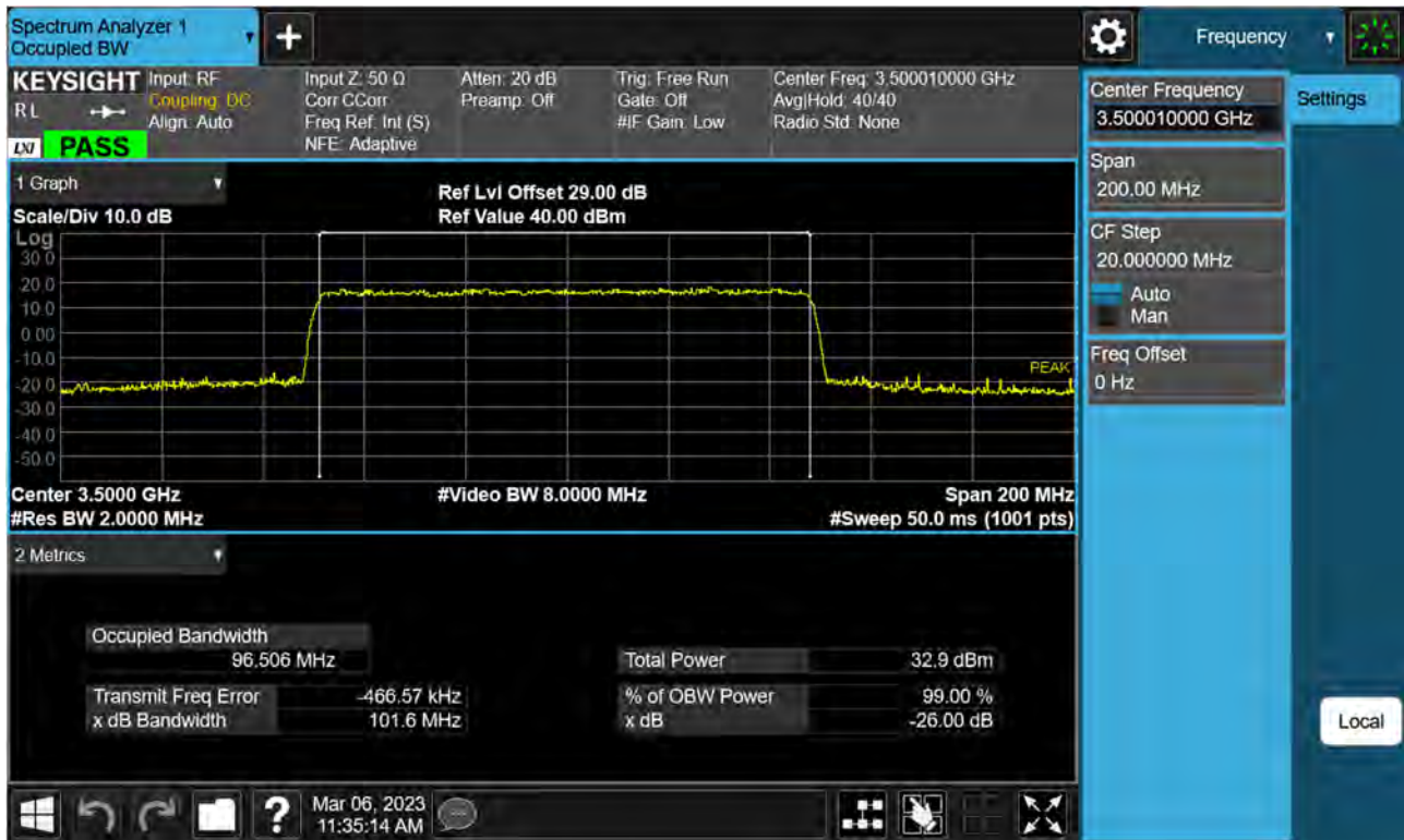
Sub6 n77(78). Occupied Bandwidth Plot (100 M BW Ch.633334 QPSK)
