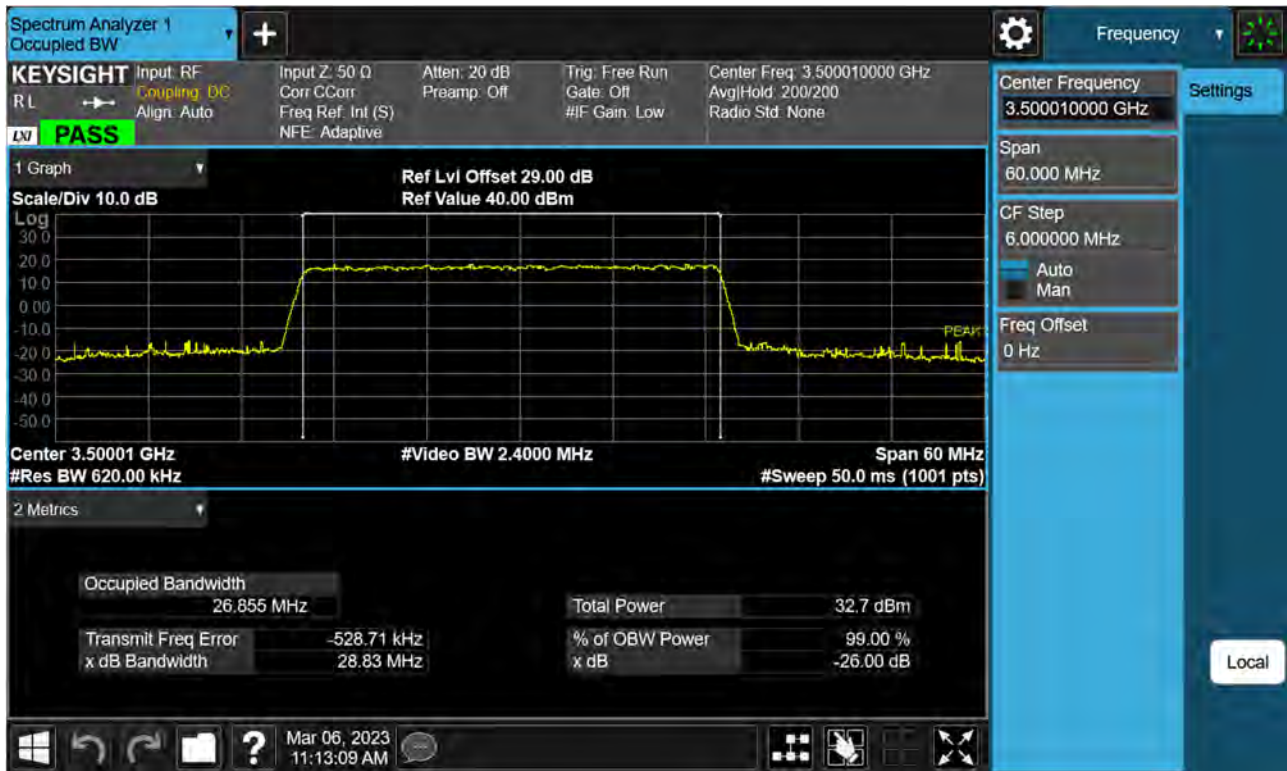
Sub6 n77(78). Occupied Bandwidth Plot (30 M BW Ch.633334 QPSK)
