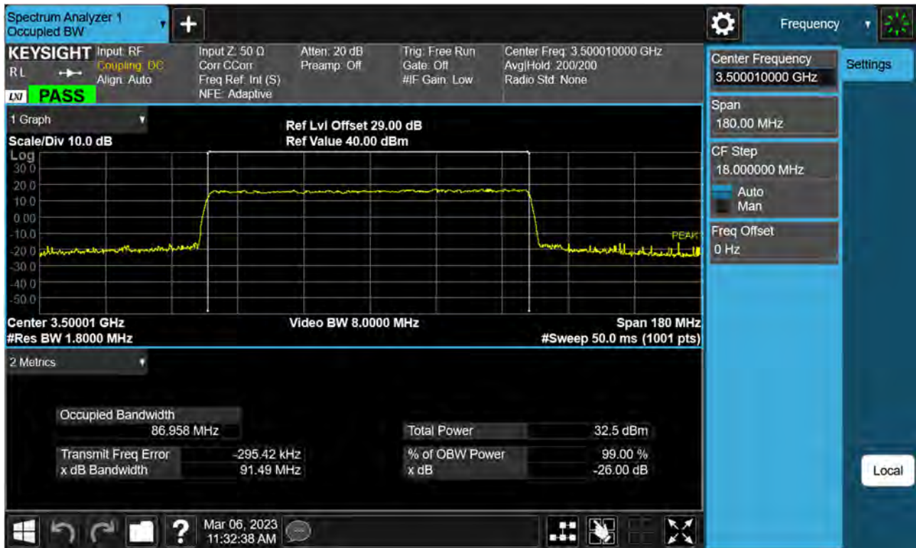
Sub6 n77(78). Occupied Bandwidth Plot (90 M BW Ch.633334 16QAM)
