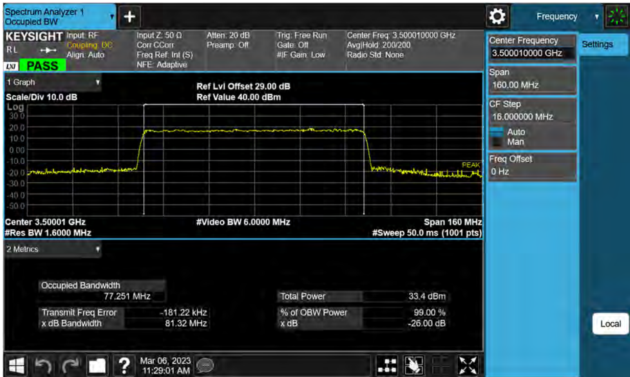
Sub6 n77(78). Occupied Bandwidth Plot (80 M BW Ch.633334 QPSK)
