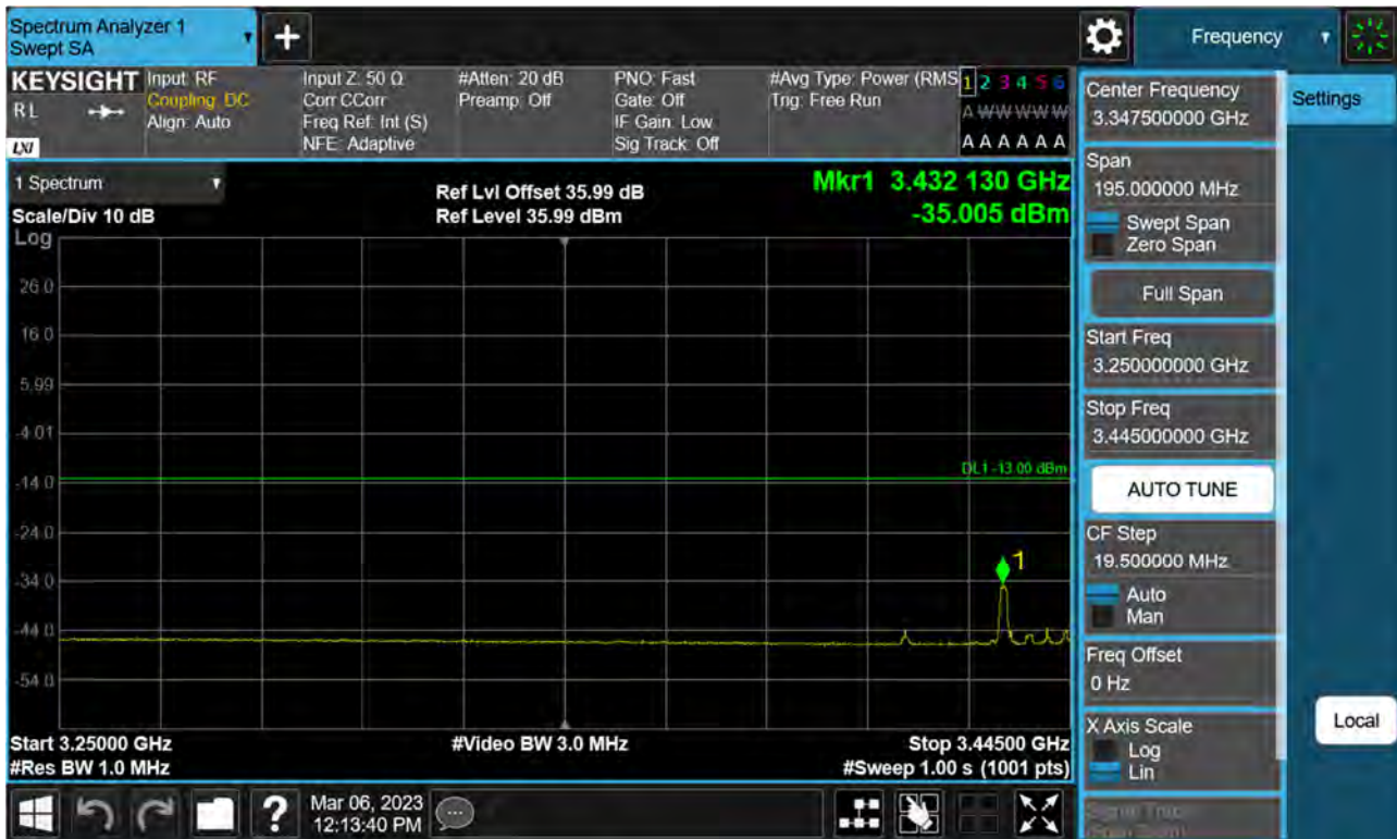
Sub6 n77(78). Low Band Edge Plot (40 M BW Ch.631334 BPSK 1RB)(3)
