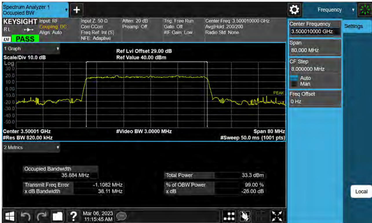
Sub6 n77(78). Occupied Bandwidth Plot (40 M BW Ch.633334 BPSK)
