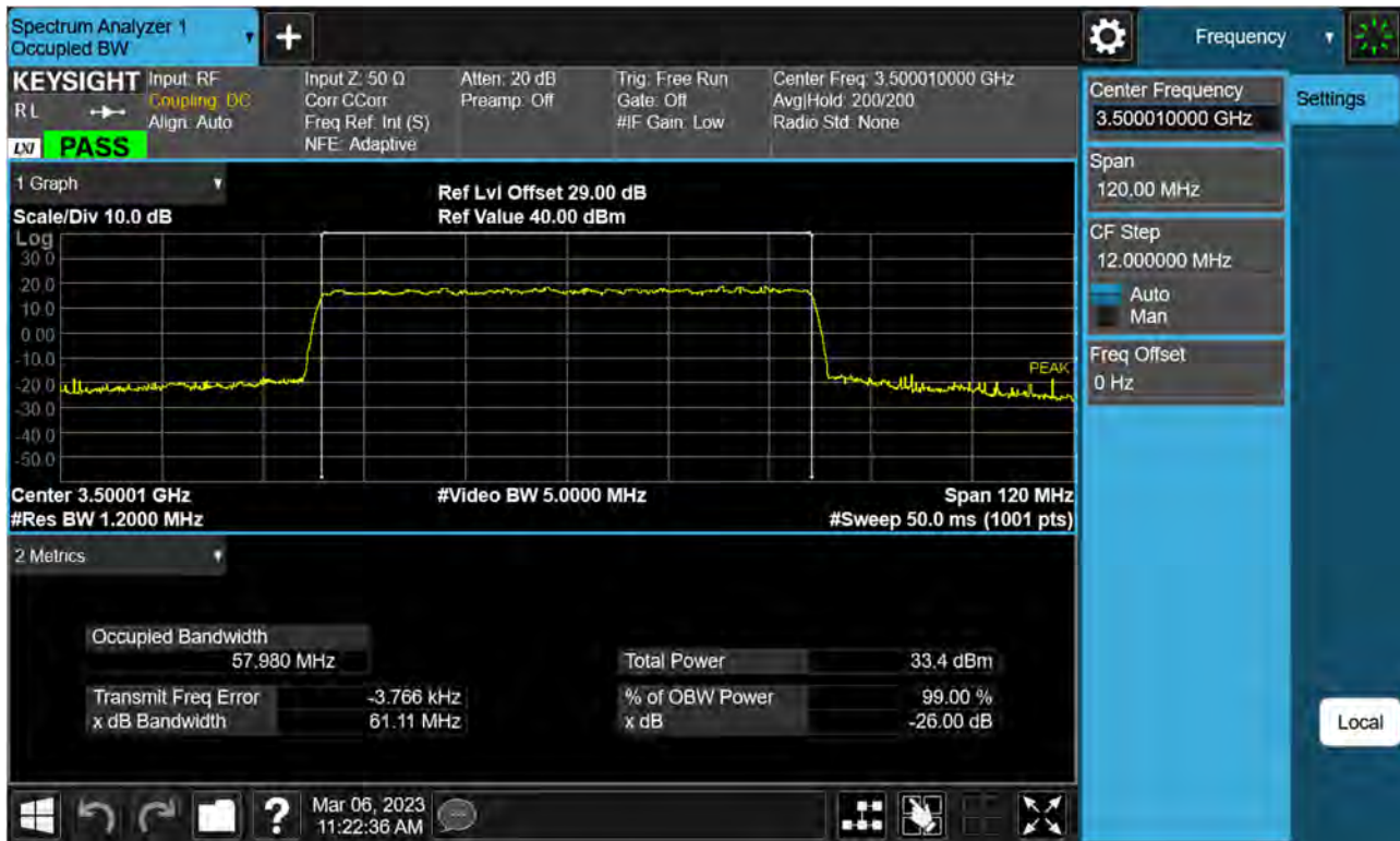
Sub6 n77(78). Occupied Bandwidth Plot (60 M BW Ch.633334 QPSK)
