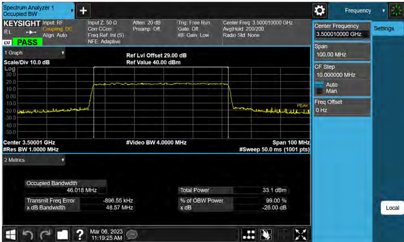
Sub6 n77(78). Occupied Bandwidth Plot (50 M BW Ch.633334 QPSK)
