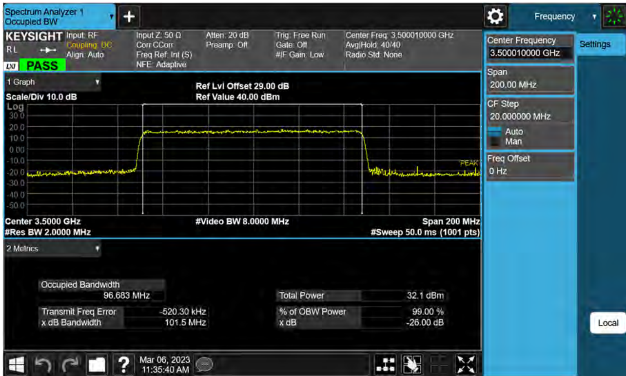
Sub6 n77(78). Occupied Bandwidth Plot (100 M BW Ch.633334 16QAM)
