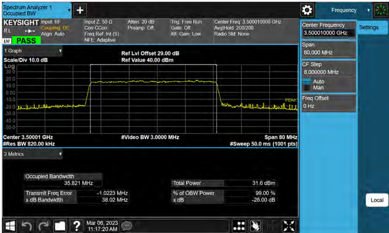
Sub6 n77(78). Occupied Bandwidth Plot (40 M BW Ch.633334 64QAM)
