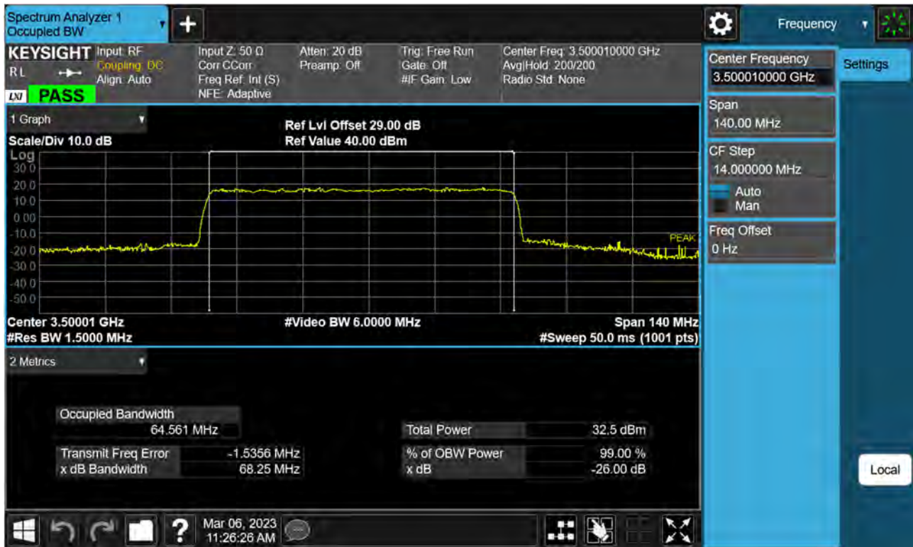
Sub6 n77(78). Occupied Bandwidth Plot (70 M BW Ch.633334 16QAM)
