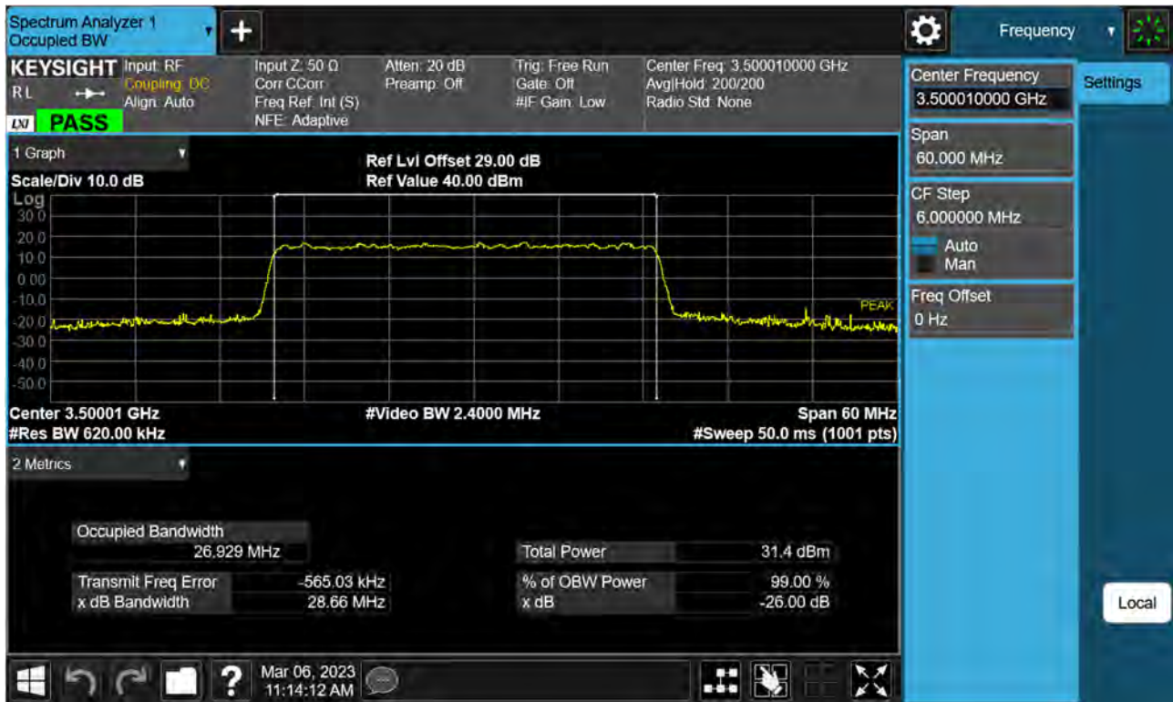
Sub6 n77(78). Occupied Bandwidth Plot (30 M BW Ch.633334 64QAM)
