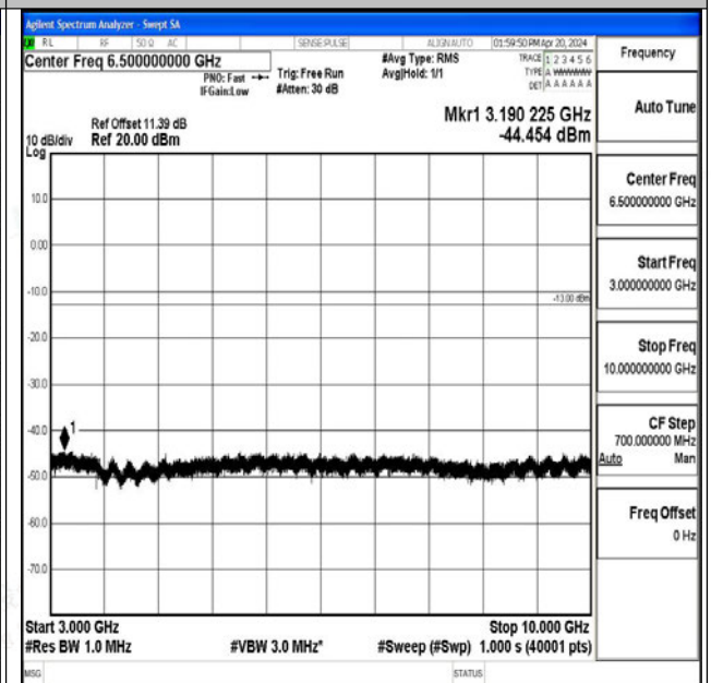
Band26_3MHz_16QAM_26775_1RB#0_3000~10000_30
