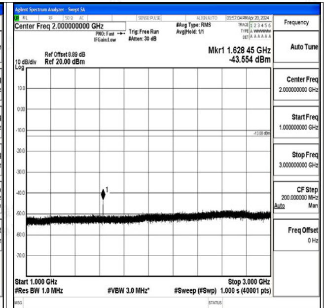
Band26_3MHz_QPSK_26705_1RB#0_1000~3000_1000
