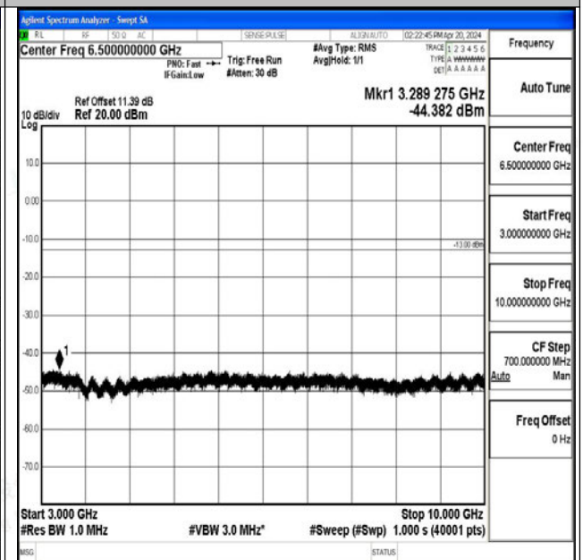
Band26_5MHz_16QAM_26740_1RB#0_3000~10000_30
