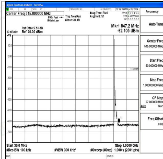
Band26_10MHz_QPSK_26740_1RB#0_30~1000_30~1000
