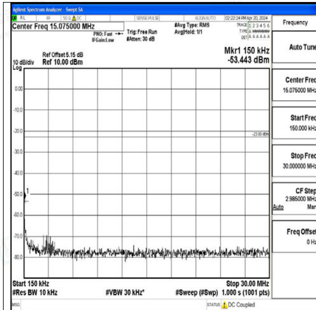
Band26_5MHz_16QAM_26740_1RB#0_0.15~30_0.15~3
