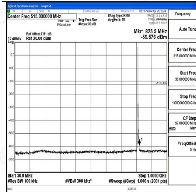
Band26_3MHz_QPSK_26705_1RB#0_30~1000_30~100
