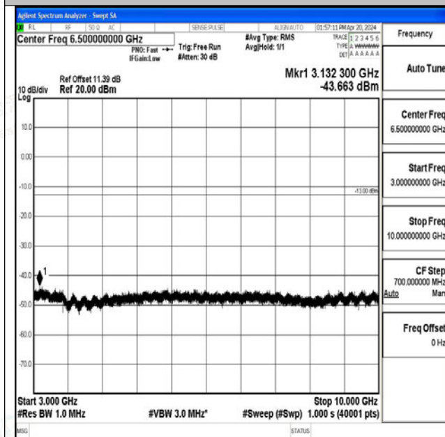
Band26_3MHz_QPSK_26705_1RB#0_3000~10000_300
