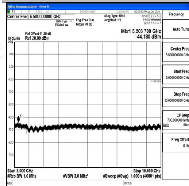
Band26_10MHz_QPSK_26740_1RB#0_3000~10000_3000~10000
