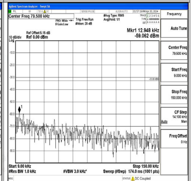
Band26_3MHz_16QAM_26705_1RB#0_0.009~0.15_0.0
