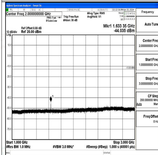
Band26_5MHz_16QAM_26740_1RB#0_1000~3000_100
