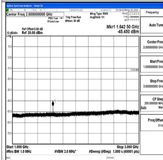
Band26_3MHz_16QAM_26775_1RB#0_1000~3000_100
