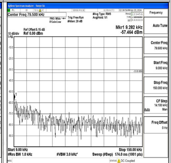
Band26_10MHz_16QAM_26740_1RB#0_0.009~0.15_0.009~0.15
