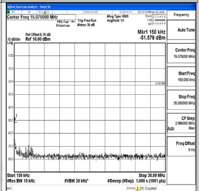
Band26_5MHz_QPSK_26740_1RB#0_0.15~30_0.15~30
