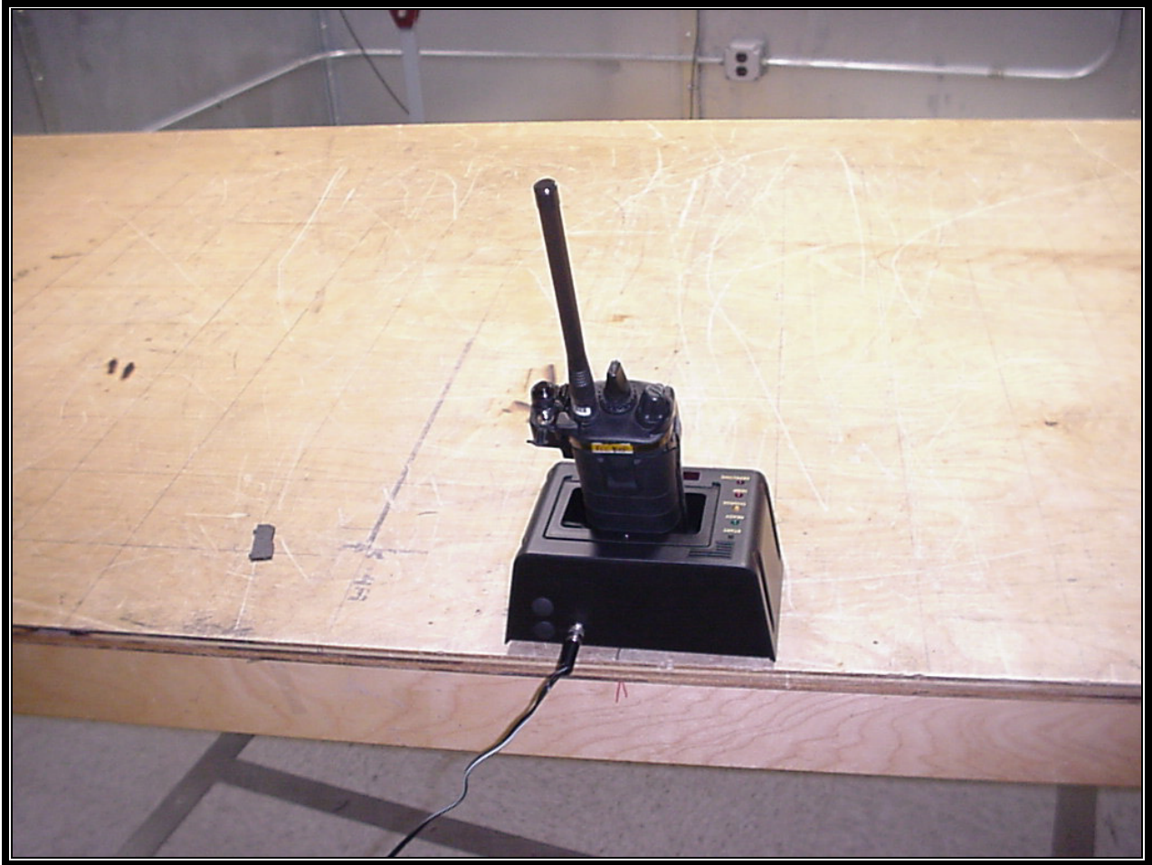
PHOTOGRAPH 6: CONDUCTED EMISSIONS BACK VIEW
