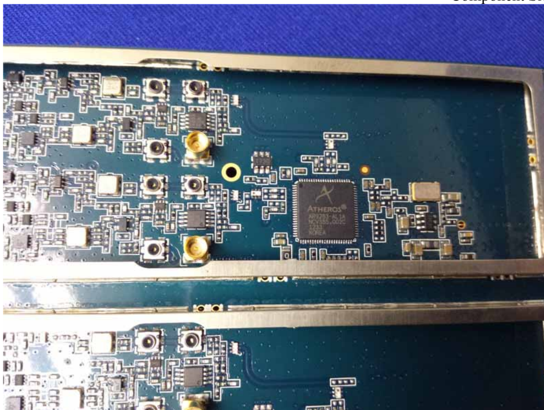
Figure 35 Component Side of the PCB
