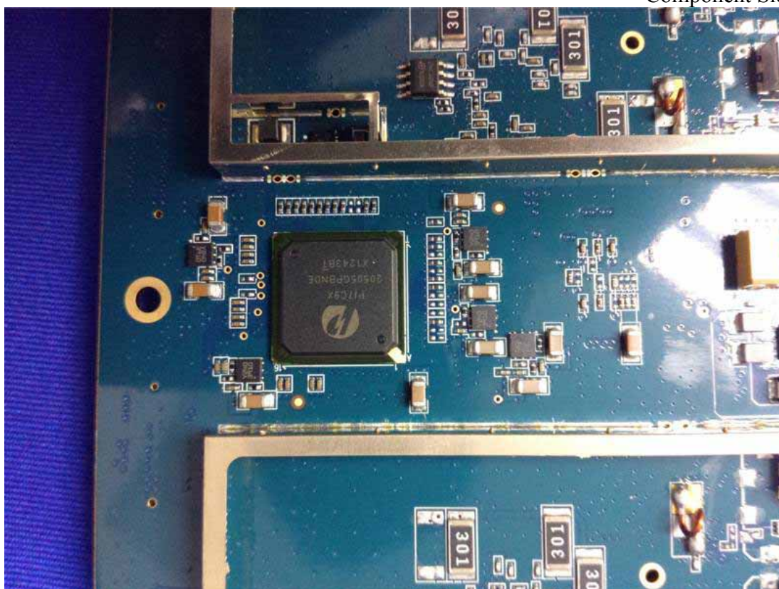
Figure 33 Component Side of the PCB
