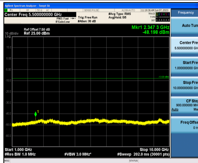
Band13-5MHz-QPSK-23255-1-0-Low-1000-10000--48.2-PASS
