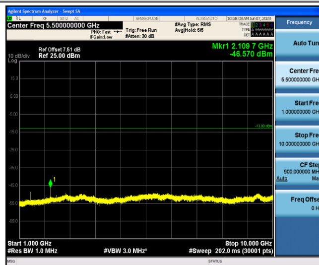
Band12-10MHz-QPSK-23095-1-0-Low-1000-10000--46.57-PASS
