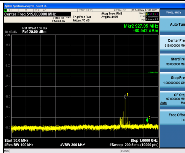
Band13-5MHz-16QAM-23205-1-0-Low-30-1000--60.54-PASS
