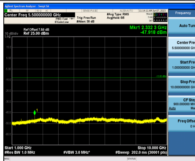
Band13-5MHz-16QAM-23205-1-0-Low-1000-10000--47.92-PASS
