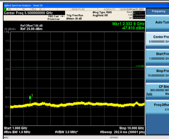
Band13-10MHz-16QAM-23230-1-0-Low-1000-10000--47.81-PASS
