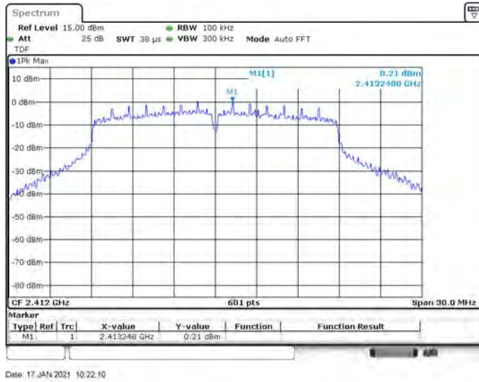
802.11n-20 MHz LOW CHANNEL, Carrier level
