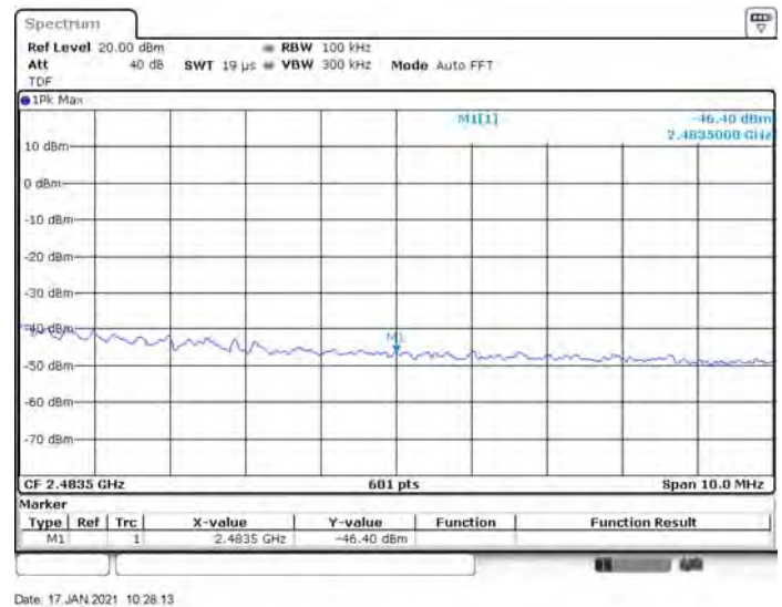
802.11n-20 MHz HIGH CHANNEL, Reference level
