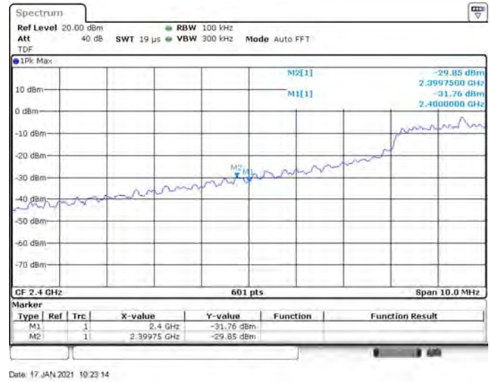
802.11n-20 MHz LOW CHANNEL, Reference level
