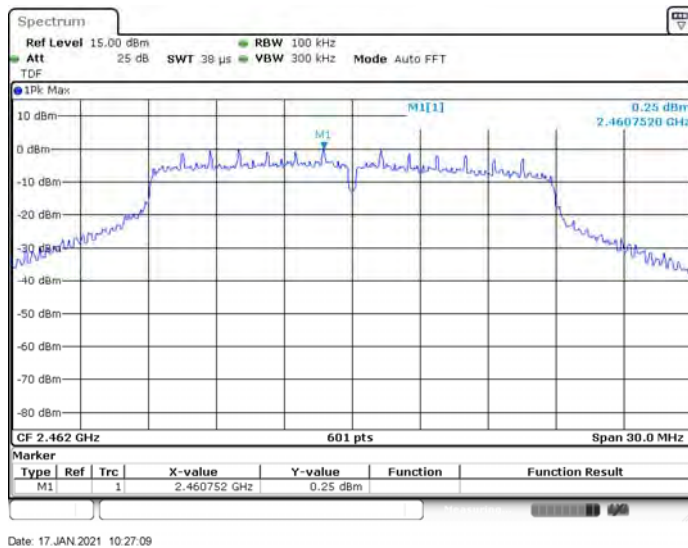
802.11n-20 MHz HIGH CHANNEL, Carrier level
