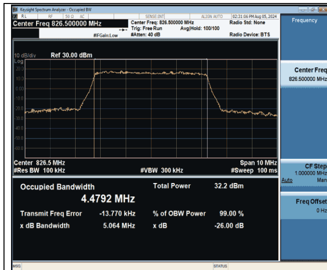
Band5-5MHz-QPSK-20425-25RB#0-PASS
