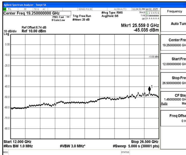
Band26-3MHz-16QAM-26705-1-0-Low-12000-26500--45.04-PASS
