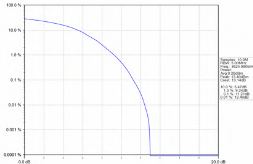
n78d_30kHz_SISO_NTNV_70MHz_DFT-s-OFDM_16_QAM_3624.99MHz_Outer_Full
