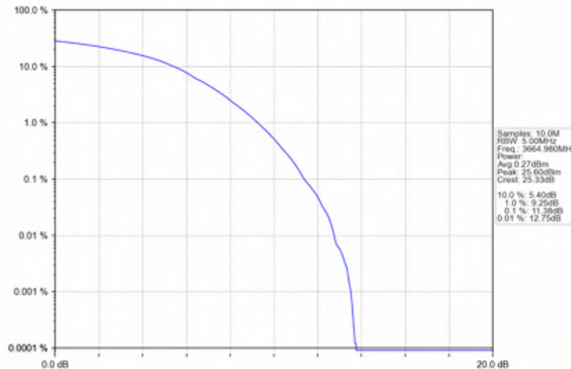
n78d_30kHz_SISO_NTNV_70MHz_DFT-s-OFDM_256_QAM_3664.98MHz_Outer_Full
