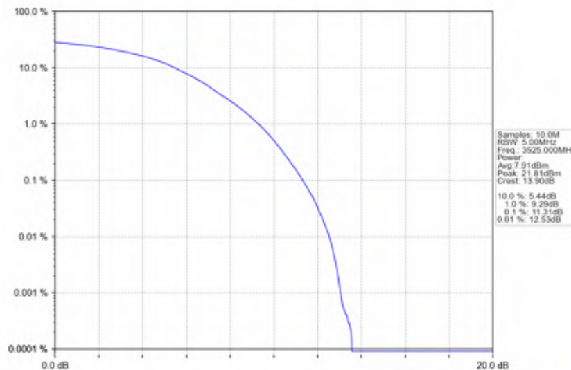
n78e_15kHz_SISO_NTNV_50MHz_DFT-s-OFDM QPSK_3525MHz_Outer_Full
