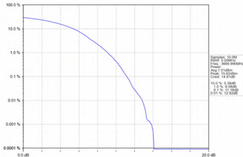
n78d_30kHz_SISO_NTNV_60MHz_DFT-s-OFDM_256_QAM_3669.99MHz_Outer_Full
