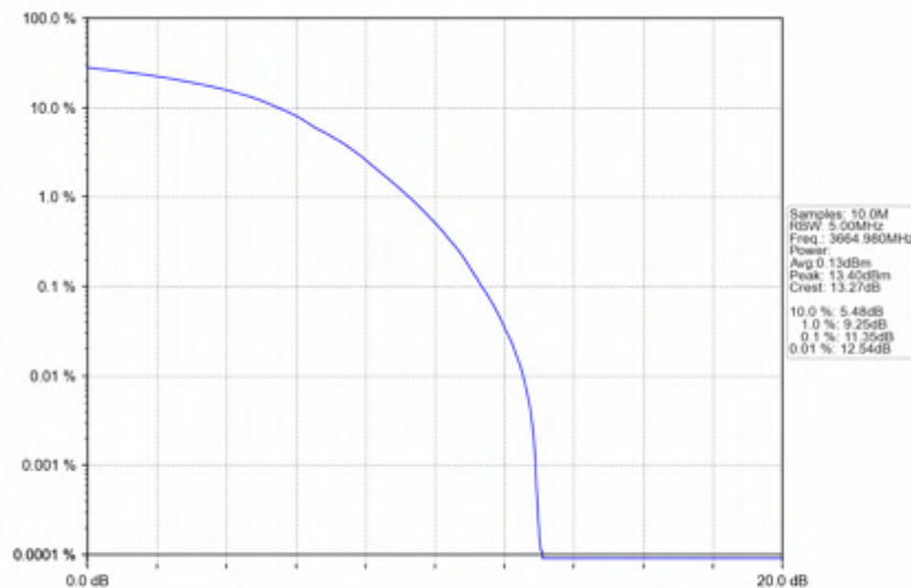
n78d_30kHz_SISO_NTV_70MHz_DFT-s-OFDM 16 QAM_3664.98MHz_Outer_Full
