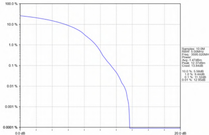
n78d_30kHz_SISO_NTNV_90MHz_DFT-s-OFDM_256_QAM_3595.02MHz_Outer_Full
