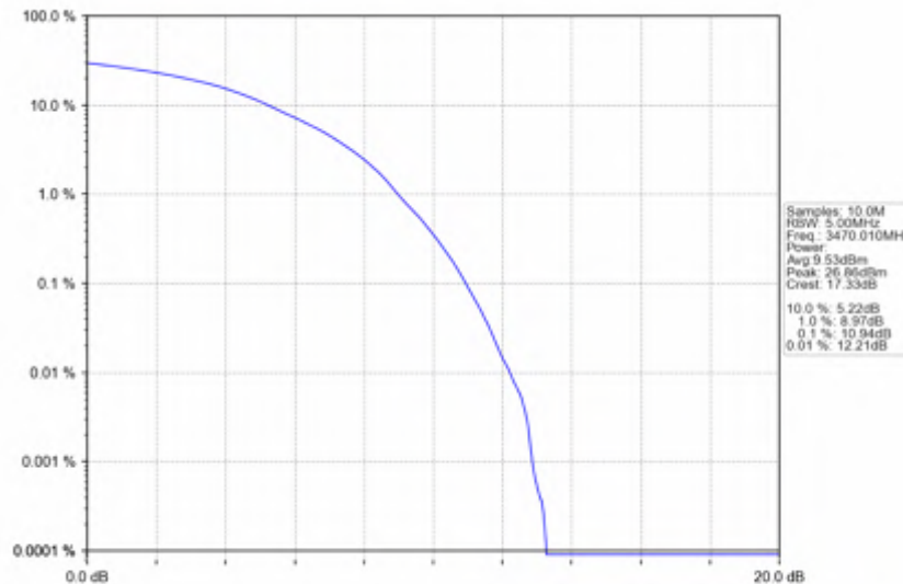
n78e_15kHz_SISO_NTNV_40MHz_DFT-s-OFDM 64 QAM_3470.01MHz_Outer_Full
