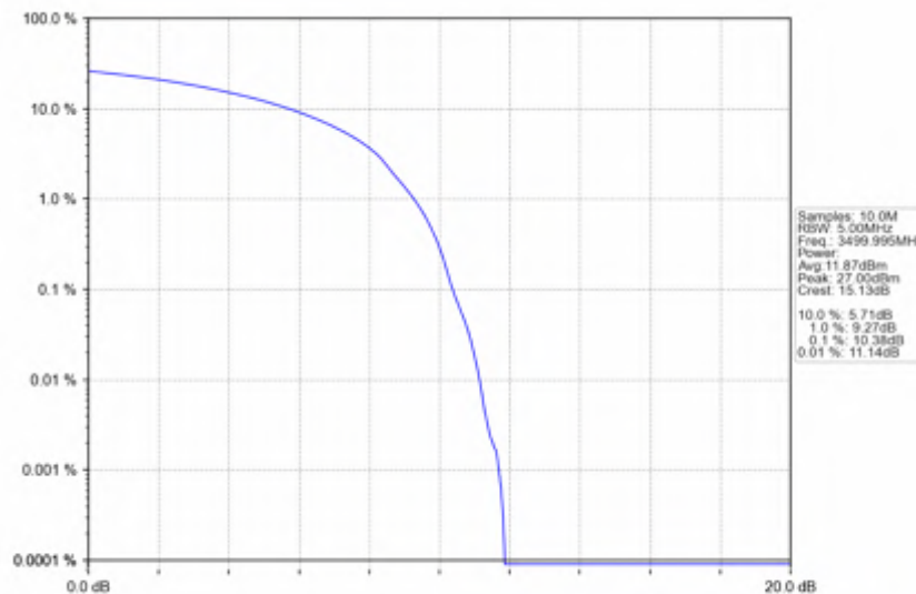
n78e_15kHz_SISO_NTNV_20MHz_DFT-s-OFDM QPSK_3499.995MHz_Outer_Full
