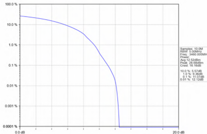
n78e_15kHz_SISO_NTNV_20MHz_DFT-s-OFDM 64 QAM_3460.005MHz_Outer_Full
