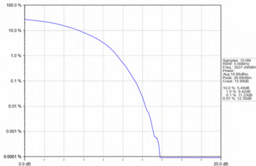
n78e_15kHz_SISO_NTNV_25MHz_DFT-s-OFDM_16_QAM_3537.495MHz_Outer_Full
