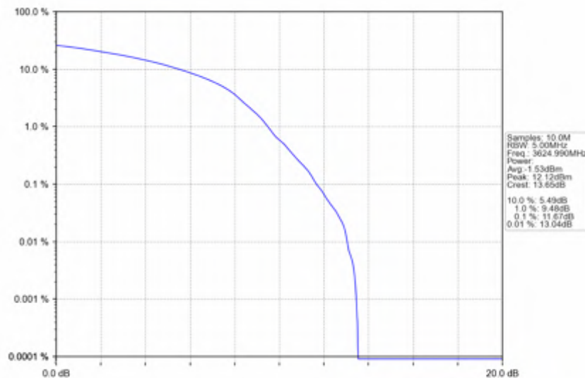
n78d_30kHz_SISO_NTNV_100MHz_DFT-s-OFDM_16_QAM_3624.99MHz_Outer_Full
