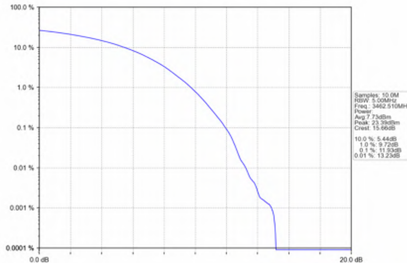
n78e_15kHz_SISO_NTNV_25MHz_CP-OFDM_256_QAM_3462.51MHz_Outer_Full
