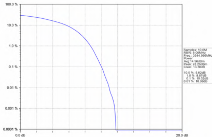
n78e_15kHz_SISO_NTNV_10MHz_DFT-s-OFDM 16 QAM_3544.995MHz_Outer_Full
