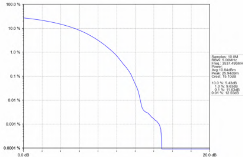
n78e_15kHz_SISO_NTNV_25MHz_CP-OFDM_16_QAM_3537.495MHz_Outer_Full
