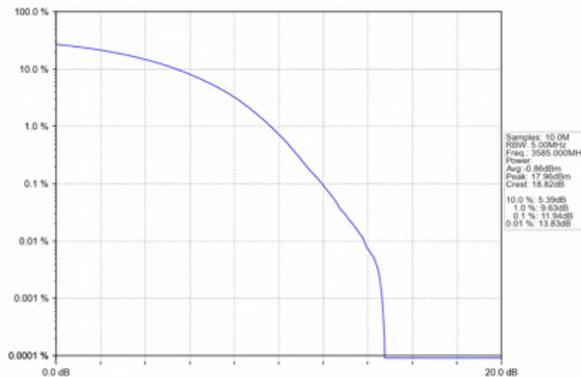
n78d_30kHz_SISO_NTNV_70MHz_CP-OFDM 64 QAM_3585MHz_Outer_Full
