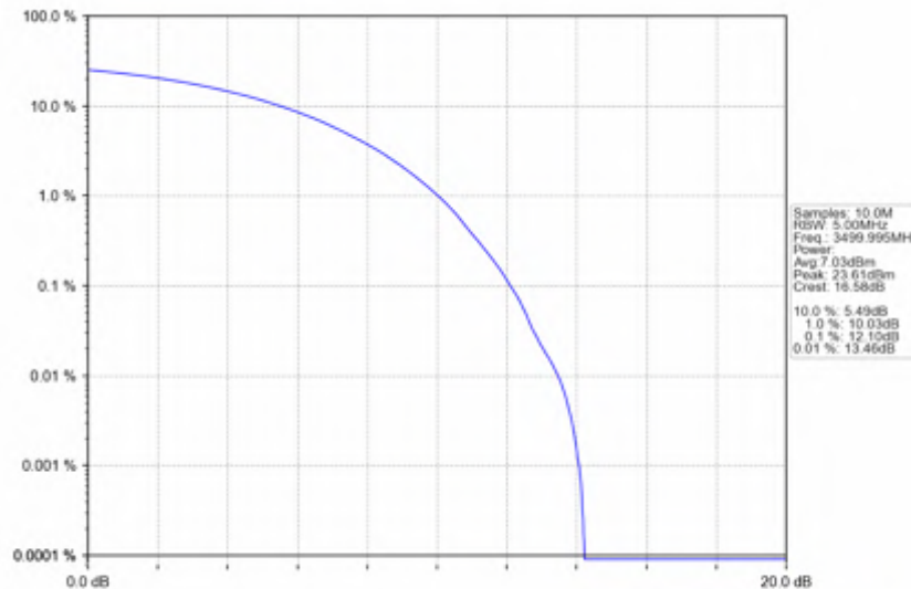
n78e_15kHz_SISO_NTNV_50MHz_CP-OFDM 64 QAM_3499.995MHz_Outer_Full
