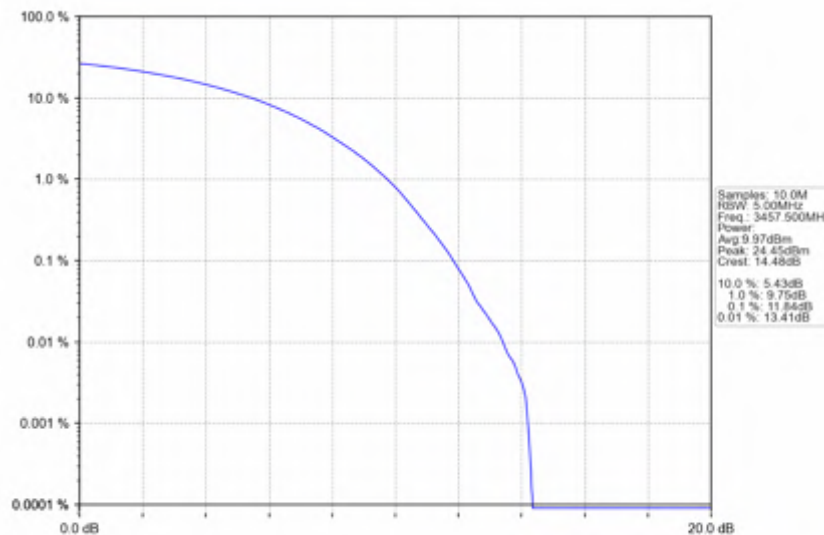
n78e_15kHz_SISO_NTNV_15MHz_CP-OFDM_256_QAM_3457.5MHz_Outer_Full
