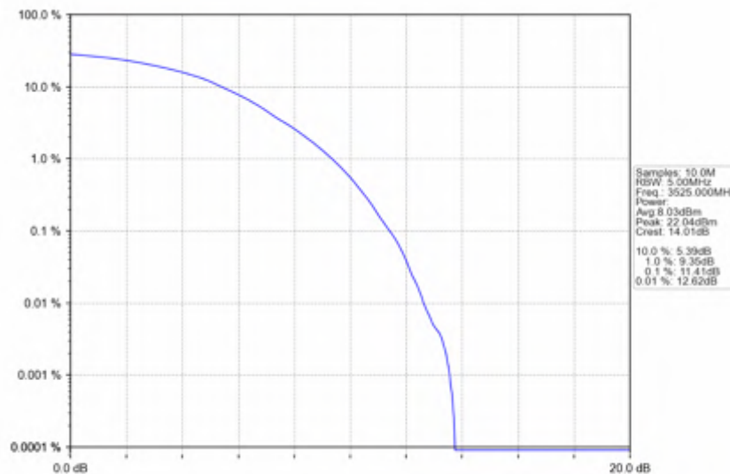
n78e_15kHz_SISO_NTNV_50MHz_DFT-s-OFDM 64 QAM_3525MHz_Outer_Full
