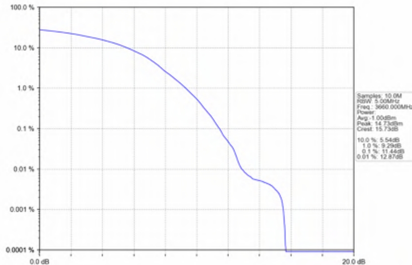
n78d_30kHz_SISO_NTNV_80MHz_DFT-s-OFDM_256_QAM_3660MHz_Outer_Full
