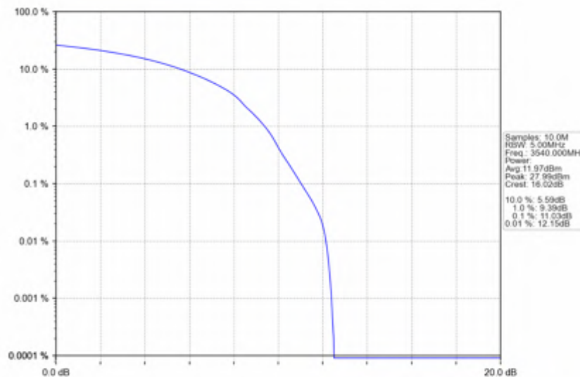
n78e_15kHz_SISO_NTNV_20MHz_DFT-s-OFDM 64 QAM_3540MHz_Outer_Full
