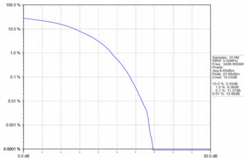
n78e_15kHz_SISO_NTNV_40MHz_DFT-s-OFDM_64_QAM_3499.995MHz_Outer_Full
