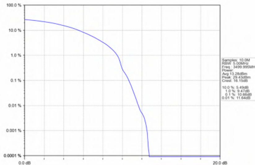
n78e_15kHz_SISO_NTNV_15MHz_DFT-s-OFDM_64_QAM_3499.995MHz_Outer_Full
