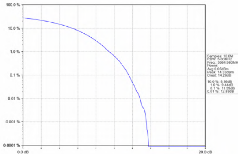
n78d_30kHz_SISO_NTNV_70MHz_CP-OFDM QPSK_3664.98MHz_Outer_Full
