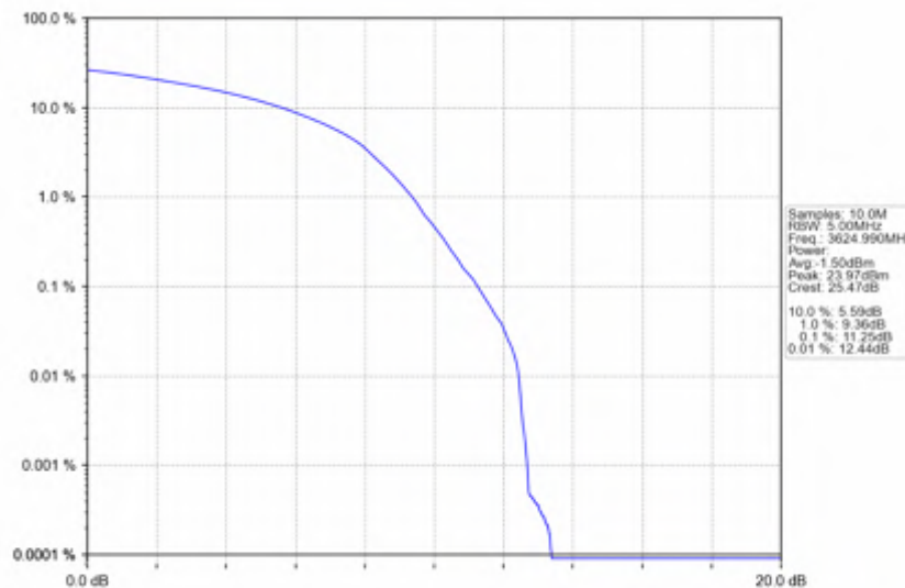
n78d_30kHz_SISO_NTNV_100MHz_DFT-s-OFDM_QPSK_3624.99MHz_Outer_Full
