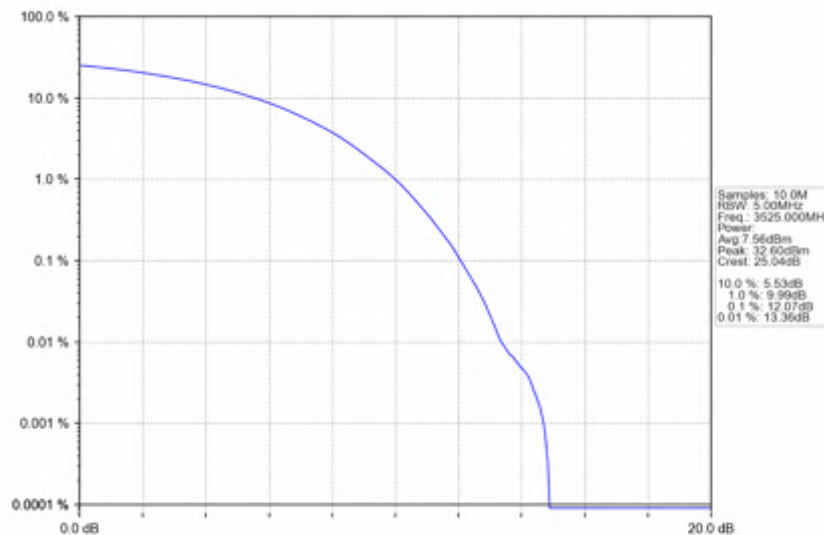
n78e_15kHz_SISO_NTNV_50MHz_CP-OFDM QPSK_3525MHz_Outer_Full
