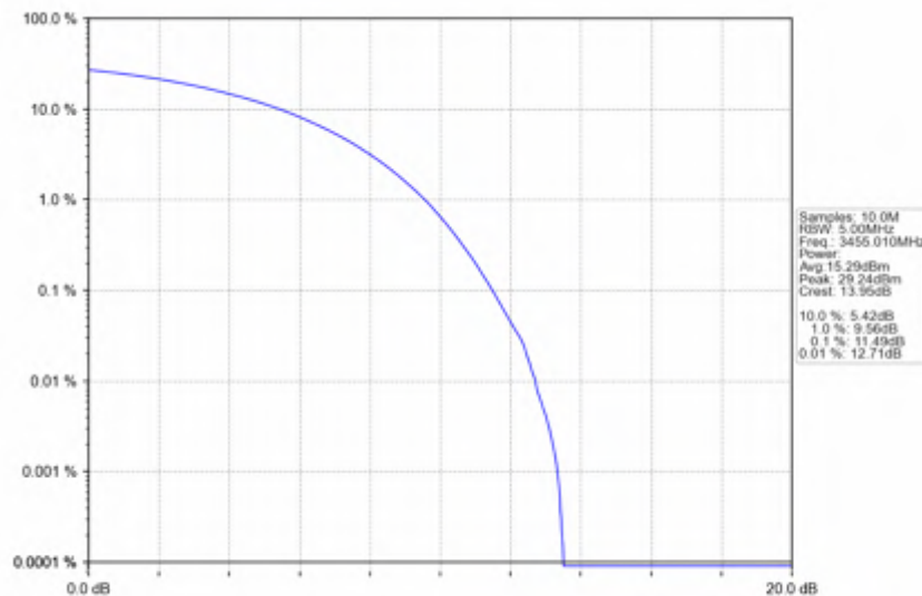
n78e_15kHz_SISO_NTNV_10MHz_CP-OFDM QPSK_3455.01MHz_Outer_Full
