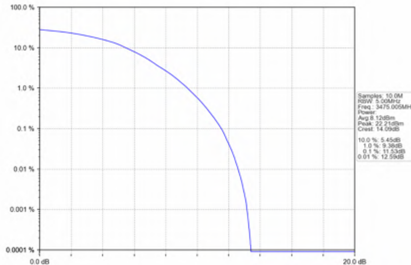
n78e_15kHz_SISO_NTNV_50MHz_DFT-s-OFDM_16_QAM_3475.005MHz_Outer_Full
