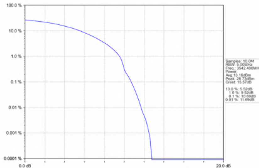
n78e_15kHz_SISO_NTNV_15MHz_DFT-s-OFDM_64_QAM_3542.49MHz_Outer_Full
