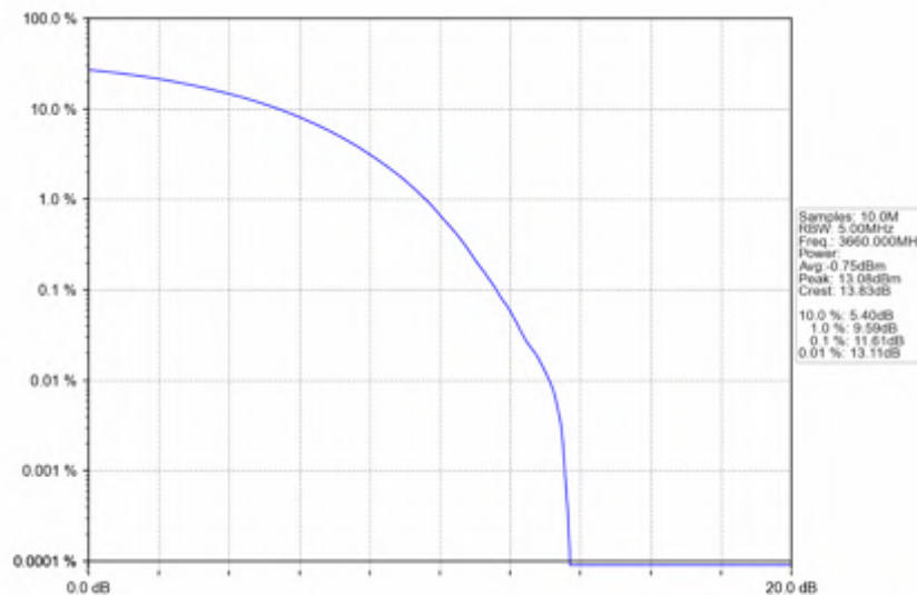
n78d_30kHz_SISO_NTNV_80MHz_CP-OFDM QPSK_3660MHz_Outer_Full
