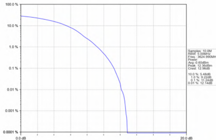
n78d_30kHz_SISO_NTNV_80MHz_DFT-s-OFDM_QPSK_3624.99MHz_Outer_Full
