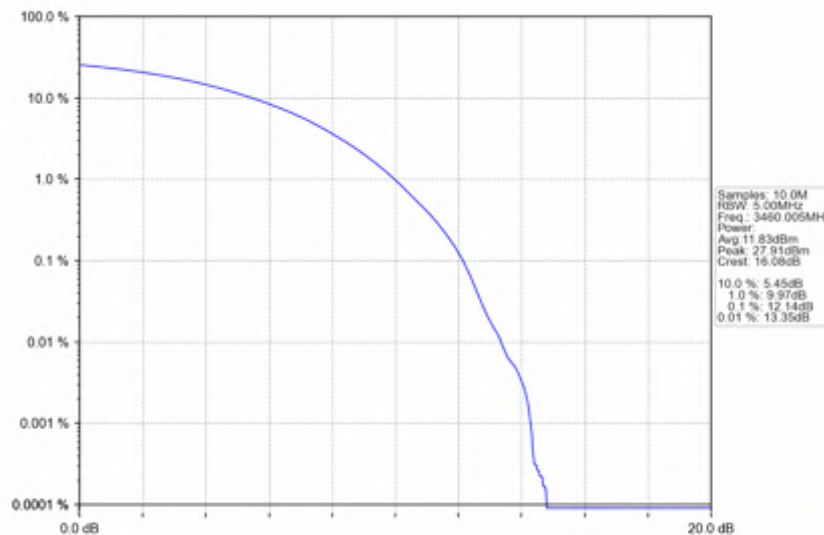
n78e_15kHz_SISO_NTNV_20MHz_CP-OFDM_QPSK_3460.005MHz_Outer_Full
