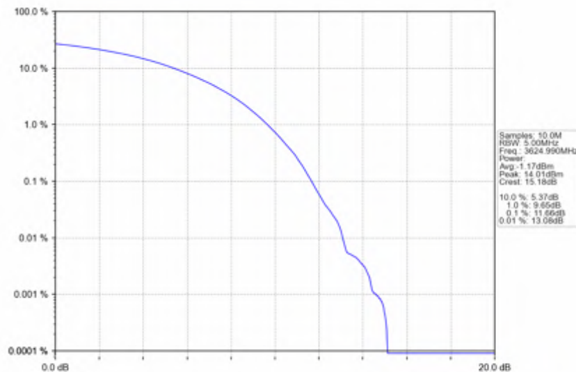
n78d_30kHz_SISO_NTNV_90MHz_CP-OFDM QPSK_3624.99MHz_Outer_Full
