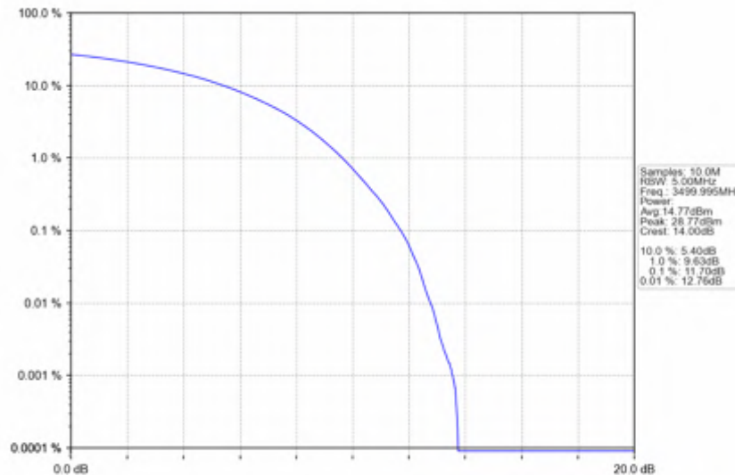
n78e_15kHz_SISO_NTNV_10MHz_CP-OFDM_16_QAM_3499.995MHz_Outer_Full
