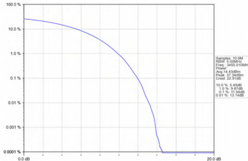
n78e_15kHz_SISO_NTNV_10MHz_CP-OFDM_64_QAM_3455.01MHz_Outer_Full
