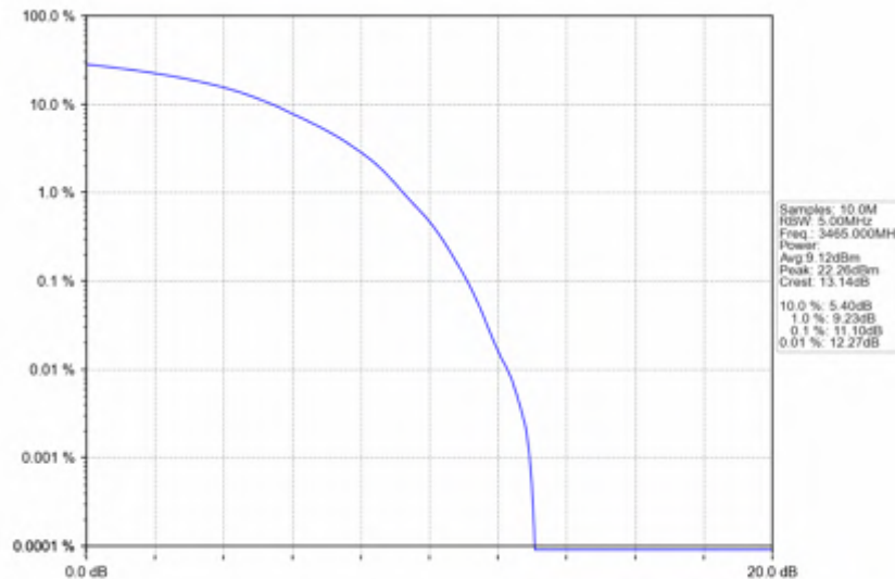
n78e_15kHz_SISO_NTNV_30MHz_DFT-s-OFDM_256_QAM_3465MHz_Outer_Full
