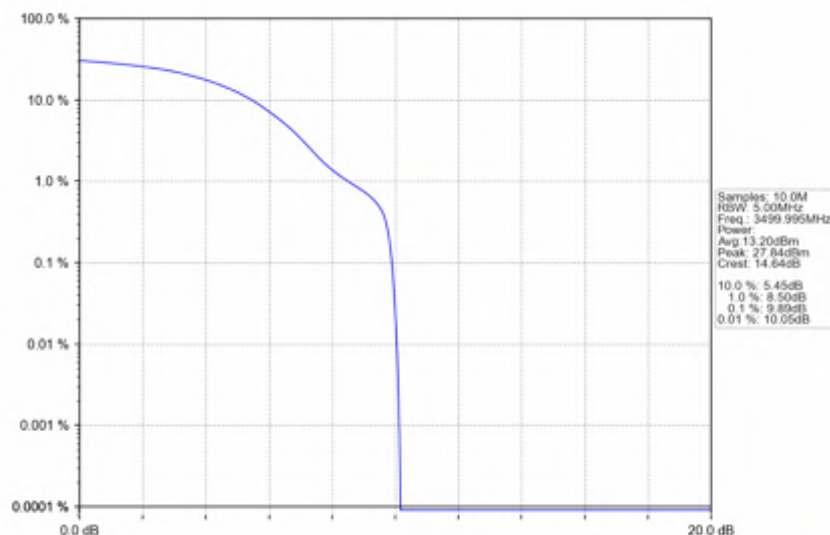
n78e_15kHz_SISO_NTNV_15MHz_DFT-s-OFDM_PI/2_BPSK_3499.995MHz_Outer_Full
