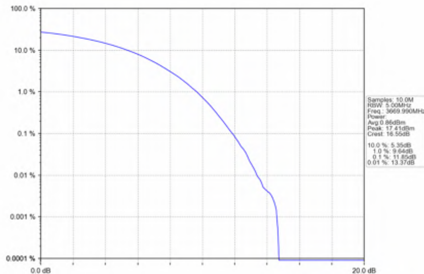
n78d_30kHz_SISO_NTNV_60MHz_CP-OFDM 16 QAM_3669.99MHz_Outer_Full
