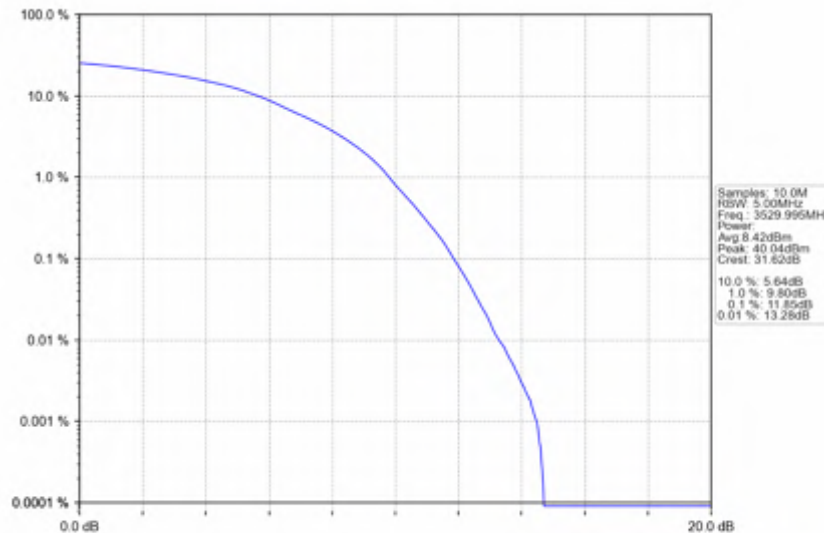
n78e_15kHz_SISO_NTNV_40MHz_DFT-s-OFDM 16 QAM_3529.995MHz_Outer_Full
