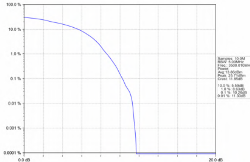
n78e_30kHz_SISO_NTNV_10MHz_DFT-s-OFDM_256_QAM_3500.01MHz_Outer_Full
