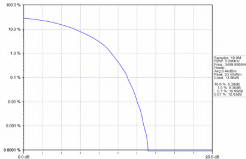
n78e_15kHz_SISO_NTNV_25MHz_DFT-s-OFDM_256_QAM_3499.995MHz_Outer_Full
