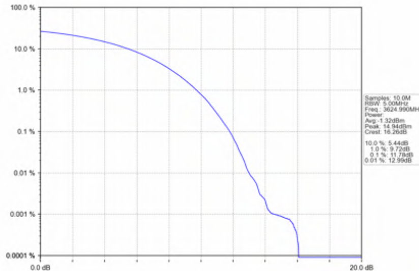
n78d_30kHz_SISO_NTNV_90MHz_CP-OFDM_256_QAM_3624.99MHz_Outer_Full
