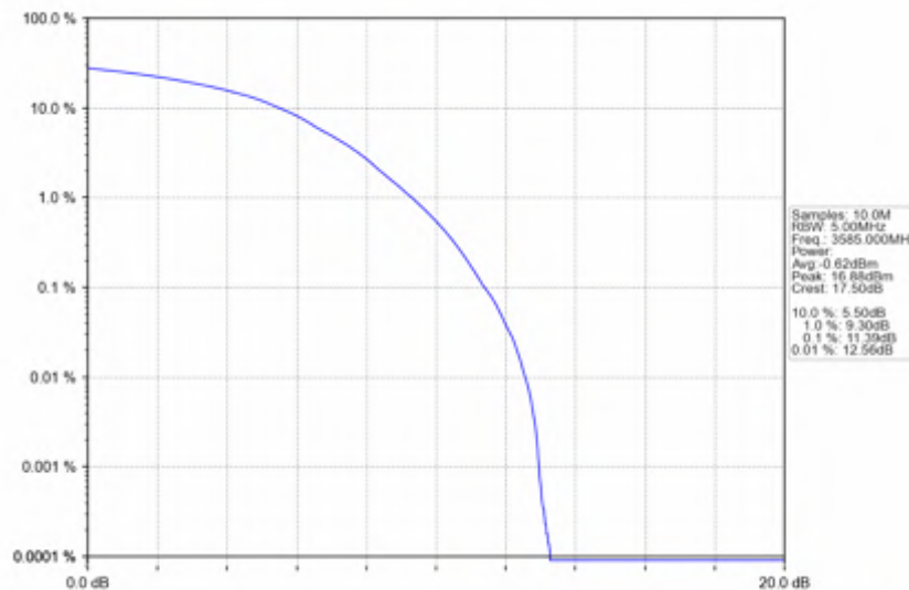
n78d_30kHz_SISO_NTNV_70MHz_DFT-s-OFDM_16_QAM_3585MHz_Outer_Full
