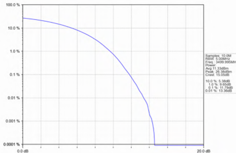
n78e_15kHz_SISO_NTNV_10MHz_CP-OFDM_256_QAM_3499.995MHz_Outer_Full
