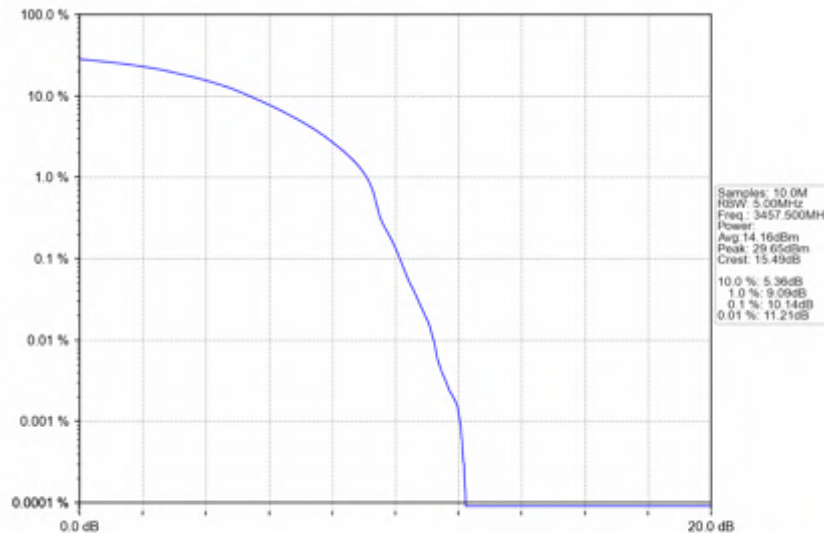
n78e_15kHz_SISO_NTNV_15MHz_DFT-s-OFDM_16_QAM_3457.5MHz_Outer_Full
