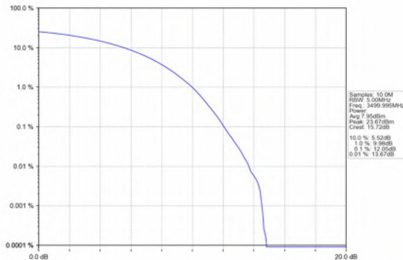
n78e_15kHz_SISO_NTNV_40MHz_CP-OFDM_64_QAM_3499.995MHz_Outer_Full
