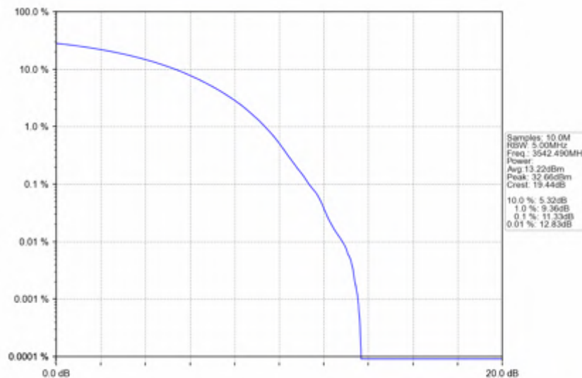
n78e_15kHz_SISO_NTNV_15MHz_CP-OFDM QPSK_3542.49MHz_Outer_Full
