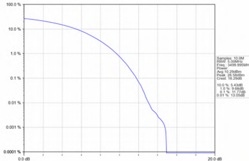
n78e_15kHz_SISO_NTNV_25MHz_CP-OFDM_64_QAM_3499.995MHz_Outer_Full
