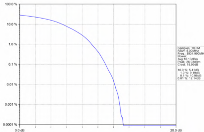
n78e_15kHz_SISO_NTV_30MHz_DFT-s-OFDM 16 QAM_3534.99MHz_Outer_Full
