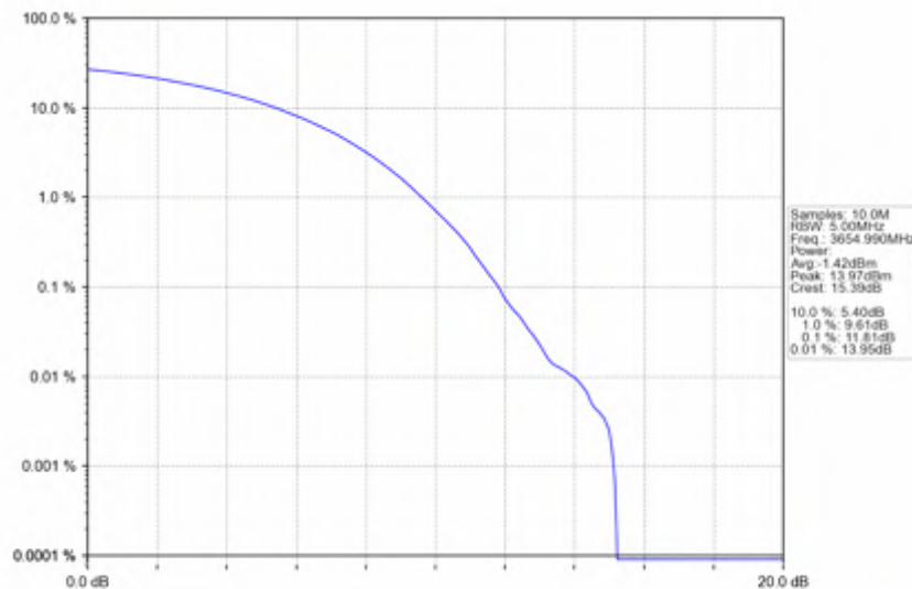
n78d_30kHz_SISO_NTNV_90MHz_CP-OFDM QPSK_3654.99MHz_Outer_Full
