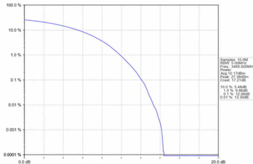
n78e_15kHz_SISO_NTNV_30MHz_CP-OFDM_QPSK_3465MHz_Outer_Full
