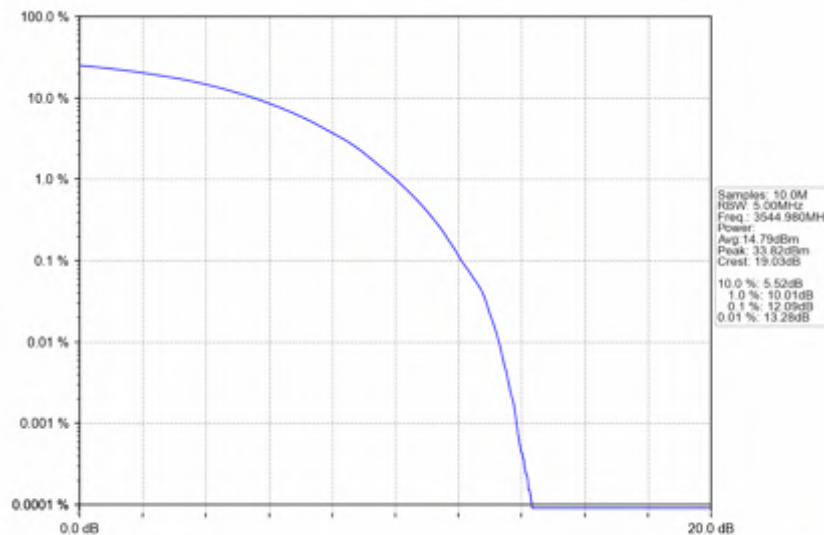
n78e_30kHz_SISO_NTNV_10MHz_CP-OFDM_QPSK_3544.98MHz_Outer_Full
