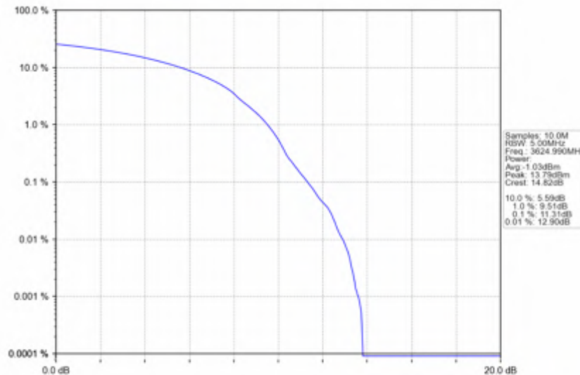
n78d_30kHz_SISO_NTNV_90MHz_DFT-s-OFDM_256_QAM_3624.99MHz_Outer_Full
