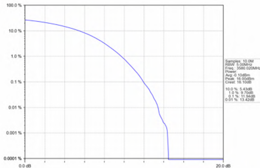
n78d_30kHz_SISO_NTNV_60MHz_CP-OFDM_QPSK_3580.02MHz_Outer_Full
