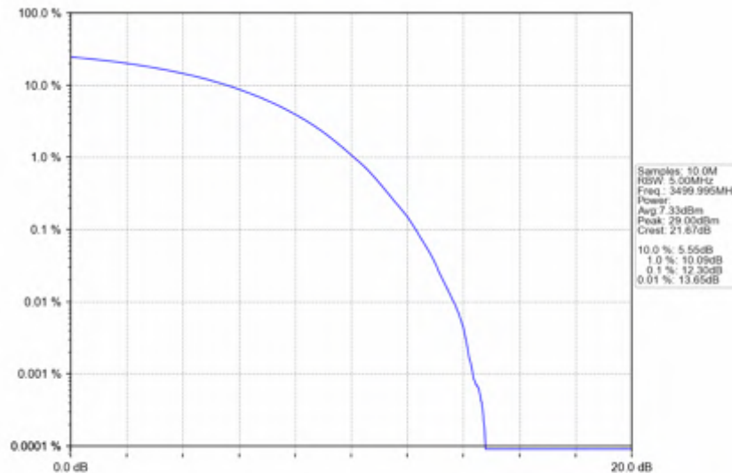
n78e_15kHz_SISO_NTNV_50MHz_CP-OFDM_16_QAM_3499.995MHz_Outer_Full
