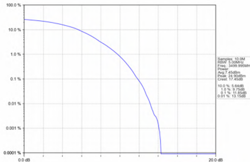
n78e_15kHz_SISO_NTNV_50MHz_DFT-s-OFDM 64 QAM_3499.995MHz_Outer_Full
