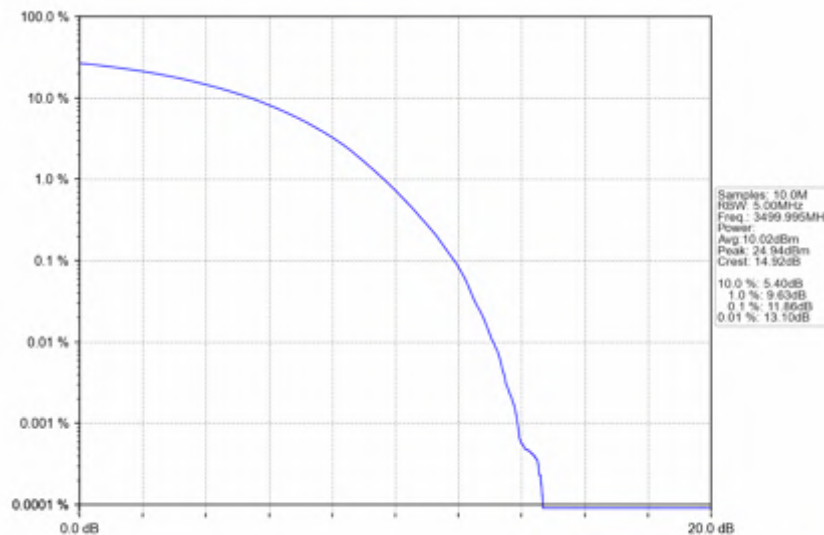
n78e_15kHz_SISO_NTNV_30MHz_CP-OFDM QPSK_3499.995MHz_Outer_Full
