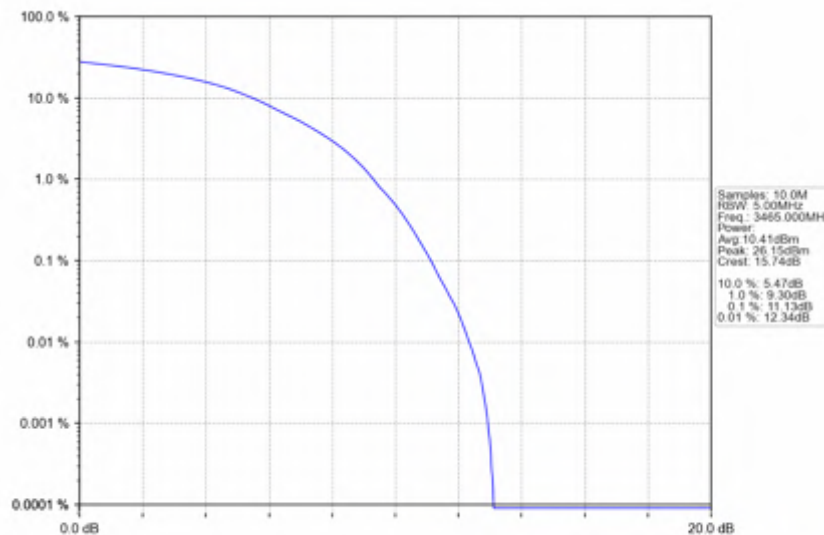
n78e_15kHz_SISO_NTNV_30MHz_DFT-s-OFDM_16_QAM_3465MHz_Outer_Full
