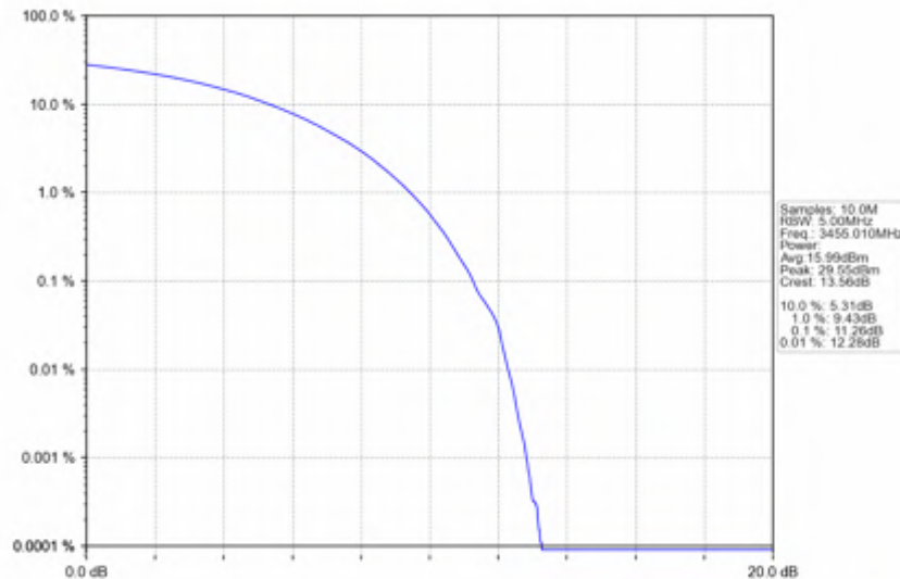
n78e_30kHz_SISO_NTNV_10MHz_CP-OFDM_QPSK_3455.01MHz_Outer_Full
