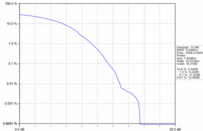
n78d_30kHz_SISO_NTNV_80MHz_DFT-s-OFDM_256_QAM_3590.01MHz_Outer_Full
