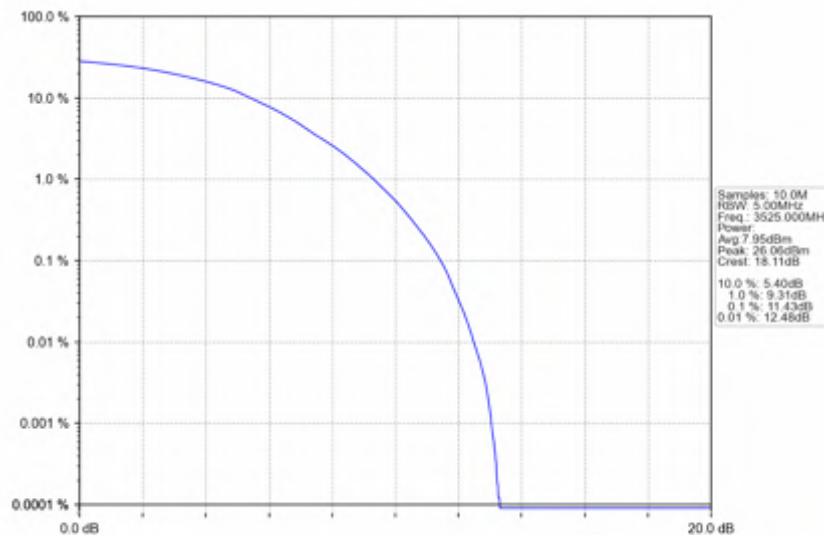
n78e_15kHz_SISO_NTNV_50MHz_DFT-s-OFDM 16 QAM_3525MHz_Outer_Full
