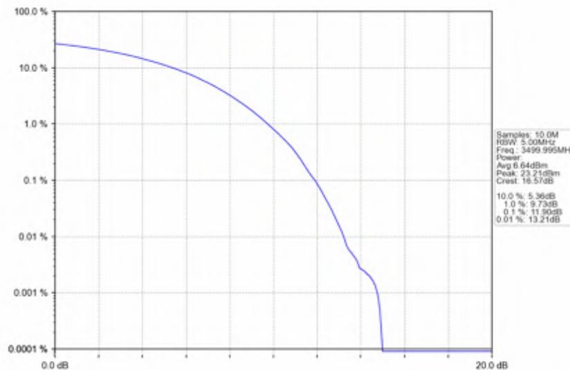
n78e_15kHz_SISO_NTNV_30MHz_CP-OFDM_256_QAM_3499.995MHz_Outer_Full
