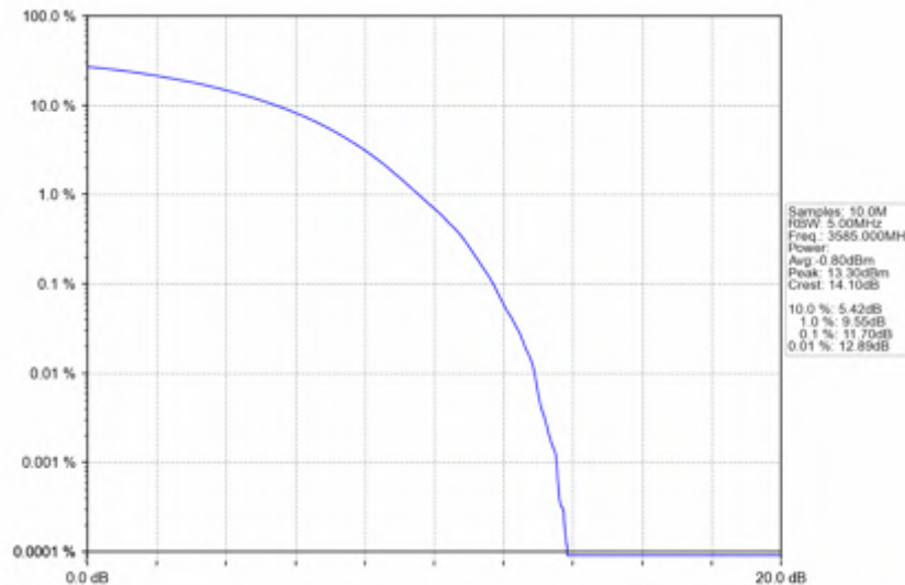
n78d_30kHz_SISO_NTNV_70MHz_CP-OFDM_QPSK_3585MHz_Outer_Full
