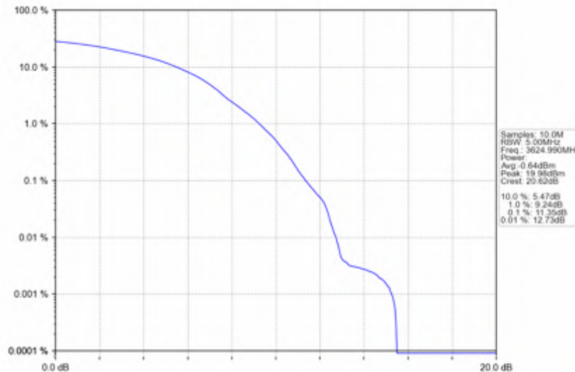
n78d_30kHz_SISO_NTNV_80MHz_DFT-s-OFDM_256_QAM_3624.99MHz_Outer_Full
