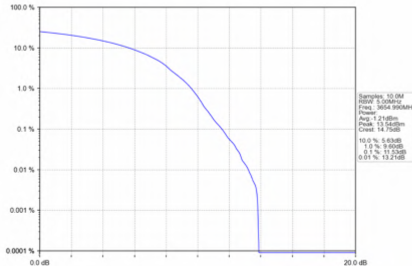
n78d_30kHz_SISO_NTNV_90MHz_DFT-s-OFDM_256_QAM_3654.99MHz_Outer_Full
