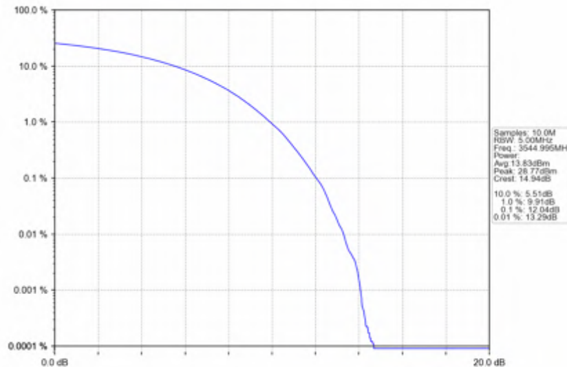
n78e_15kHz_SISO_NTNV_10MHz_CP-OFDM 64 QAM_3544.995MHz_Outer_Full
