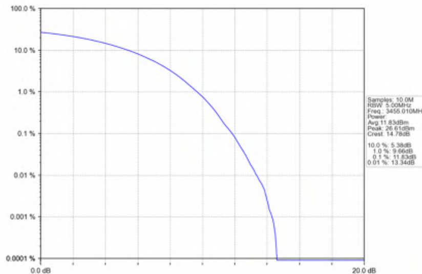
n78e_15kHz_SISO_NTNV_10MHz_CP-OFDM_256_QAM_3455.01MHz_Outer_Full
