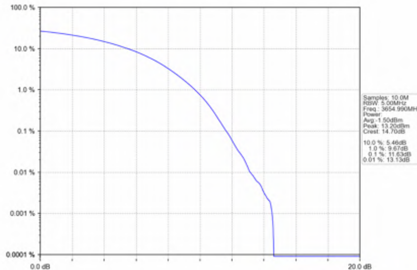
n78d_30kHz_SISO_NTNV_90MHz_CP-OFDM 64 QAM_3654.99MHz_Outer_Full
