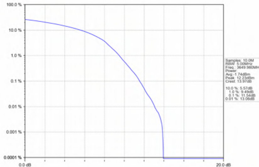
n78d_30kHz_SISO_NTNV_100MHz_DFT-s-OFDM_64_QAM_3649.98MHz_Outer_Full
