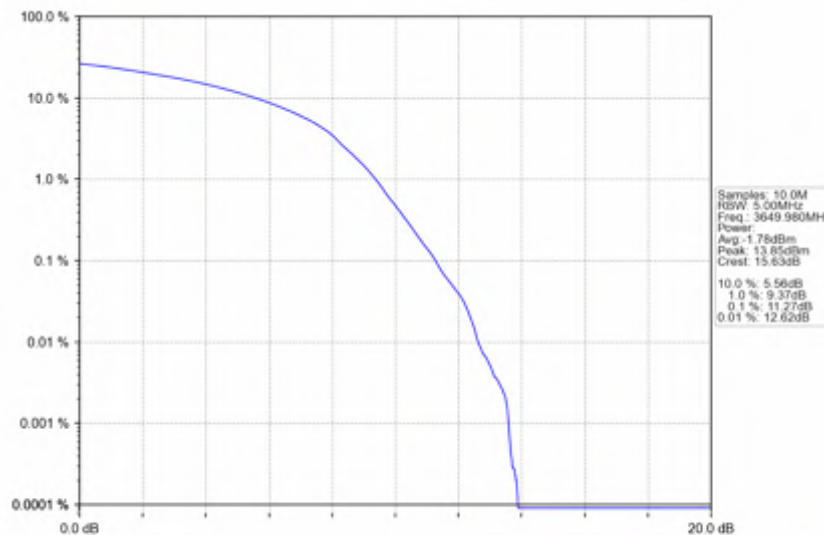
n78d_30kHz_SISO_NTNV_100MHz_DFT-s-OFDM_QPSK_3649.98MHz_Outer_Full
