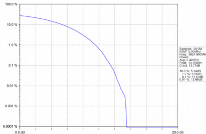
n78d_30kHz_SISO_NTNV_80MHz_CP-OFDM QPSK_3624.99MHz_Outer_Full
