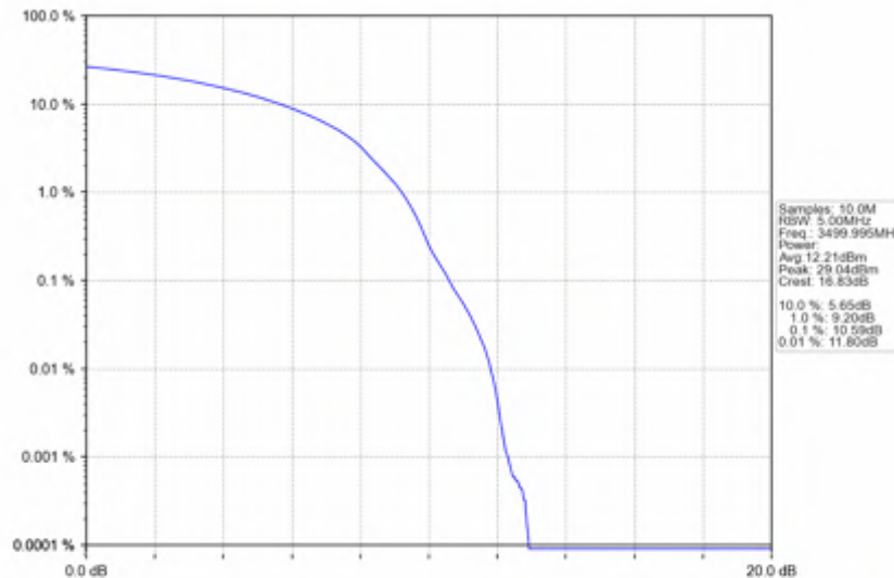
n78e_15kHz_SISO_NTNV_20MHz_DFT-s-OFDM_16_QAM_3499.995MHz_Outer_Full
