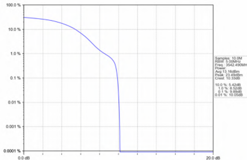
n78e_15kHz_SISO_NTNV_15MHz_DFT-s-OFDM PI/2 BPSK_3542.49MHz_Outer_Full
