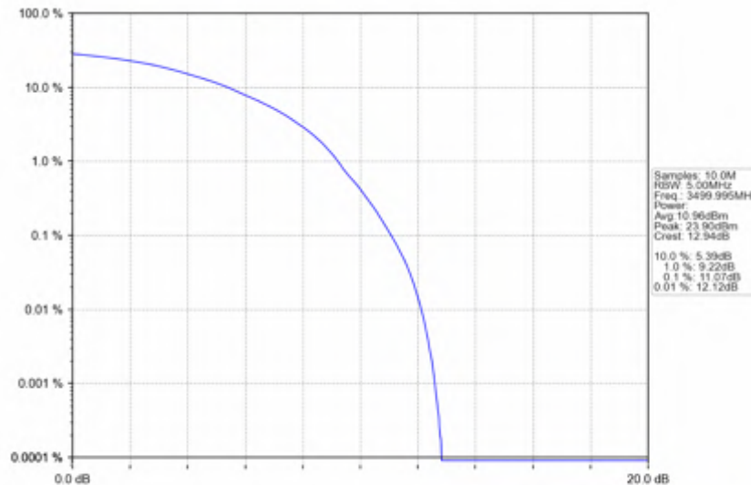
n78e_15kHz_SISO_NTNV_25MHz_DFT-s-OFDM_64_QAM_3499.995MHz_Outer_Full
