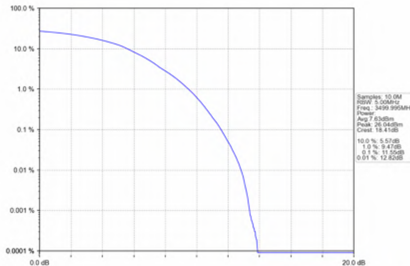
n78e_15kHz_SISO_NTNV_50MHz_DFT-s-OFDM QPSK_3499.995MHz_Outer_Full
