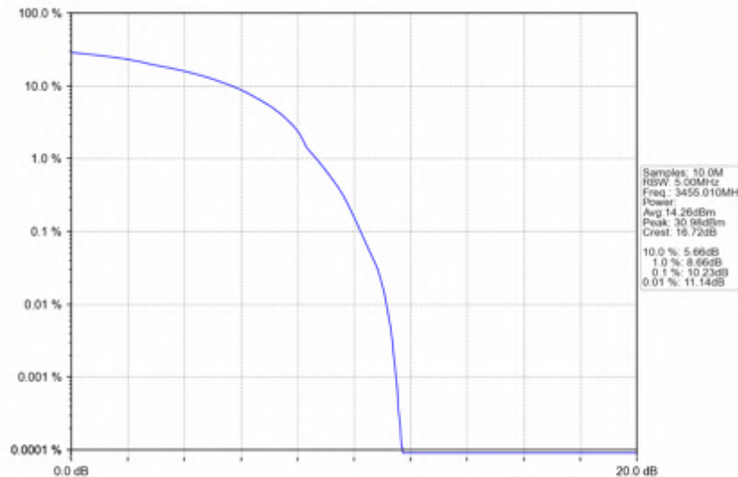
n78e_30kHz_SISO_NTNV_10MHz_DFT-s-OFDM_256_QAM_3455.01MHz_Outer_Full
