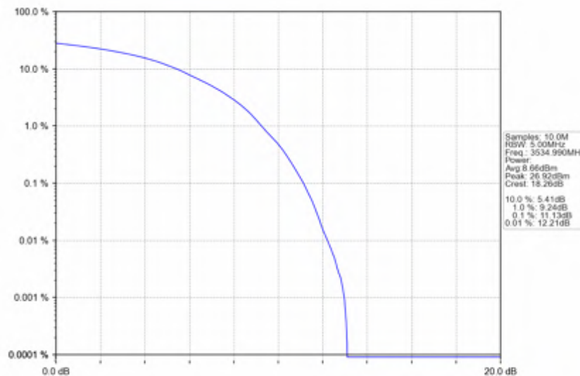
n78e_15kHz_SISO_NTNV_30MHz_DFT-s-OFDM_256_QAM_3534.99MHz_Outer_Full
