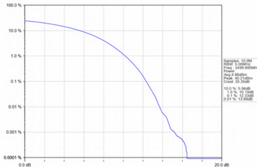
n78e_15kHz_SISO_NTNV_40MHz_CP-OFDM_256_QAM_3499.995MHz_Outer_Full
