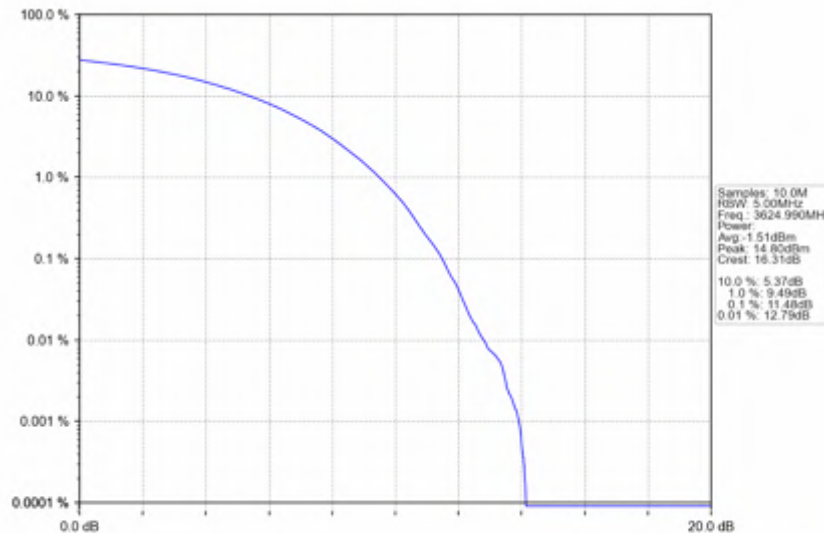
n78d_30kHz_SISO_NTNV_100MHz_CP-OFDM_256_QAM_3624.99MHz_Outer_Full
