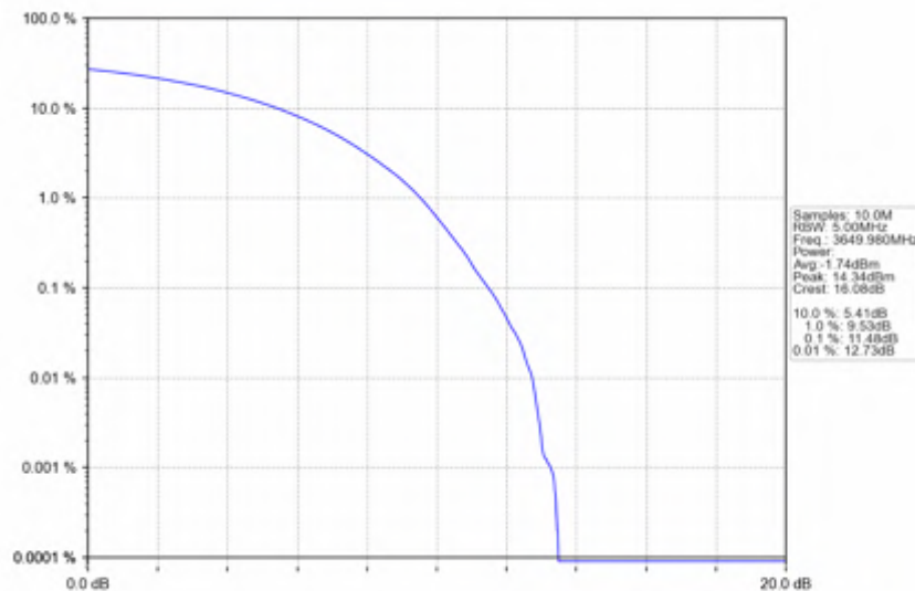
n78d_30kHz_SISO_NTNV_100MHz_CP-OFDM 16 QAM_3649.98MHz_Outer_Full
