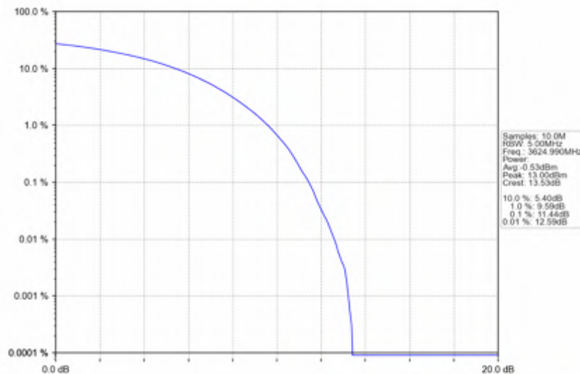
n78d_30kHz_SISO_NTNV_80MHz_CP-OFDM_256_QAM_3624.99MHz_Outer_Full
