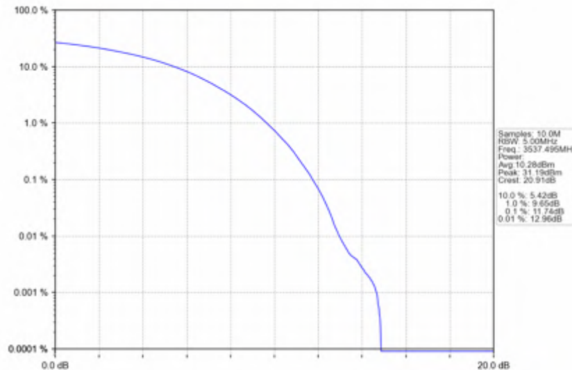
n78e_15kHz_SISO_NTNV_25MHz_CP-OFDM_64_QAM_3537.495MHz_Outer_Full
