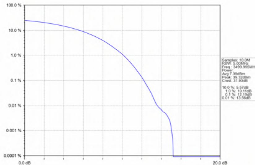
n78e_15kHz_SISO_NTNV_50MHz_CP-OFDM QPSK_3499.995MHz_Outer_Full
