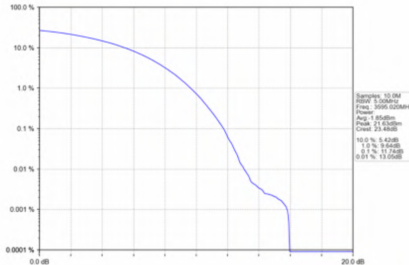
n78d_30kHz_SISO_NTNV_90MHz_CP-OFDM_256_QAM_3595.02MHz_Outer_Full
