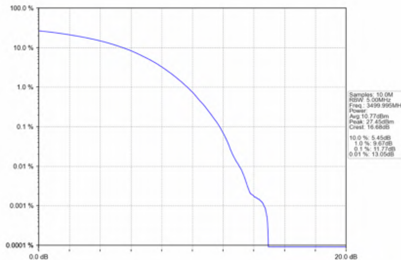
n78e_15kHz_SISO_NTNV_25MHz_CP-OFDM QPSK_3499.995MHz_Outer_Full
