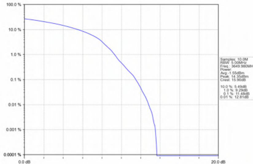
n78d_30kHz_SISO_NTNV_100MHz_DFT-s-OFDM 16 QAM_3649.98MHz_Outer_Full
