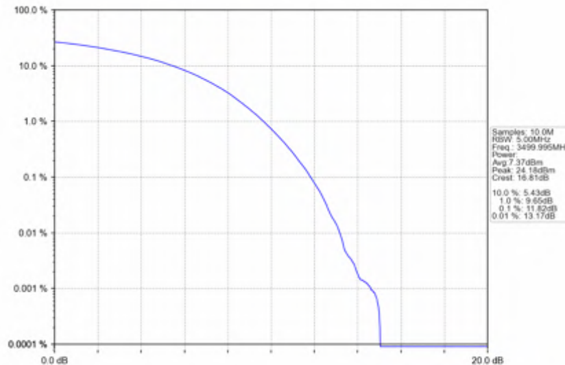
n78e_15kHz_SISO_NTNV_25MHz_CP-OFDM_256_QAM_3499.995MHz_Outer_Full
