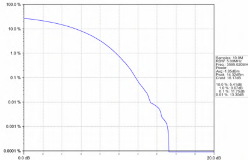
n78d_30kHz_SISO_NTNV_90MHz_CP-OFDM_QPSK_3595.02MHz_Outer_Full
