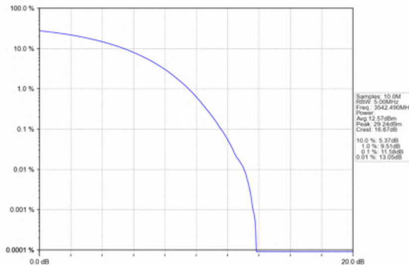
n78e_15kHz_SISO_NTNV_15MHz_CP-OFDM 64 QAM_3542.49MHz_Outer_Full
