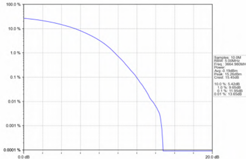
n78d_30kHz_SISO_NTNV_70MHz_CP-OFDM 64 QAM_3664.98MHz_Outer_Full
