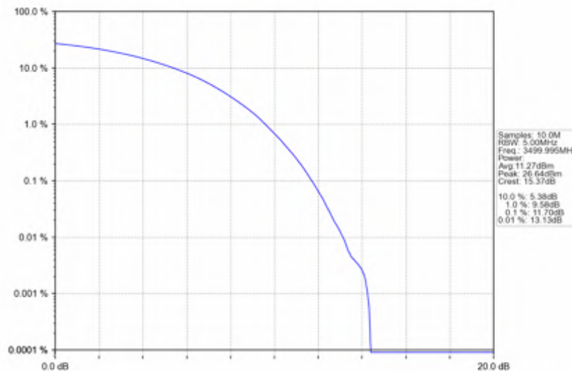
n78e_15kHz_SISO_NTNV_20MHz_CP-OFDM 64 QAM_3499.995MHz_Outer_Full
