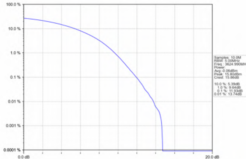
n78d_30kHz_SISO_NTNV_70MHz_CP-OFDM 64 QAM_3624.99MHz_Outer_Full
