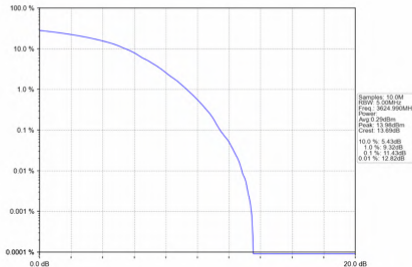
n78d_30kHz_SISO_NTNV_70MHz_DFT-s-OFDM_256_QAM_3624.99MHz_Outer_Full
