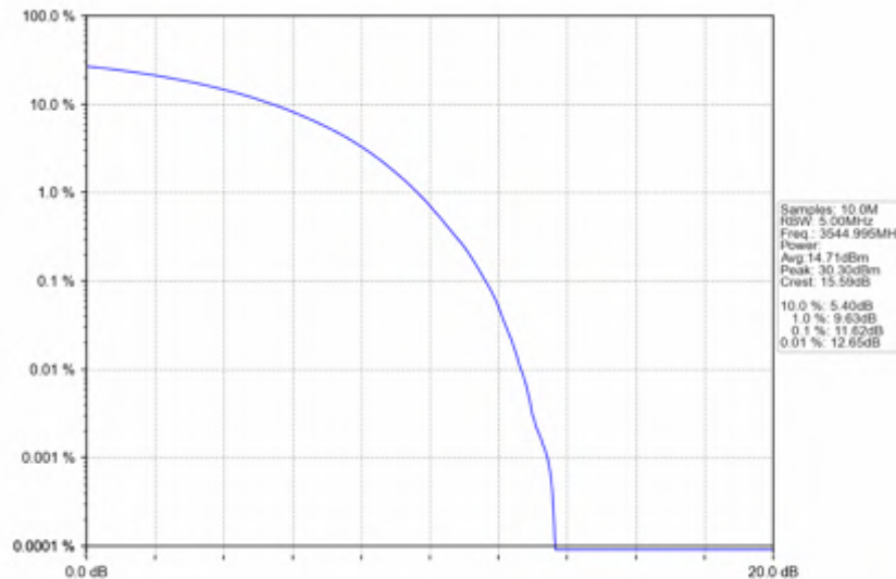
n78e_15kHz_SISO_NTNV_10MHz_CP-OFDM_16_QAM_3544.995MHz_Outer_Full
