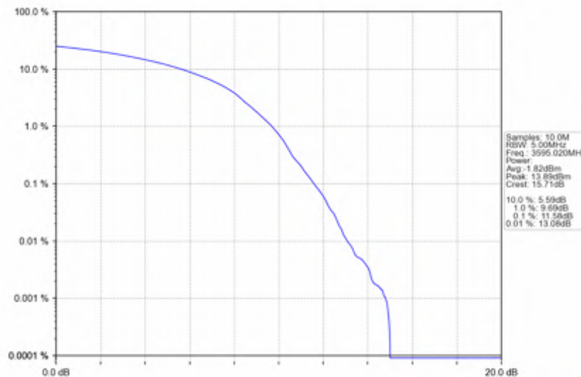
n78d_30kHz_SISO_NTV_90MHz_DFT-s-OFDM 64 QAM_3595.02MHz_Outer_Full
