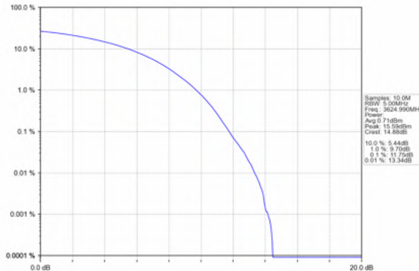
n78d_30kHz_SISO_NTNV_60MHz_CP-OFDM_256_QAM_3624.99MHz_Outer_Full
