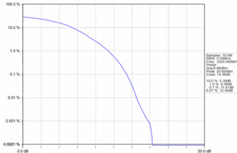
n78e_15kHz_SISO_NTNV_50MHz_DFT-s-OFDM_256_QAM_3525MHz_Outer_Full
