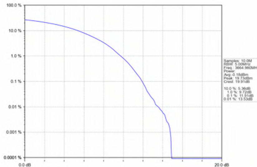
n78d_30kHz_SISO_NTNV_70MHz_CP-OFDM 16 QAM_3664.98MHz_Outer_Full
