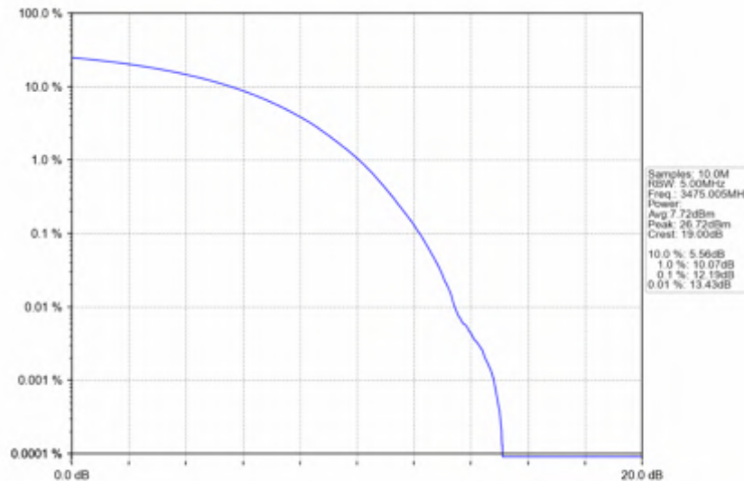
n78e_15kHz_SISO_NTNV_50MHz_CP-OFDM_QPSK_3475.005MHz_Outer_Full
