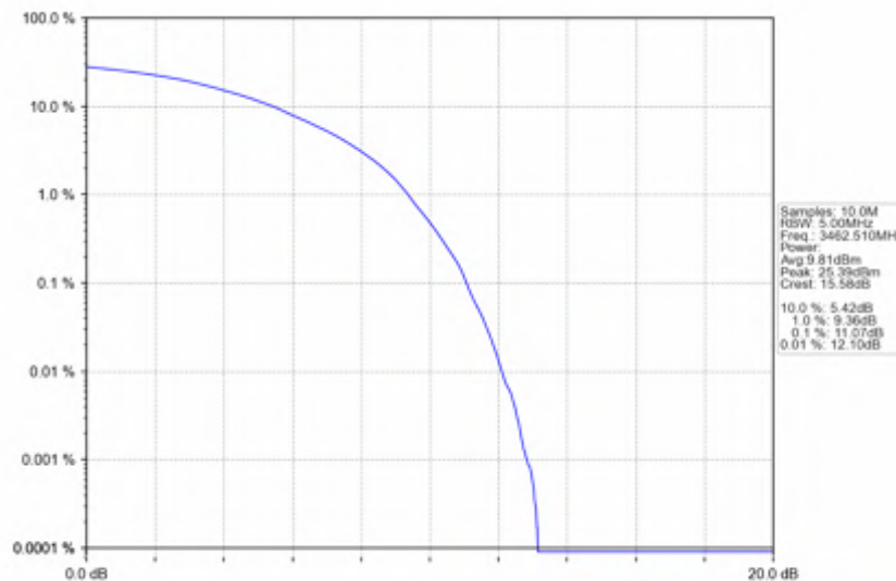
n78e_15kHz_SISO_NTNV_25MHz_DFT-s-OFDM_256_QAM_3462.51MHz_Outer_Full
