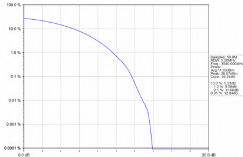
n78e_15kHz_SISO_NTNV_20MHz_CP-OFDM QPSK_3540MHz_Outer_Full
