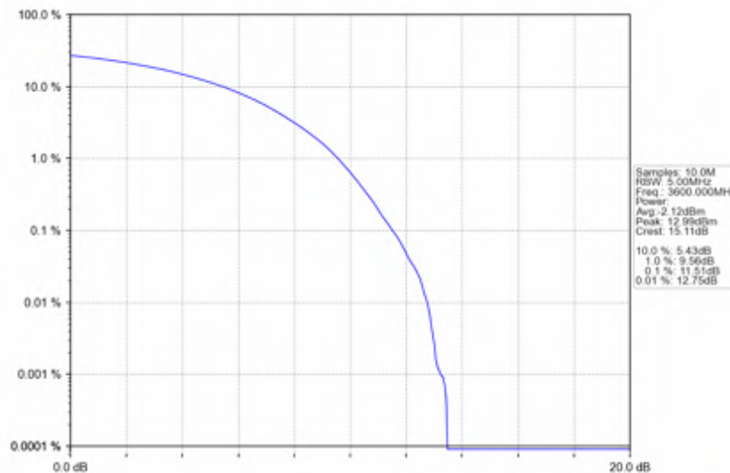
n78d_30kHz_SISO_NTNV_100MHz_CP-OFDM_16_QAM_3600MHz_Outer_Full
