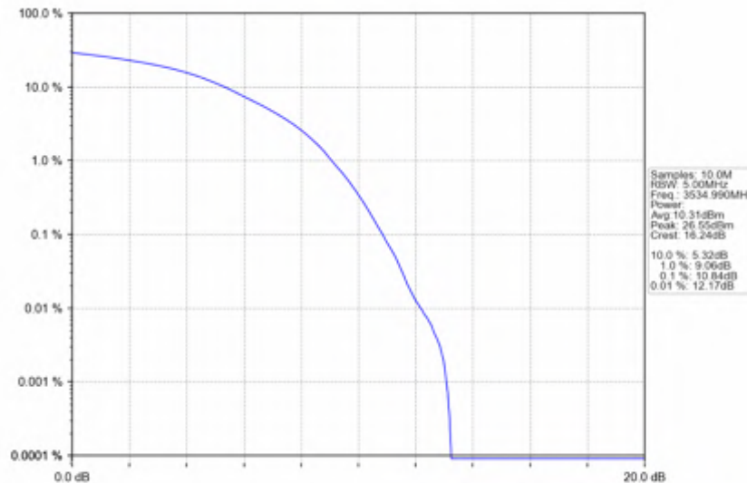
n78e_15kHz_SISO_NTNV_30MHz_DFT-s-OFDM 64 QAM_3534.99MHz_Outer_Full
