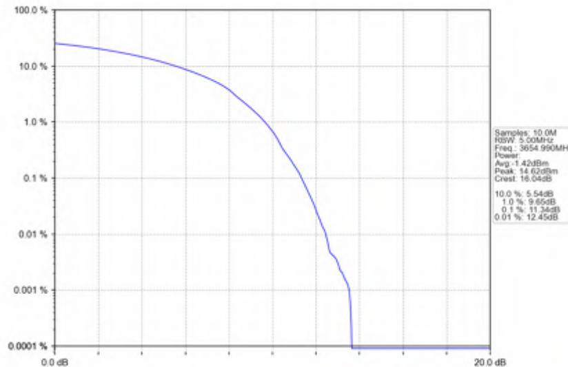
n78d_30kHz_SISO_NTNV_90MHz_DFT-s-OFDM_QPSK_3654.99MHz_Outer_Full
