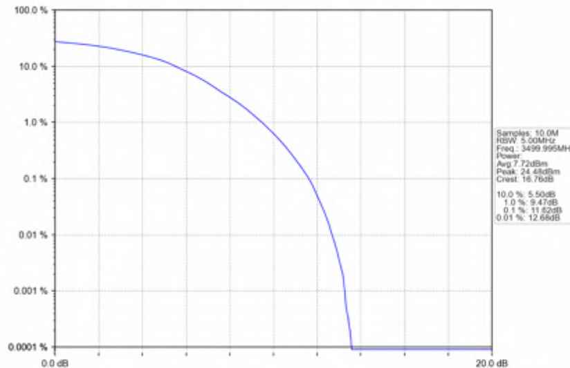
n78e_15kHz_SISO_NTNV_50MHz_DFT-s-OFDM_16_QAM_3499.995MHz_Outer_Full
