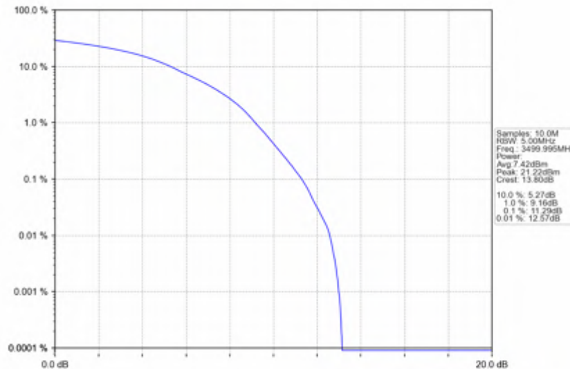
n78e_15kHz_SISO_NTNV_40MHz_DFT-s-OFDM_256_QAM_3499.995MHz_Outer_Full
