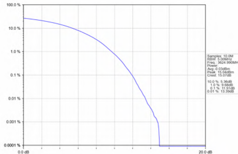
n78d_30kHz_SISO_NTNV_70MHz_CP-OFDM_16_QAM_3624.99MHz_Outer_Full
