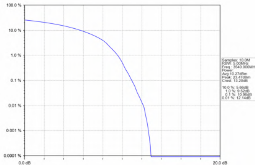
n78e_15kHz_SISO_NTNV_20MHz_DFT-s-OFDM_256_QAM_3540MHz_Outer_Full
