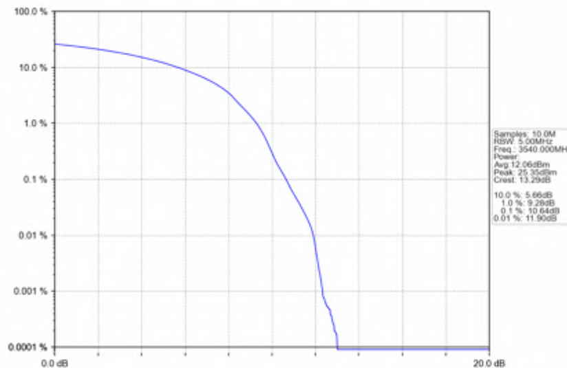
n78e_15kHz_SISO_NTNV_20MHz_DFT-s-OFDM 16 QAM_3540MHz_Outer_Full
