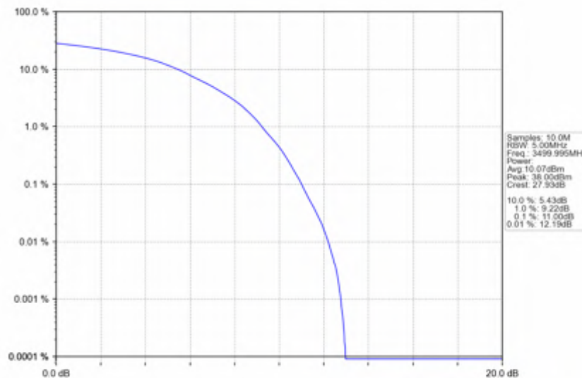
n78e_15kHz_SISO_NTNV_30MHz_DFT-s-OFDM_16_QAM_3499.995MHz_Outer_Full
