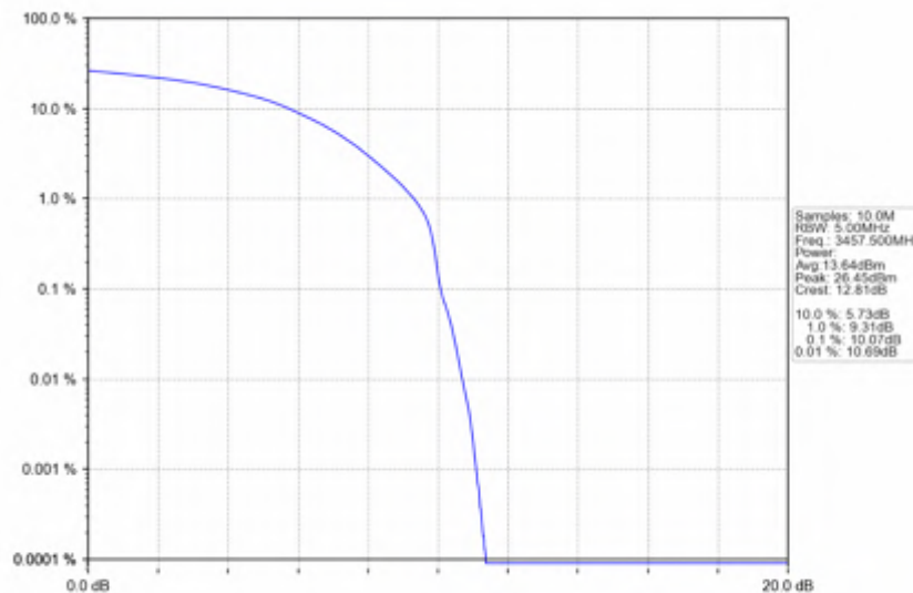
n78e_15kHz_SISO_NTNV_15MHz_DFT-s-OFDM QPSK_3457.5MHz_Outer_Full
