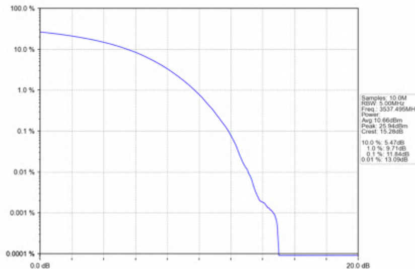
n78e_15kHz_SISO_NTNV_25MHz_CP-OFDM QPSK_3537.495MHz_Outer_Full
