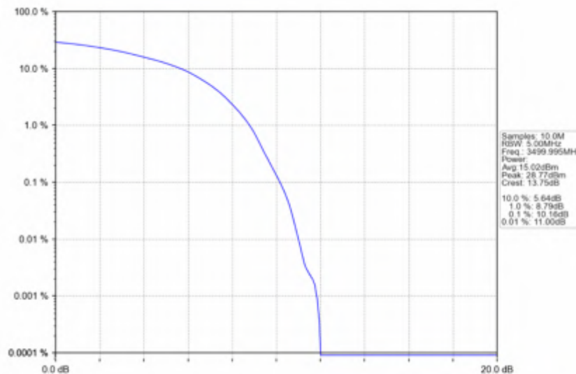
n78e_15kHz_SISO_NTNV_10MHz_DFT-s-OFDM_64_QAM_3499.995MHz_Outer_Full
