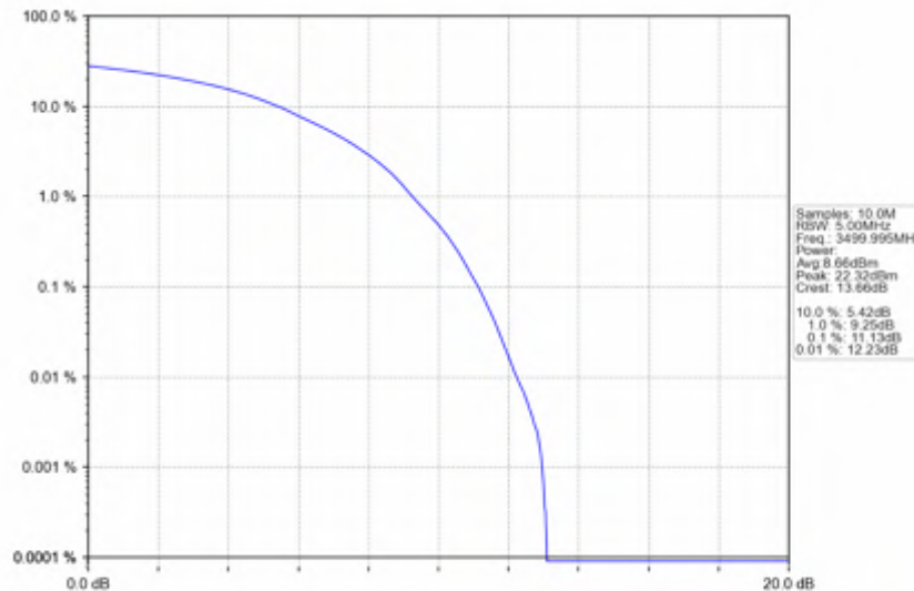
n78e_15kHz_SISO_NTNV_30MHz_DFT-s-OFDM_256_QAM_3499.995MHz_Outer_Full
