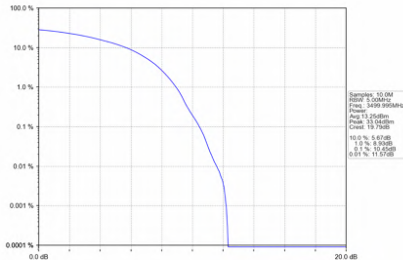
n78e_15kHz_SISO_NTNV_10MHz_DFT-s-OFDM_256_QAM_3499.995MHz_Outer_Full
