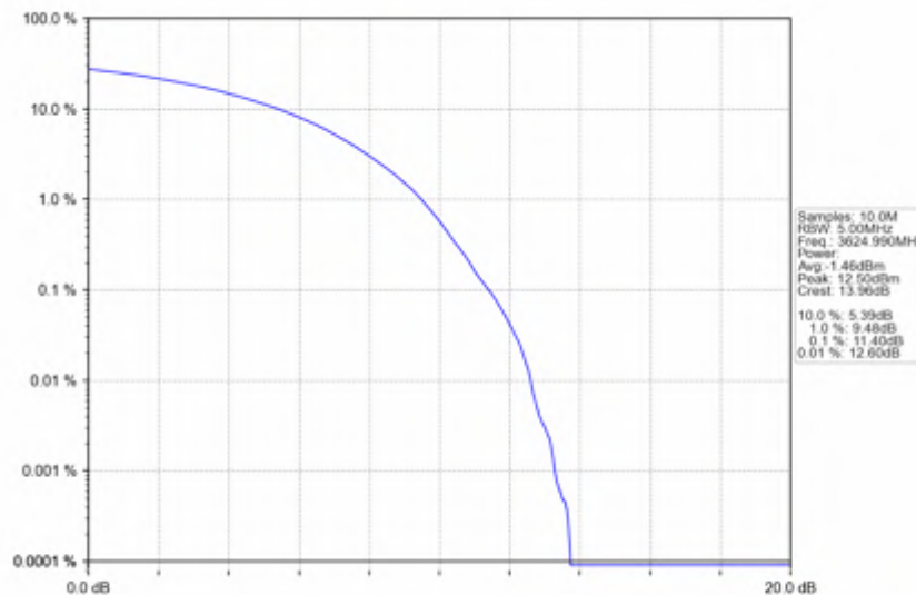
n78d_30kHz_SISO_NTNV_100MHz_CP-OFDM_16_QAM_3624.99MHz_Outer_Full
