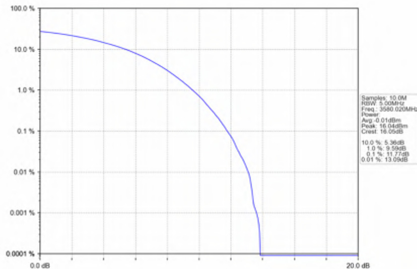
n78d_30kHz_SISO_NTNV_60MHz_CP-OFDM 64 QAM_3580.02MHz_Outer_Full
