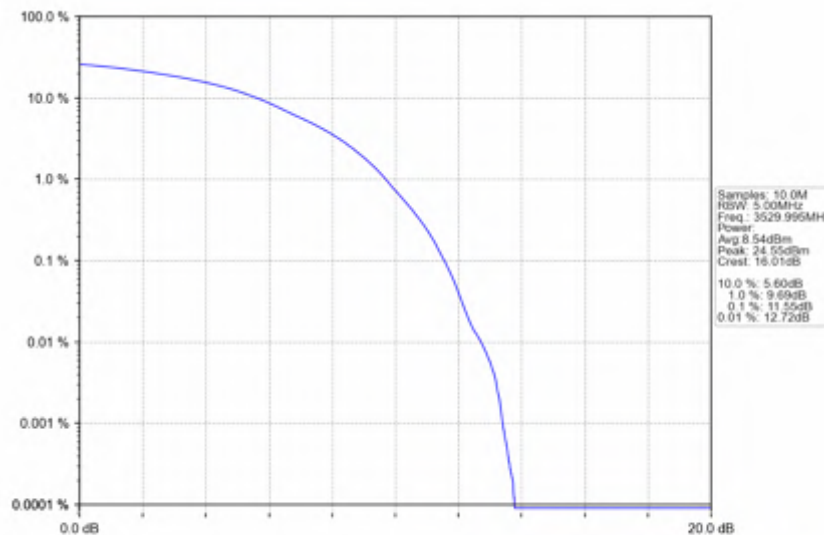
n78e_15kHz_SISO_NTNV_40MHz_DFT-s-OFDM_64_QAM_3529.995MHz_Outer_Full
