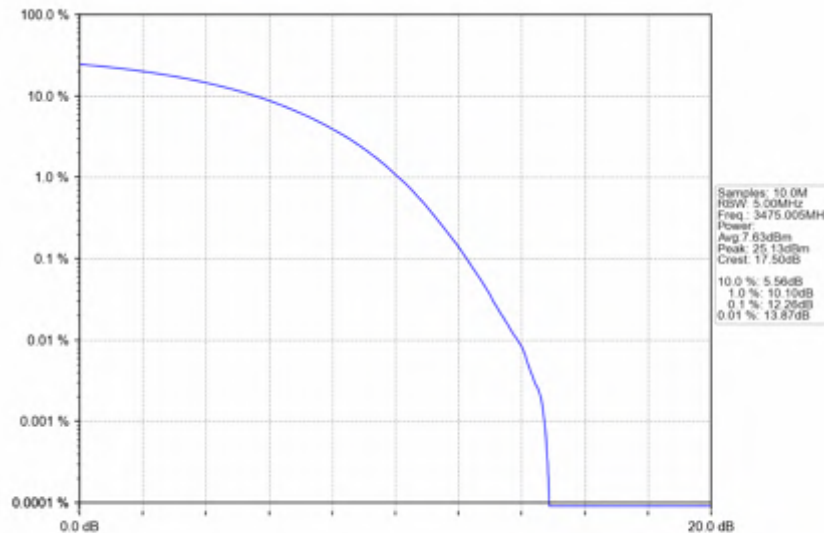
n78e_15kHz_SISO_NTNV_50MHz_CP-OFDM_16_QAM_3475.005MHz_Outer_Full
