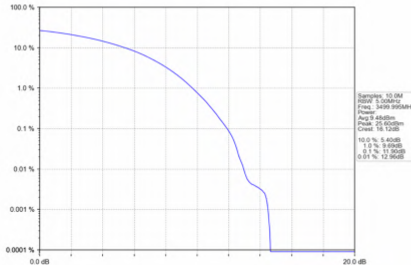
n78e_15kHz_SISO_NTNV_30MHz_CP-OFDM 64 QAM_3499.995MHz_Outer_Full
