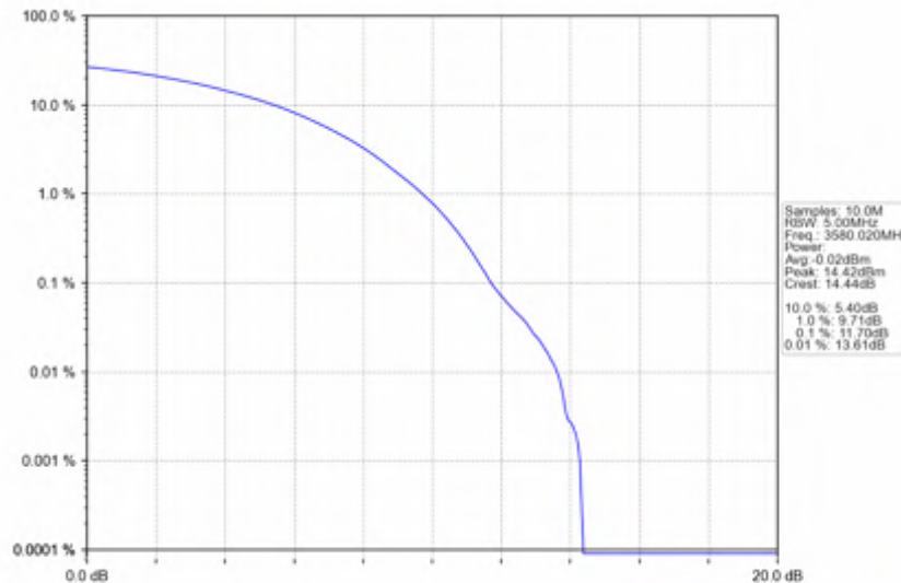
n78d_30kHz_SISO_NTNV_60MHz_CP-OFDM_256_QAM_3580.02MHz_Outer_Full
