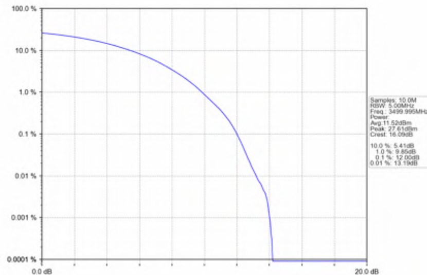
n78e_15kHz_SISO_NTNV_20MHz_CP-OFDM QPSK_3499.995MHz_Outer_Full
