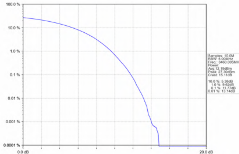
n78e_15kHz_SISO_NTNV_20MHz_CP-OFDM_16_QAM_3460.005MHz_Outer_Full
