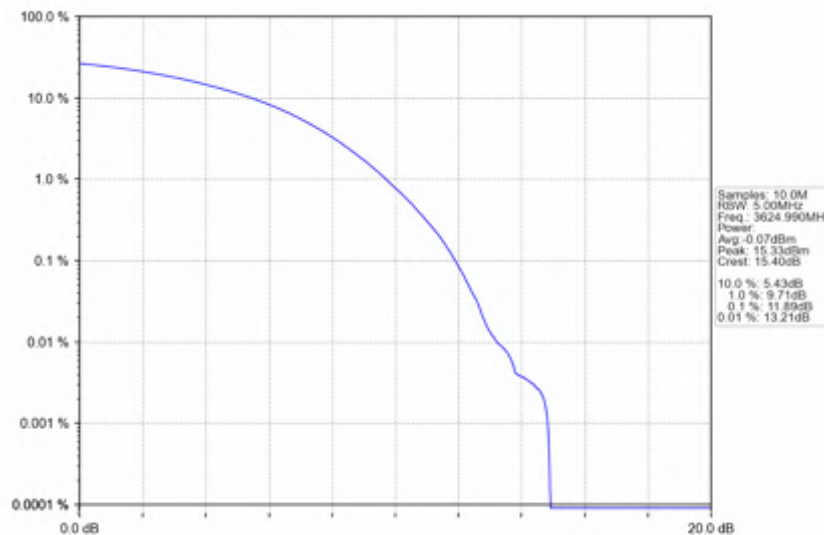
n78d_30kHz_SISO_NTNV_70MHz_CP-OFDM_256_QAM_3624.99MHz_Outer_Full
