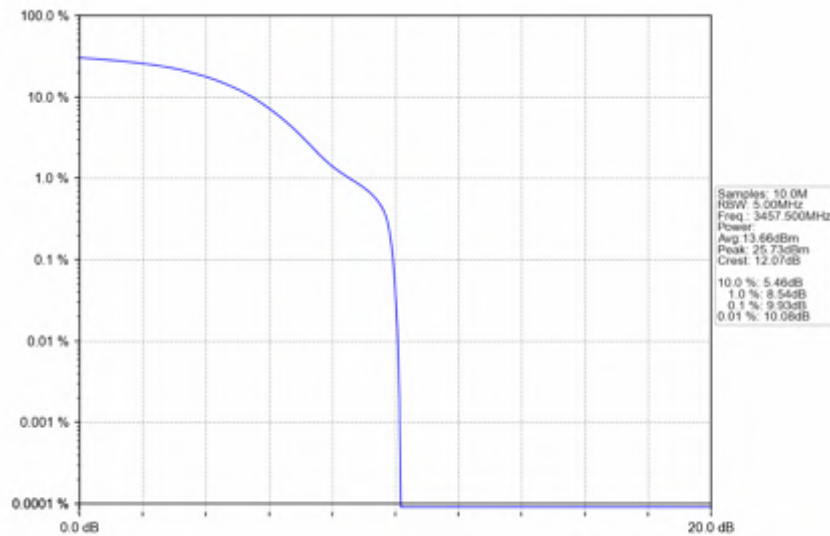
n78e_15kHz_SISO_NTNV_15MHz_DFT-s-OFDM_PI/2_BPSK_3457.5MHz_Outer_Full
