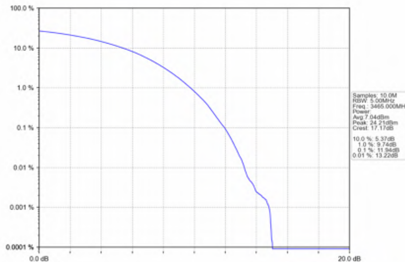
n78e_15kHz_SISO_NTNV_30MHz_CP-OFDM_256_QAM_3465MHz_Outer_Full
