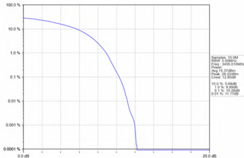
n78e_15kHz_SISO_NTNV_10MHz_DFT-s-OFDM 64 QAM_3455.01MHz_Outer_Full
