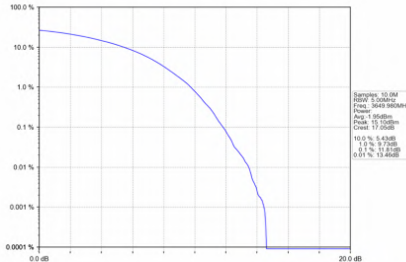
n78d_30kHz_SISO_NTNV_100MHz_CP-OFDM 64 QAM_3649.98MHz_Outer_Full
