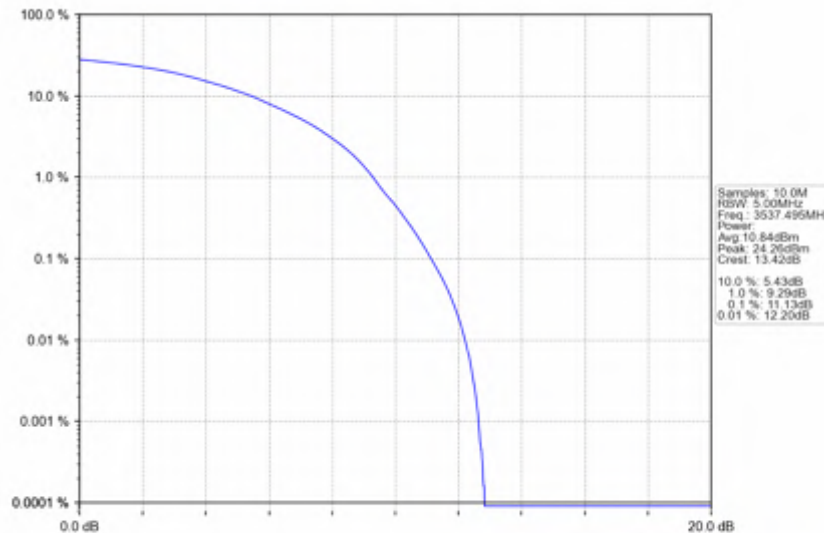
n78e_15kHz_SISO_NTNV_25MHz_DFT-s-OFDM_64_QAM_3537.495MHz_Outer_Full
