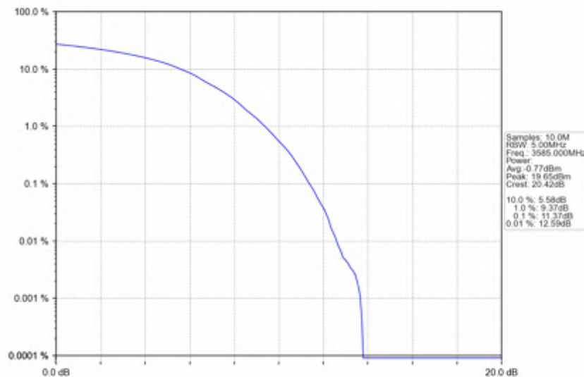
n78d_30kHz_SISO_NTV_70MHz_DFT-s-OFDM 64 QAM_3585MHz_Outer_Full
