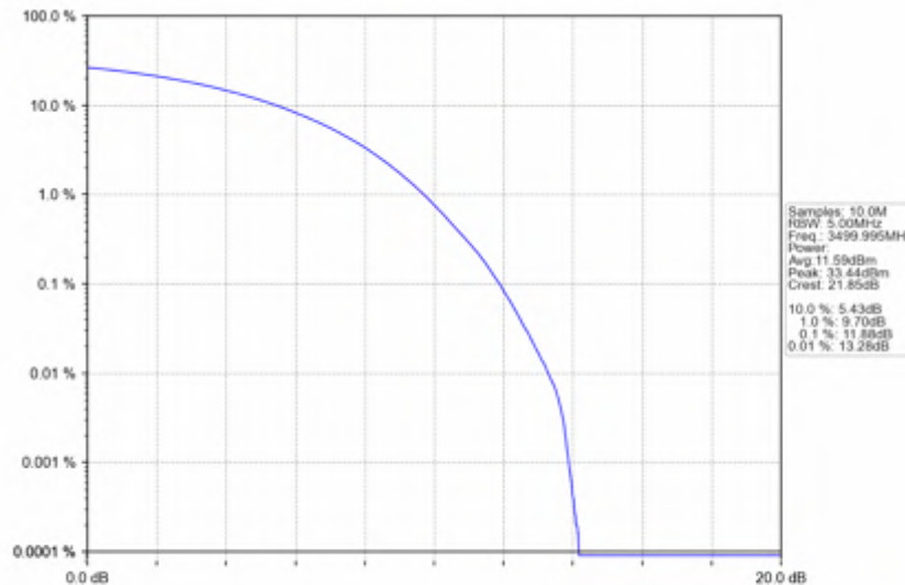
n78e_15kHz_SISO_NTNV_20MHz_CP-OFDM_16_QAM_3499.995MHz_Outer_Full
