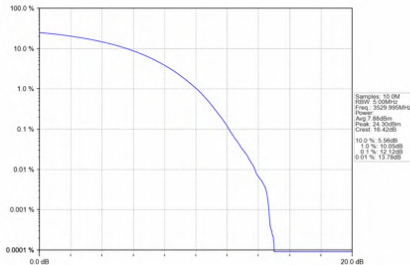
n78e_15kHz_SISO_NTNV_40MHz_CP-OFDM_64_QAM_3529.995MHz_Outer_Full
