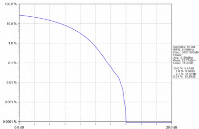
n78e_15kHz_SISO_NTNV_15MHz_CP-OFDM_16_QAM_3457.5MHz_Outer_Full
