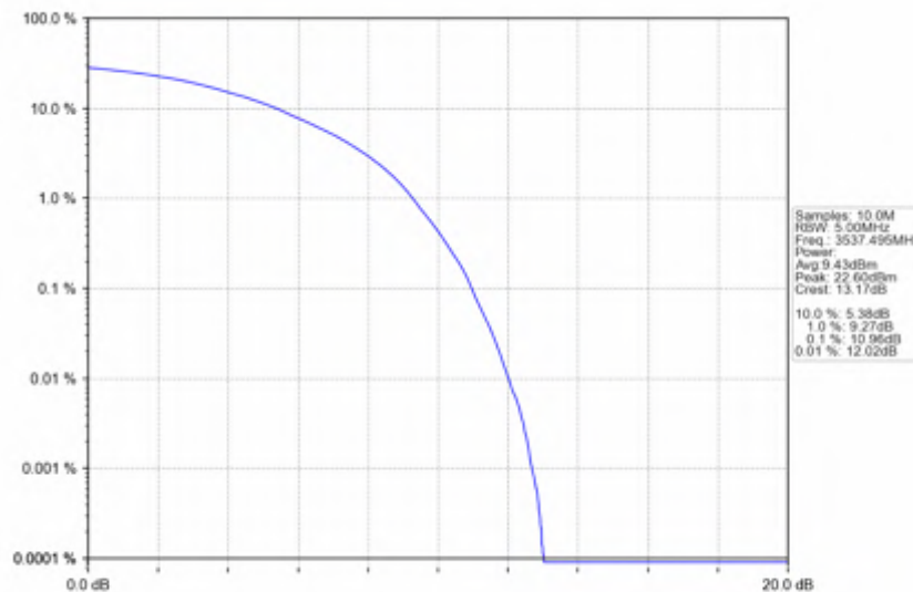
n78e_15kHz_SISO_NTNV_25MHz_DFT-s-OFDM 256 QAM_3537.495MHz_Outer_Full
