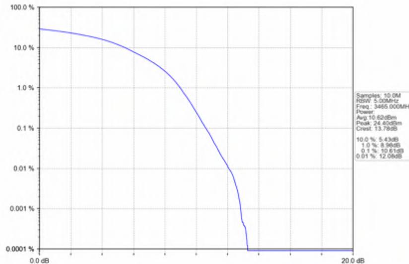
n78e_15kHz_SISO_NTNV_30MHz_DFT-s-OFDM QPSK_3465MHz_Outer_Full
