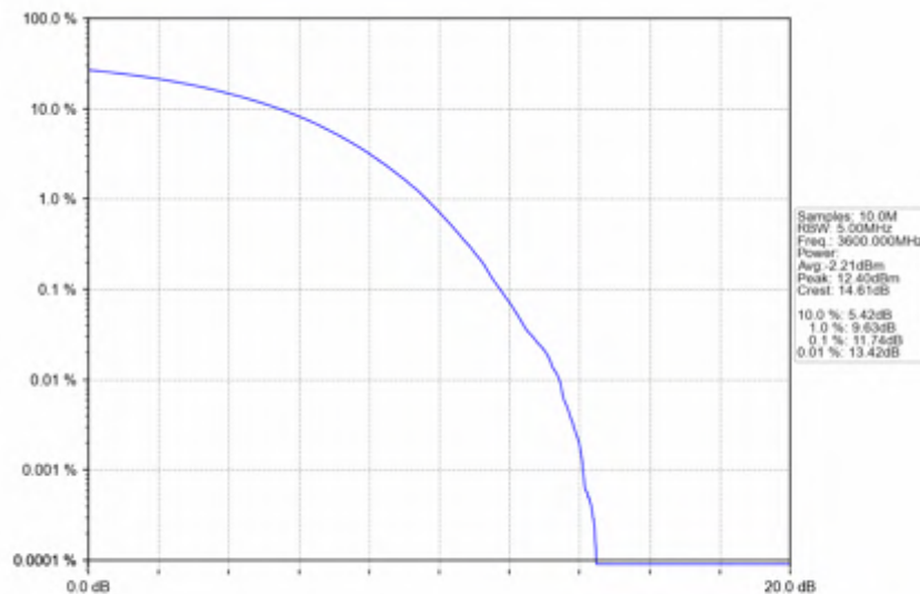
n78d_30kHz_SISO_NTNV_100MHz_CP-OFDM 64 QAM_3600MHz_Outer_Full
