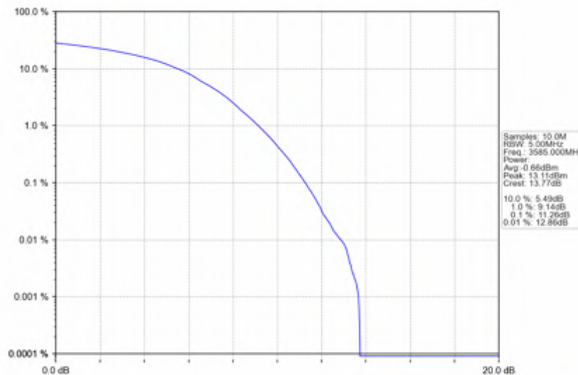
n78d_30kHz_SISO_NTNV_70MHz_DFT-s-OFDM_QPSK_3585MHz_Outer_Full
