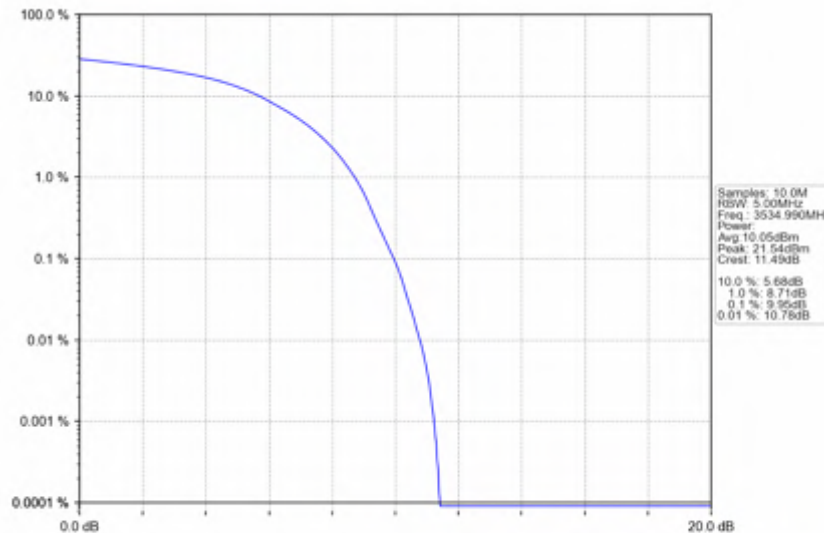
n78e_15kHz_SISO_NTNV_30MHz_DFT-s-OFDM PI/2 BPSK_3534.99MHz_Outer_Full
