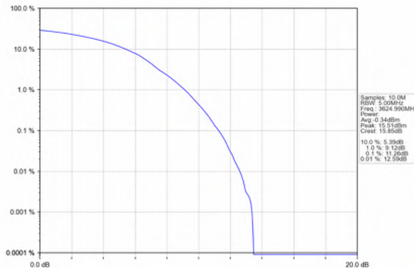
n78d_30kHz_SISO_NTV_80MHz_DFT-s-OFDM 64 QAM_3624.99MHz_Outer_Full
