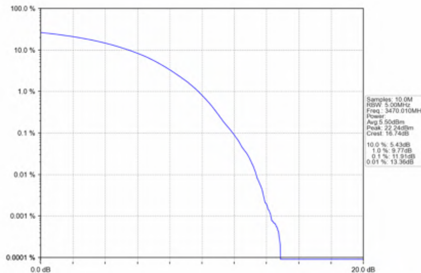
n78e_15kHz_SISO_NTNV_40MHz_CP-OFDM_256_QAM_3470.01MHz_Outer_Full
