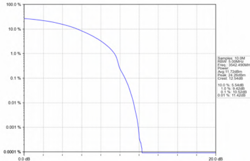
n78e_15kHz_SISO_NTNV_15MHz_DFT-s-OFDM_256_QAM_3542.49MHz_Outer_Full
