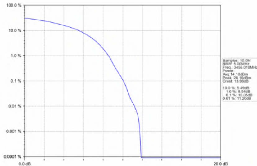
n78e_15kHz_SISO_NTNV_10MHz_DFT-s-OFDM_256_QAM_3455.01MHz_Outer_Full
