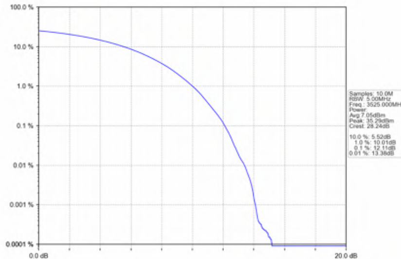
n78e_15kHz_SISO_NTNV_50MHz_CP-OFDM 64 QAM_3525MHz_Outer_Full
