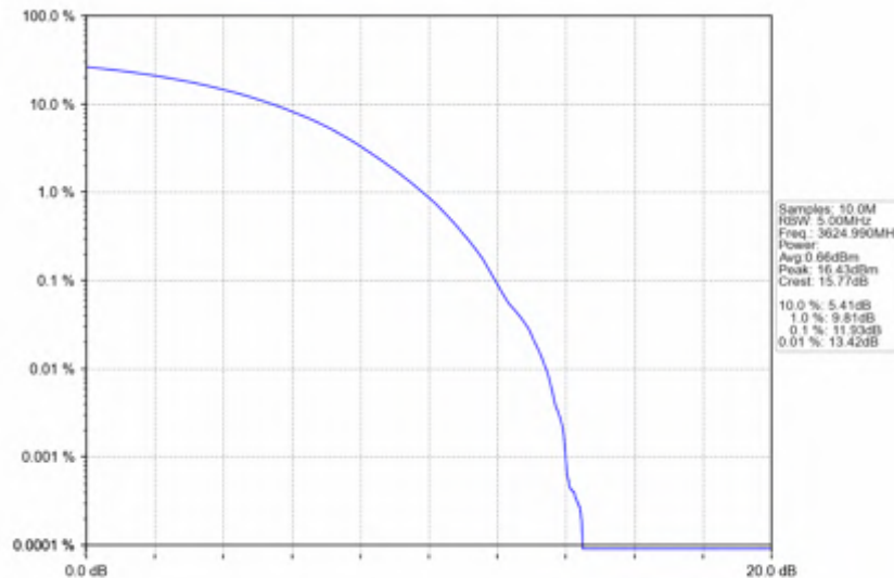
n78d_30kHz_SISO_NTNV_60MHz_CP-OFDM_QPSK_3624.99MHz_Outer_Full
