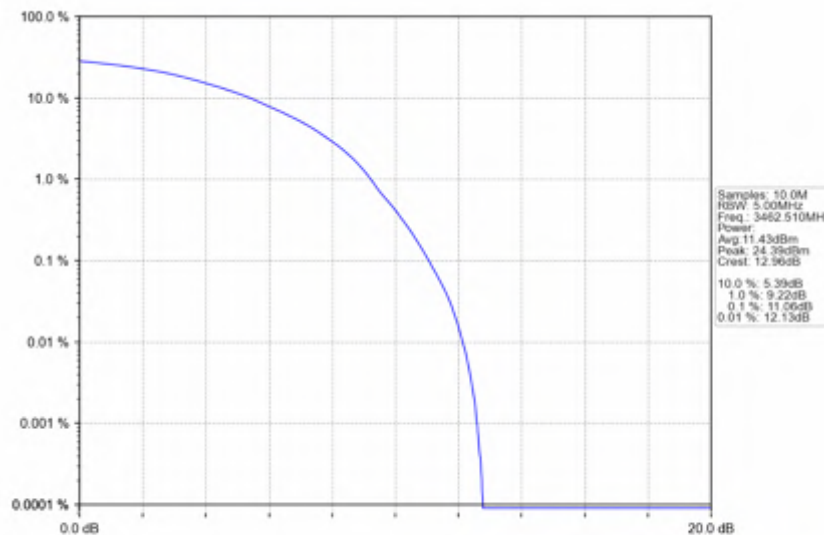
n78e_15kHz_SISO_NTNV_25MHz_DFT-s-OFDM_64_QAM_3462.51MHz_Outer_Full
