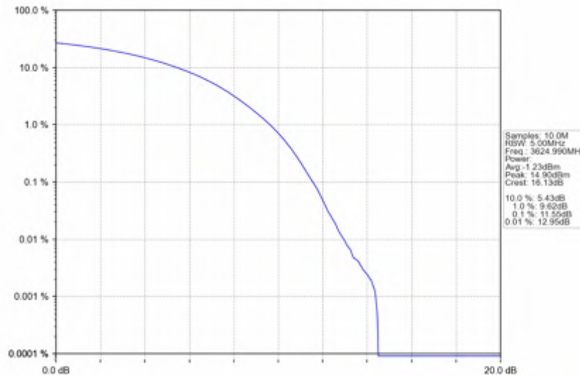
n78d_30kHz_SISO_NTNV_90MHz_CP-OFDM 64 QAM_3624.99MHz_Outer_Full
