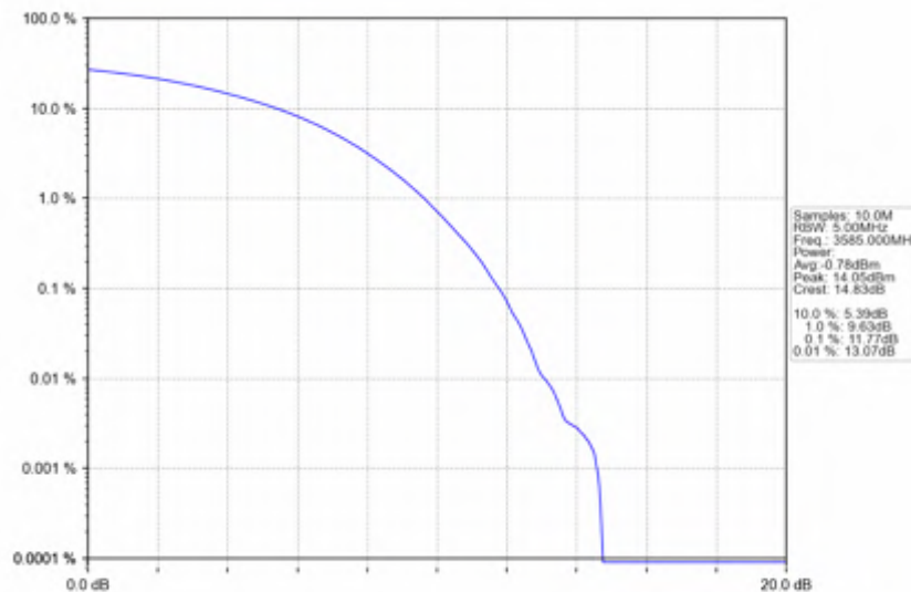
n78d_30kHz_SISO_NTNV_70MHz_CP-OFDM_256_QAM_3585MHz_Outer_Full
