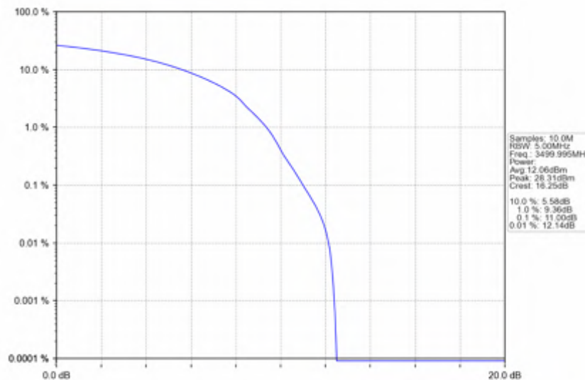
n78e_15kHz_SISO_NTNV_20MHz_DFT-s-OFDM 64 QAM_3499.995MHz_Outer_Full
