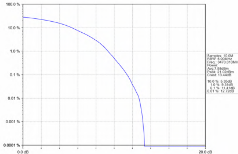
n78e_15kHz_SISO_NTNV_40MHz_DFT-s-OFDM_256_QAM_3470.01MHz_Outer_Full
