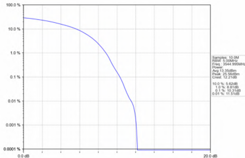
n78e_15kHz_SISO_NTNV_10MHz_DFT-s-OFDM 256 QAM_3544.995MHz_Outer_Full
