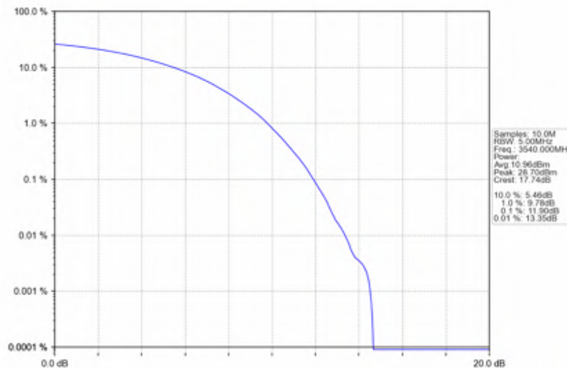
n78e_15kHz_SISO_NTNV_20MHz_CP-OFDM 64 QAM_3540MHz_Outer_Full
