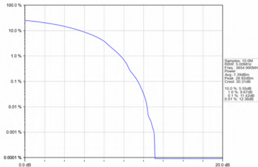
n78d_30kHz_SISO_NTV_90MHz_DFT-s-OFDM 16 QAM_3654.99MHz_Outer_Full
