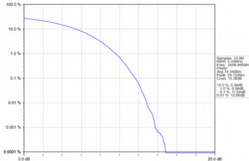
n78e_15kHz_SISO_NTNV_10MHz_CP-OFDM 64 QAM_3499.995MHz_Outer_Full
