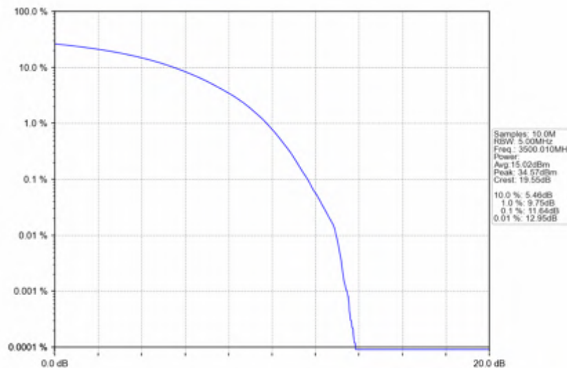
n78e_30kHz_SISO_NTNV_10MHz_CP-OFDM_QPSK_3500.01MHz_Outer_Full
