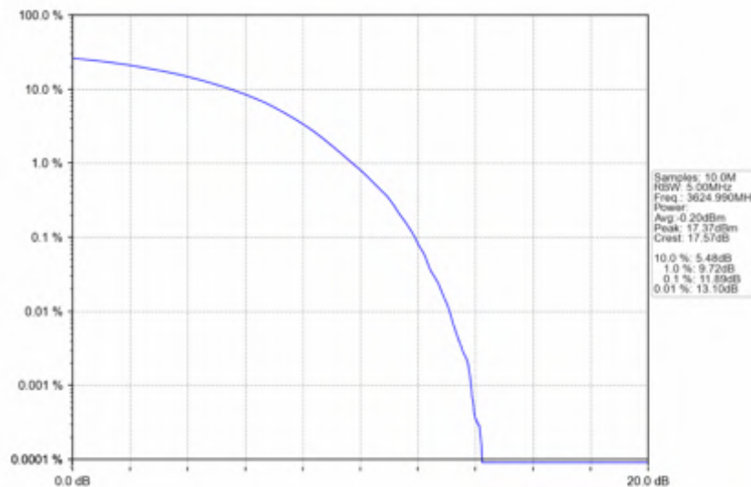
n78d_30kHz_SISO_NTNV_70MHz_CP-OFDM QPSK_3624.99MHz_Outer_Full
