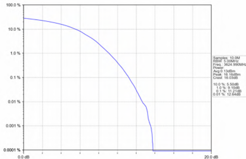
n78d_30kHz_SISO_NTNV_70MHz_DFT-s-OFDM_QPSK_3624.99MHz_Outer_Full
