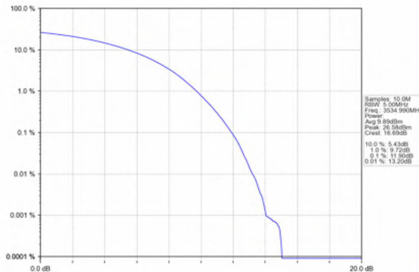
n78e_15kHz_SISO_NTNV_30MHz_CP-OFDM QPSK_3534.99MHz_Outer_Full
