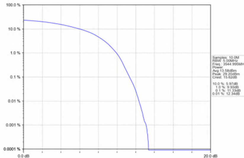
n78e_15kHz_SISO_NTNV_10MHz_DFT-s-OFDM_64_QAM_3544.995MHz_Outer_Full
