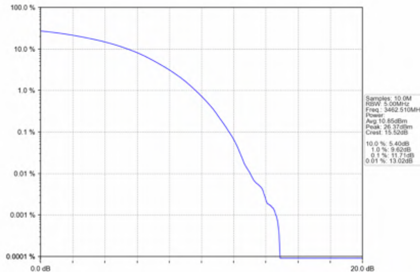
n78e_15kHz_SISO_NTNV_25MHz_CP-OFDM_64_QAM_3462.51MHz_Outer_Full
