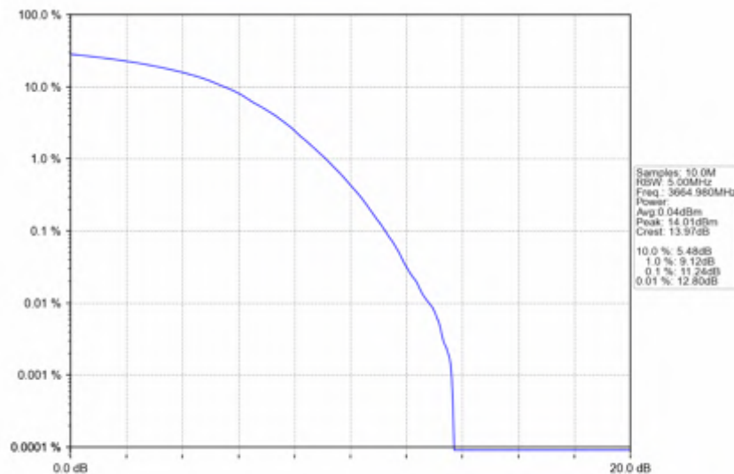
n78d_30kHz_SISO_NTNV_70MHz_DFT-s-OFDM_QPSK_3664.98MHz_Outer_Full
