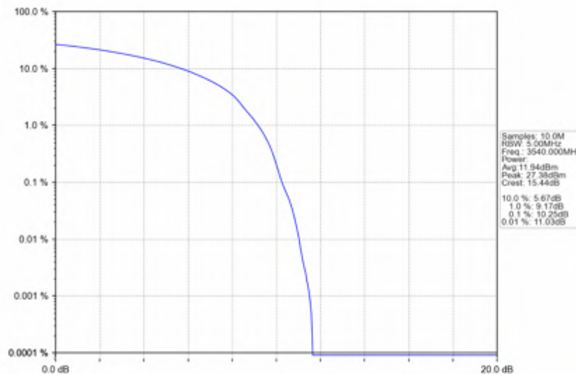
n78e_15kHz_SISO_NTNV_20MHz_DFT-s-OFDM QPSK_3540MHz_Outer_Full
