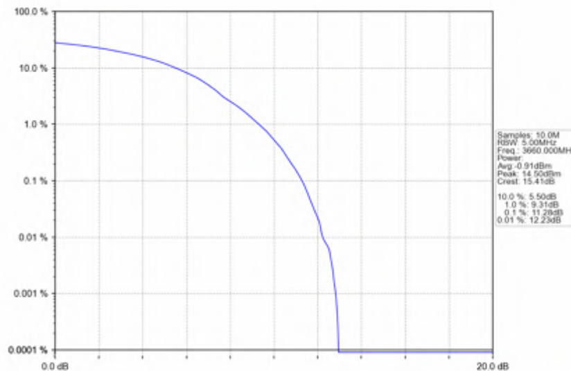
n78d_30kHz_SISO_NTNV_80MHz_DFT-s-OFDM_QPSK_3660MHz_Outer_Full
