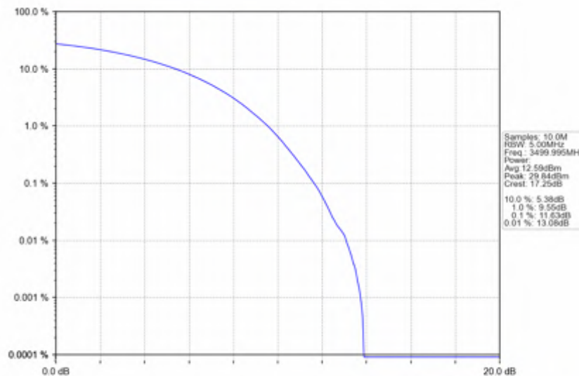
n78e_15kHz_SISO_NTNV_15MHz_CP-OFDM 64 QAM_3499.995MHz_Outer_Full
