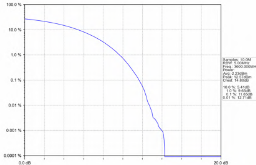
n78d_30kHz_SISO_NTNV_100MHz_CP-OFDM_256_QAM_3600MHz_Outer_Full
