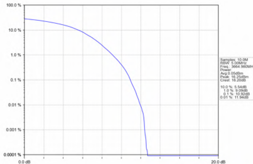
n78d_30kHz_SISO_NTNV_70MHz_DFT-s-OFDM_PI/2_BPSK_3664.98MHz_Outer_Full
