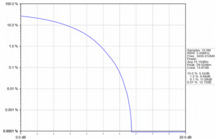
n78e_15kHz_SISO_NTNV_10MHz_CP-OFDM_16_QAM_3455.01MHz_Outer_Full
