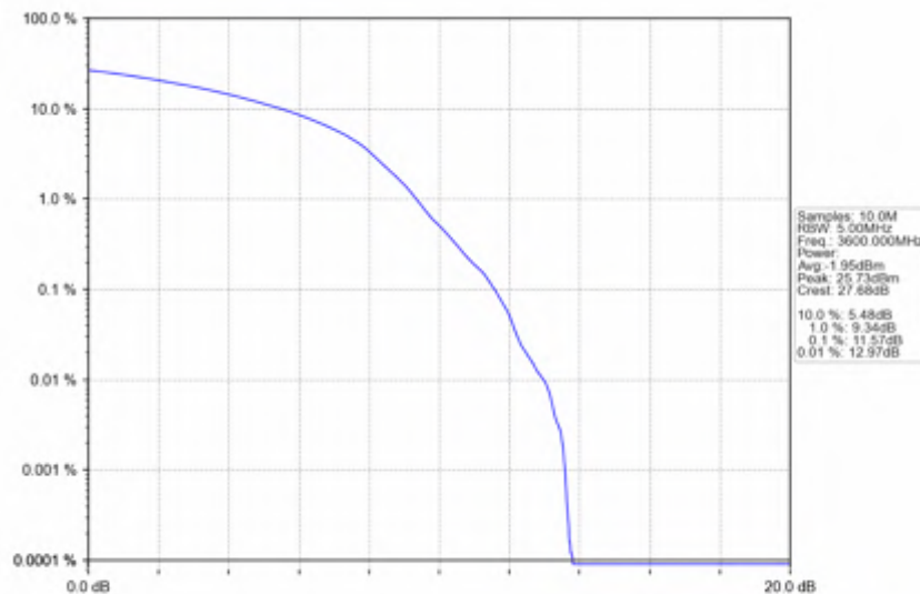
n78d_30kHz_SISO_NTNV_100MHz_DFT-s-OFDM_16_QAM_3600MHz_Outer_Full
