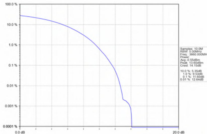
n78d_30kHz_SISO_NTNV_80MHz_CP-OFDM 64 QAM_3660MHz_Outer_Full
