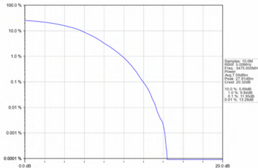
n78e_15kHz_SISO_NTNV_50MHz_DFT-s-OFDM 64 QAM_3475.005MHz_Outer_Full
