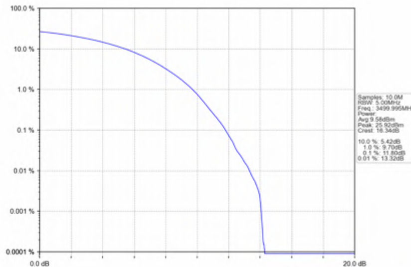
n78e_15kHz_SISO_NTNV_15MHz_CP-OFDM_256_QAM_3499.995MHz_Outer_Full
