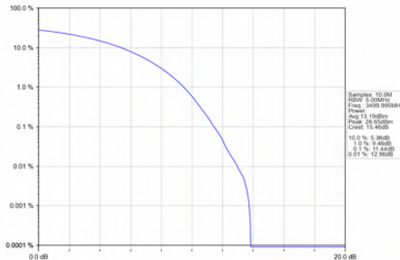
n78e_15kHz_SISO_NTNV_15MHz_CP-OFDM QPSK_3499.995MHz_Outer_Full
