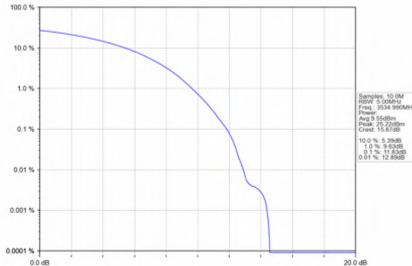
n78e_15kHz_SISO_NTNV_30MHz_CP-OFDM 64 QAM_3534.99MHz_Outer_Full
