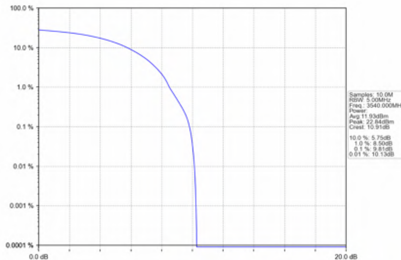
n78e_15kHz_SISO_NTNV_20MHz_DFT-s-OFDM PI/2 BPSK_3540MHz_Outer_Full
