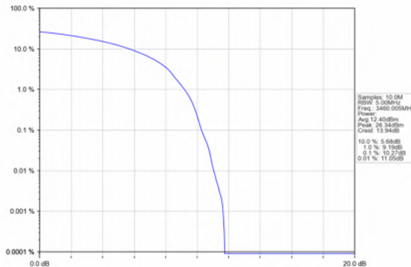
n78e_15kHz_SISO_NTNV_20MHz_DFT-s-OFDM QPSK_3460.005MHz_Outer_Full
