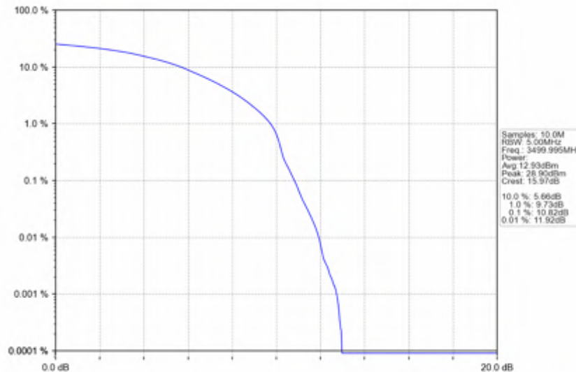
n78e_15kHz_SISO_NTNV_15MHz_DFT-s-OFDM_16_QAM_3499.995MHz_Outer_Full
