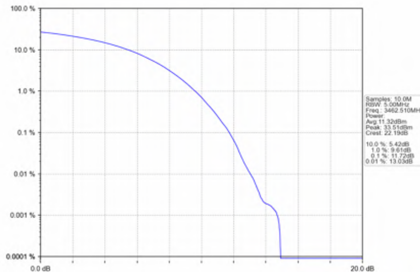
n78e_15kHz_SISO_NTNV_25MHz_CP-OFDM QPSK_3462.51MHz_Outer_Full
