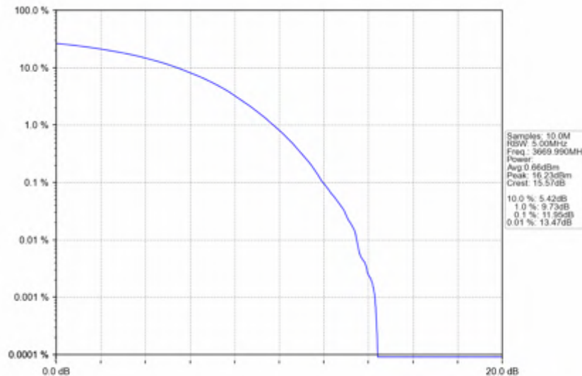
n78d_30kHz_SISO_NTNV_60MHz_CP-OFDM_QPSK_3669.99MHz_Outer_Full
