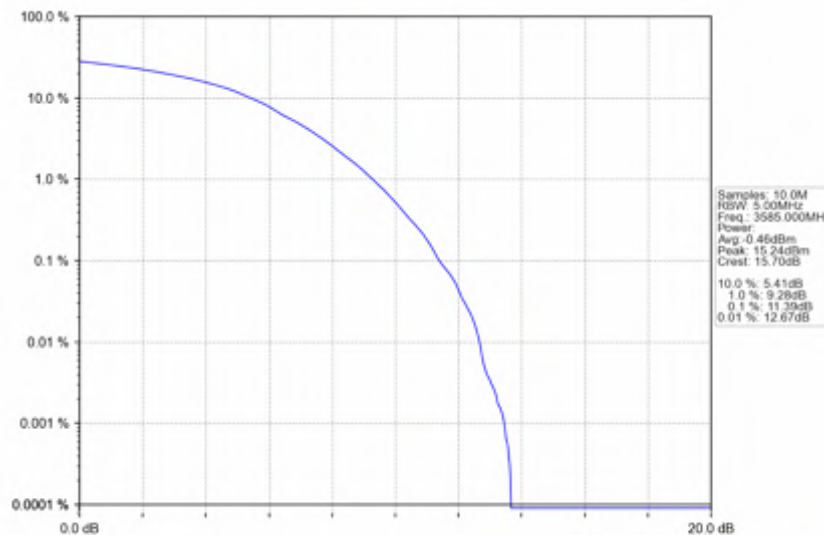
n78d_30kHz_SISO_NTNV_70MHz_DFT-s-OFDM_256_QAM_3585MHz_Outer_Full
