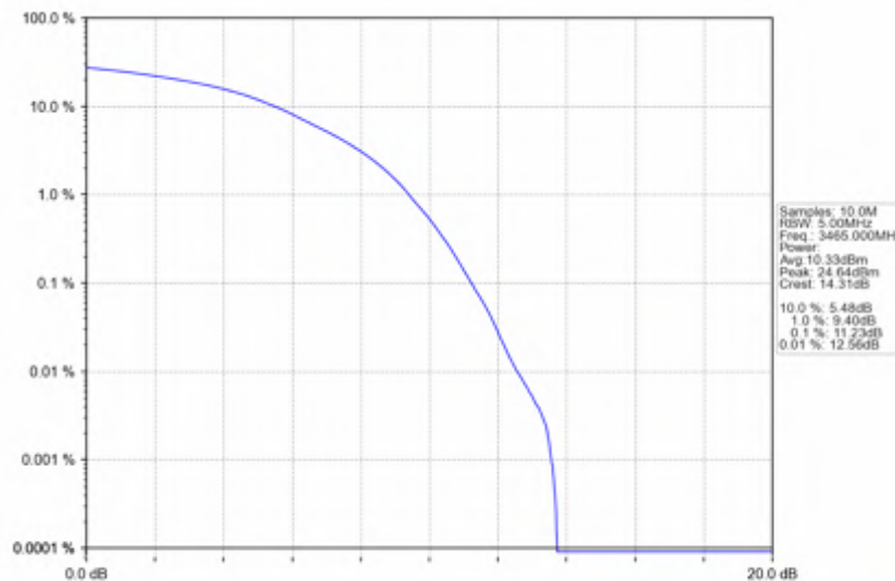
n78e_15kHz_SISO_NTV_30MHz_DFT-s-OFDM 64 QAM_3465MHz_Outer_Full
