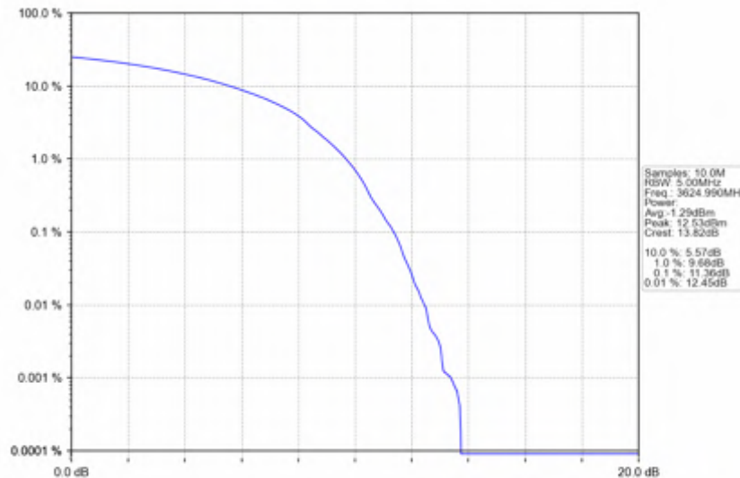
n78d_30kHz_SISO_NTNV_90MHz_DFT-s-OFDM_QPSK_3624.99MHz_Outer_Full
