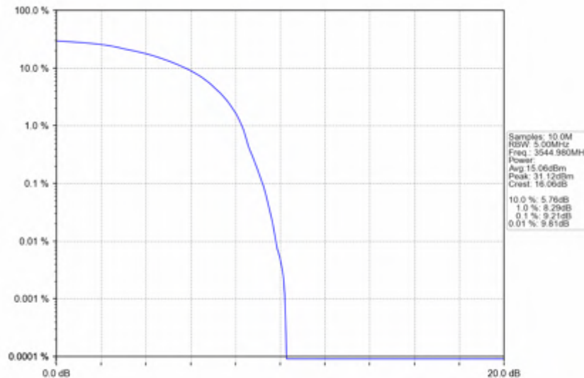
n78e_30kHz_SISO_NTNV_10MHz_DFT-s-OFDM_QPSK_3544.98MHz_Outer_Full
