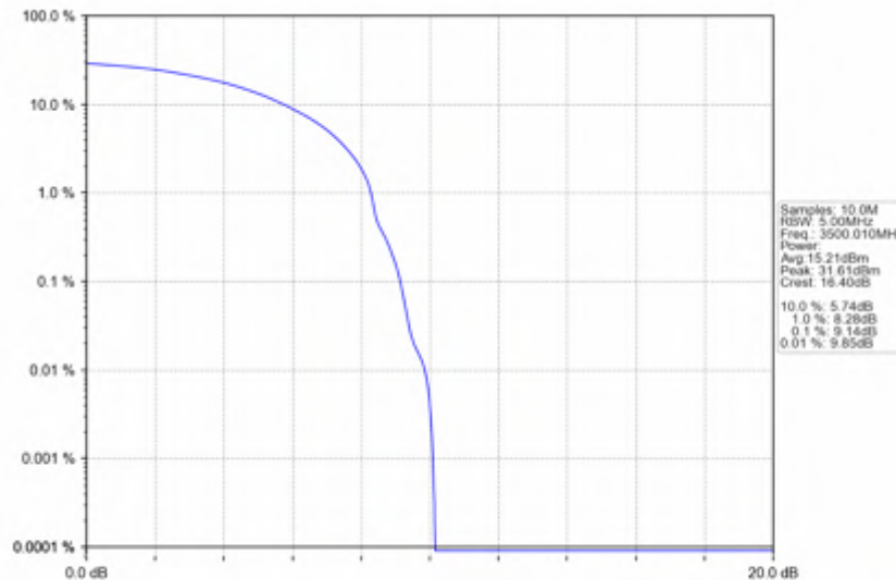
n78e_30kHz_SISO_NTNV_10MHz_DFT-s-OFDM_QPSK_3500.01MHz_Outer_Full
