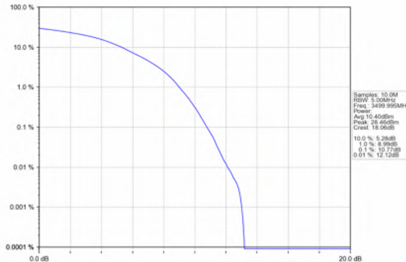
n78e_15kHz_SISO_NTNV_30MHz_DFT-s-OFDM 64 QAM_3499.995MHz_Outer_Full
