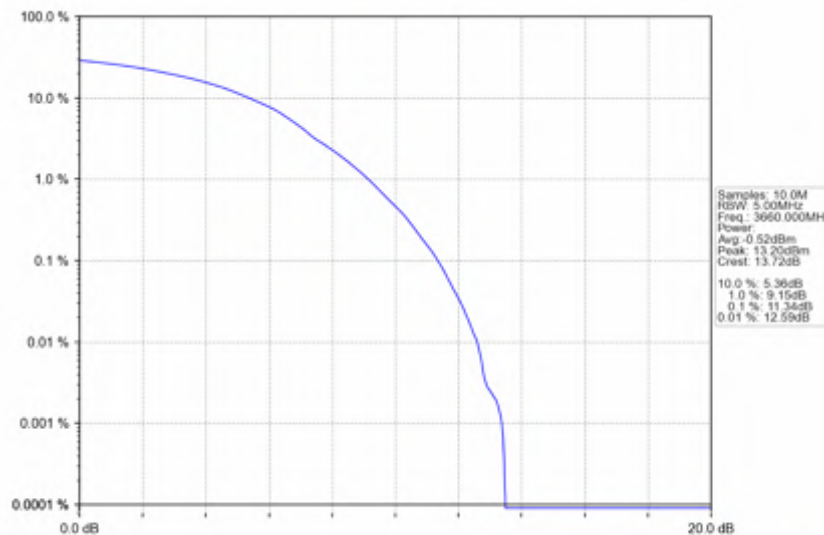
n78d_30kHz_SISO_NTV_80MHz_DFT-s-OFDM 64 QAM_3660MHz_Outer_Full
