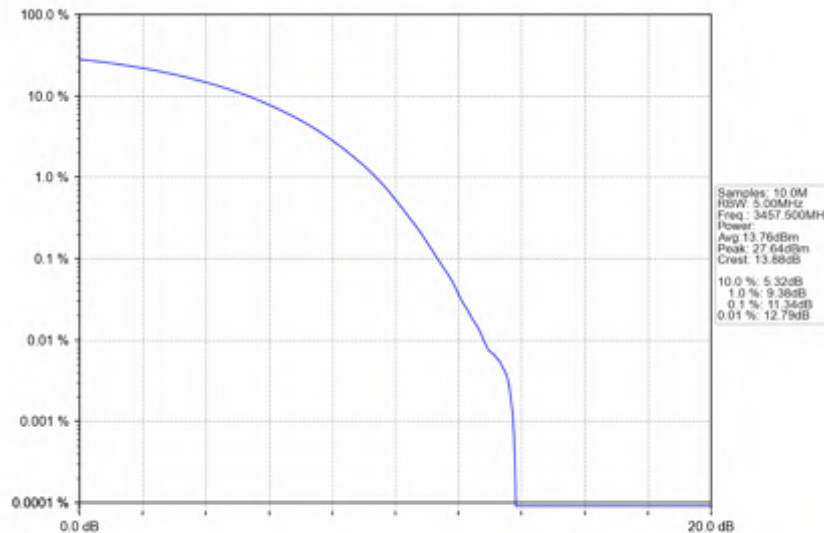
n78e_15kHz_SISO_NTNV_15MHz_CP-OFDM_QPSK_3457.5MHz_Outer_Full
