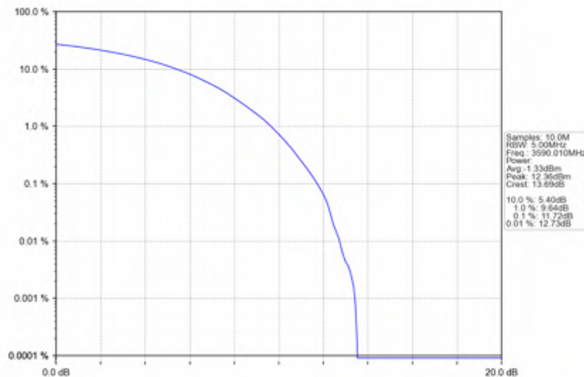
n78d_30kHz_SISO_NTNV_80MHz_CP-OFDM_256_QAM_3590.01MHz_Outer_Full
