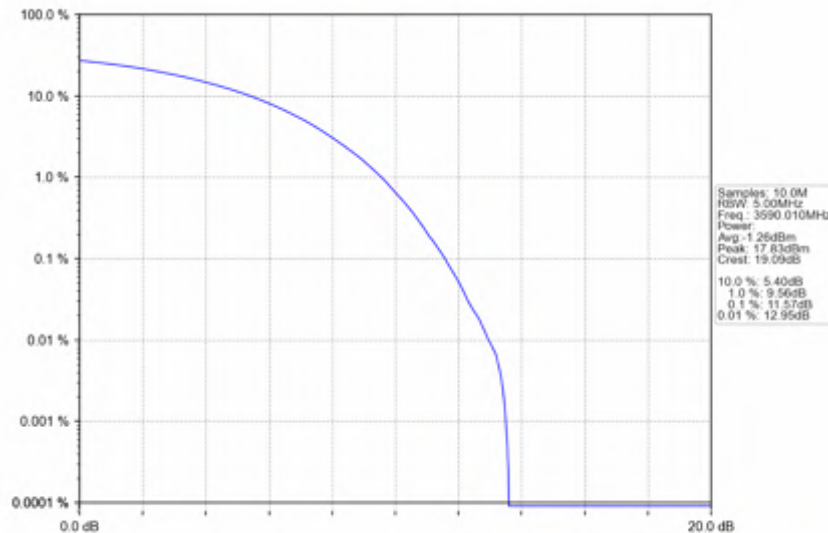
n78d_30kHz_SISO_NTNV_80MHz_CP-OFDM_QPSK_3590.01MHz_Outer_Full
