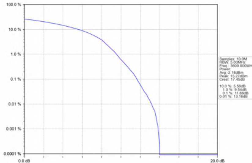
n78d_30kHz_SISO_NTNV_100MHz_DFT-s-OFDM 64 QAM_3600MHz_Outer_Full
