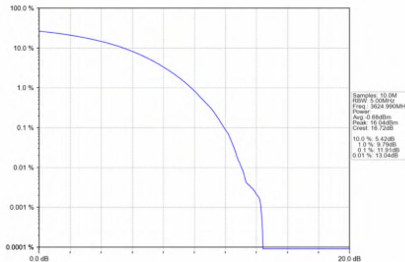
n78d_30kHz_SISO_NTNV_80MHz_CP-OFDM 64 QAM_3624.99MHz_Outer_Full
