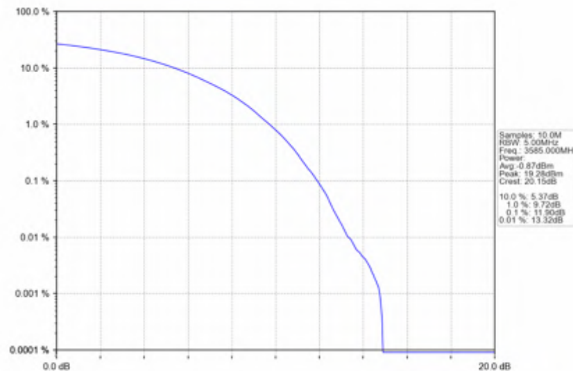
n78d_30kHz_SISO_NTNV_70MHz_CP-OFDM_16_QAM_3585MHz_Outer_Full
