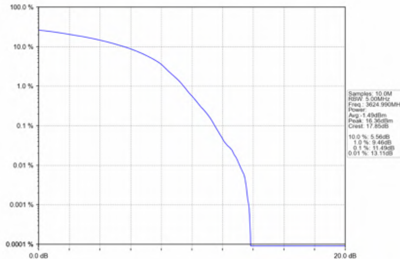
n78d_30kHz_SISO_NTNV_100MHz_DFT-s-OFDM_64_QAM_3624.99MHz_Outer_Full
