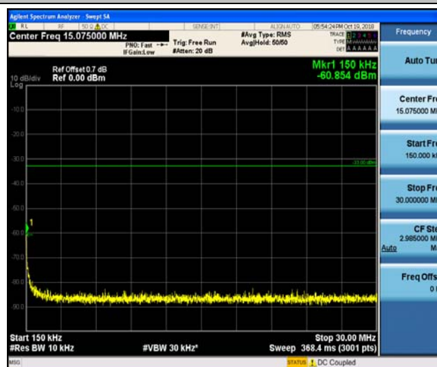
Band2_1.4MHz_16QAM_18607_1RB#0
