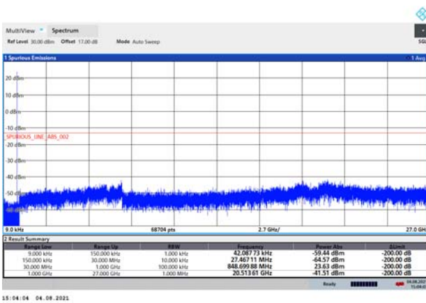
NB-IoT Band 5 CH-High 9kHz-27GHz
