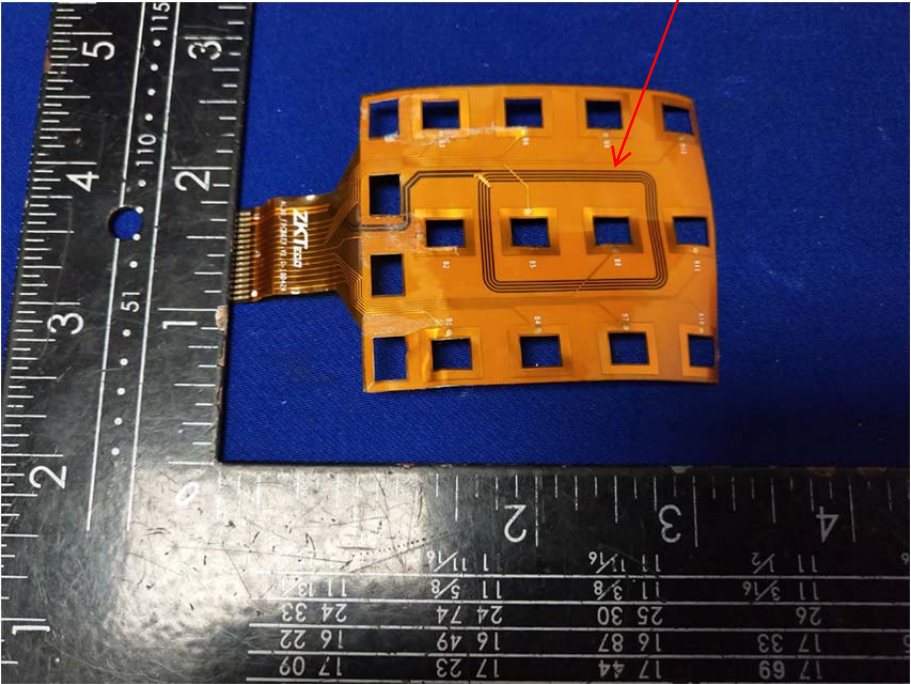
13.56MHz Antenna
