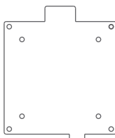
Bracket/ Screw
