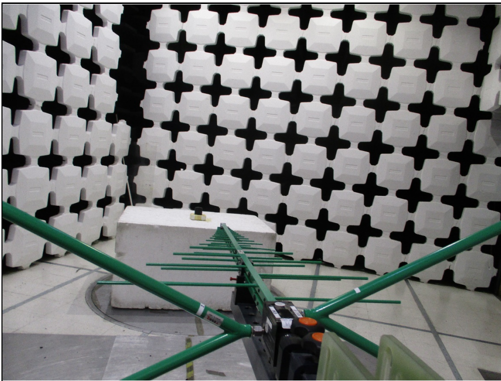
Test Setup for Spurious Radiated Emissions, 30-1000MHz – Antenna Polarization Horizontal
