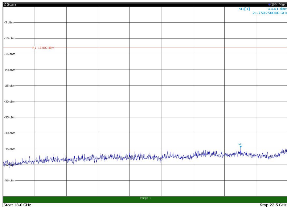
Channel: TOP, Modulation: 64QAM, BW=20MHz, Range: 18GHz - 22.5GHz, Polarization: Vertical
