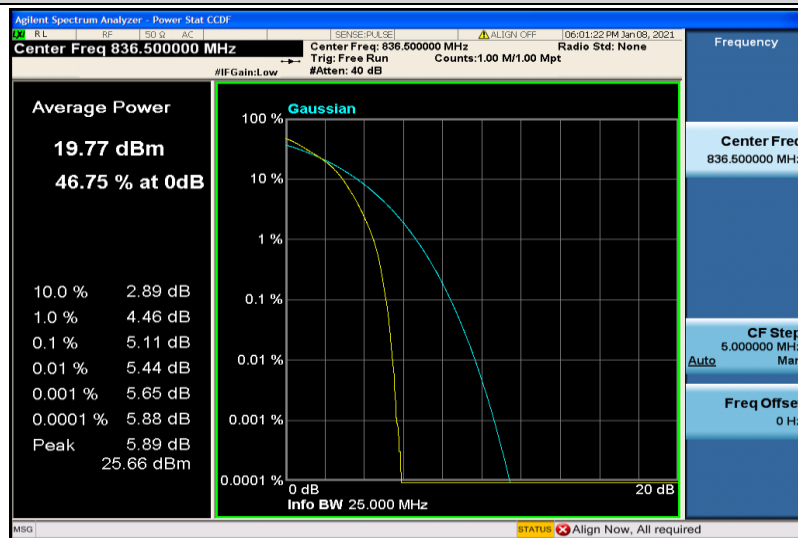
Band26-10MHz-16QAM-26915-50RB#0
