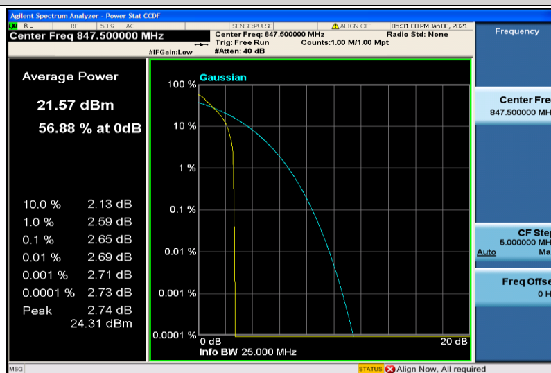
Band26-3MHz-QPSK-27025-1RB#0
