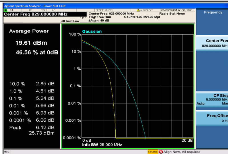
Band26-10MHz-16QAM-26840-50RB#0
