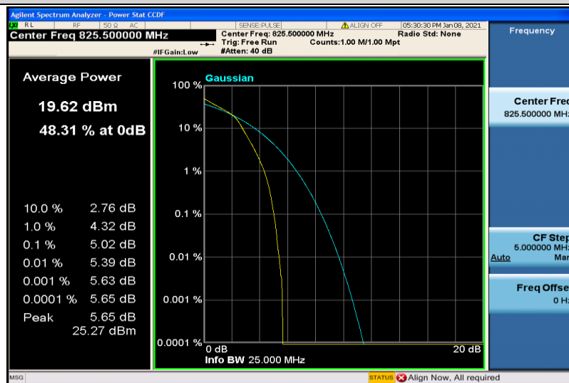
Band26-3MHz-16QAM-26805-15RB#0
