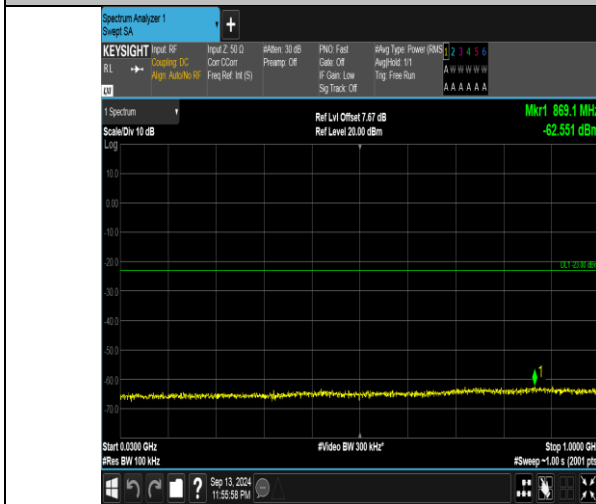
Band66_15MHz_QPSK_132047_1RB#0_30~1000_30~1000
