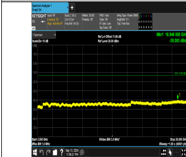
Band66_15MHz_QPSK_132047_1RB#0_3000~20000_3000~20000
