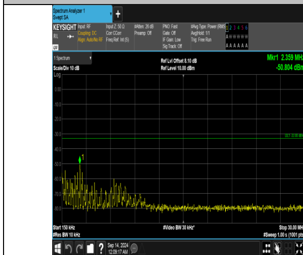
Band66_15MHz_16QAM_132597_1RB#74_0.15~30_0.15~30
