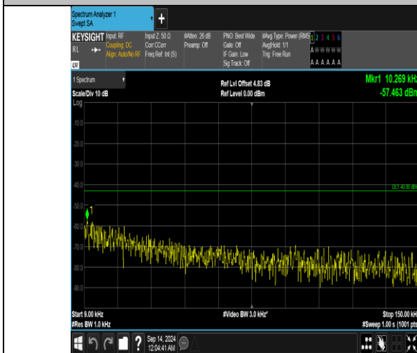
Band66_15MHz_QPSK_132322_75RB#0_0.009~0.15_0.009~0.15
