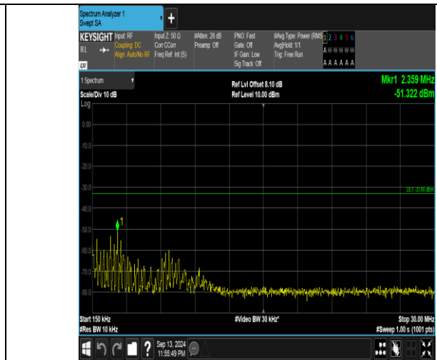
Band66_15MHz_QPSK_132047_1RB#0_0.15~30_0.15~30
