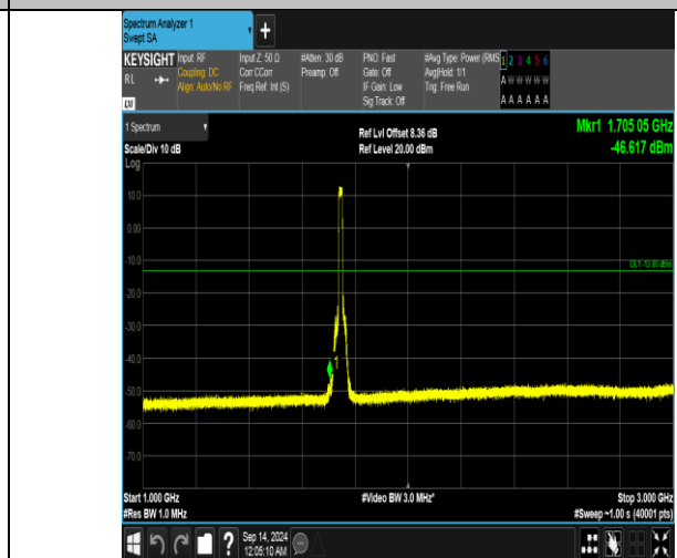
Band66_15MHz_QPSK_132322_75RB#0_1000~3000_1000~3000
