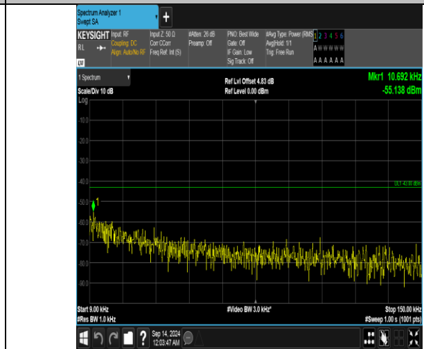
Band66_15MHz_16QAM_132322_1RB#74_0.009~0.15_0.009~0.15
