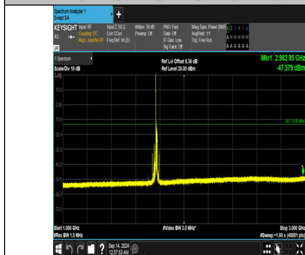
Band66 15MHz 16QAM 132597 1RB#0 1000~3000 1000~3000
