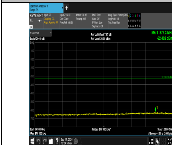
Band66_15MHz_QPSK_132322_75RB#0_30~1000_30~1000
