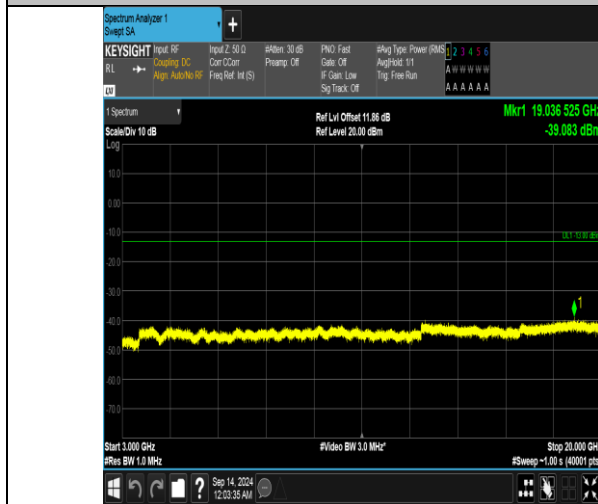
Band66_15MHz_QPSK_132322_1RB#74_3000~20000_3000~20000
