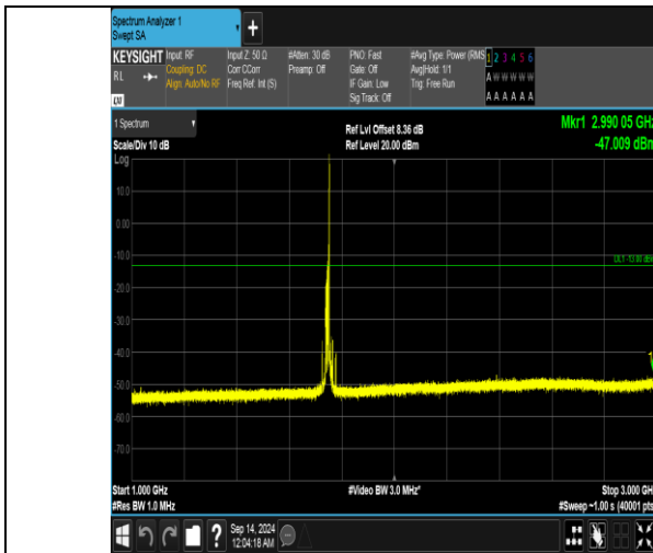
Band66_15MHz_16QAM_132322_1RB#74_1000~3000_1000~3000
