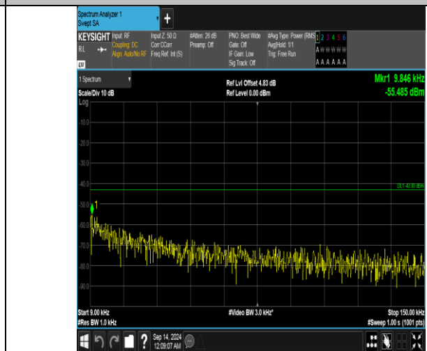
Band66_15MHz_16QAM_132597_1RB#74_0.009~0.15_0.009~0.15
