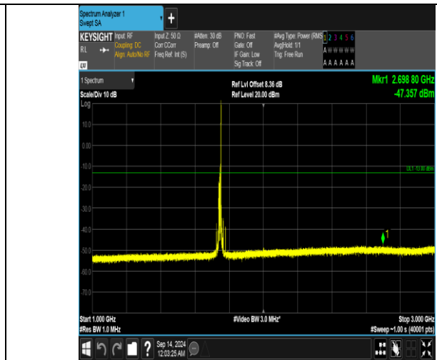
Band66_15MHz_QPSK_132322_1RB#74_1000~3000_1000~3000
