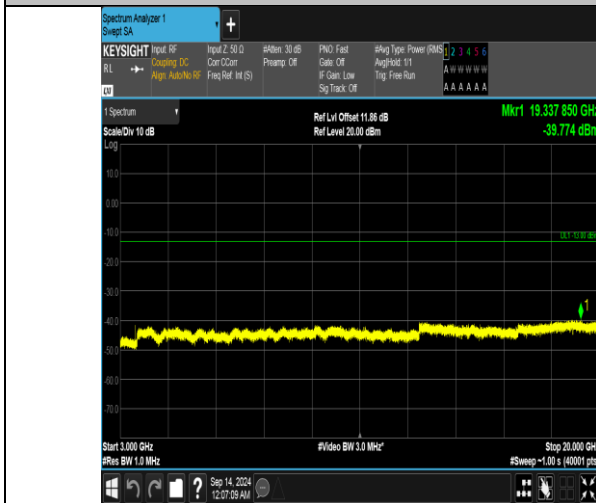
Band66_15MHz_QPSK_132597_1RB#0_3000~20000_3000~20000
