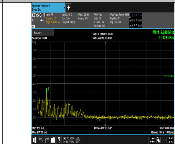
Band66_15MHz_QPSK_132047_75RB#0_0.15~30_0.15~30
