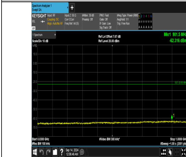
Band66_15MHz_QPSK_132597_1RB#0_30~1000_30~1000
