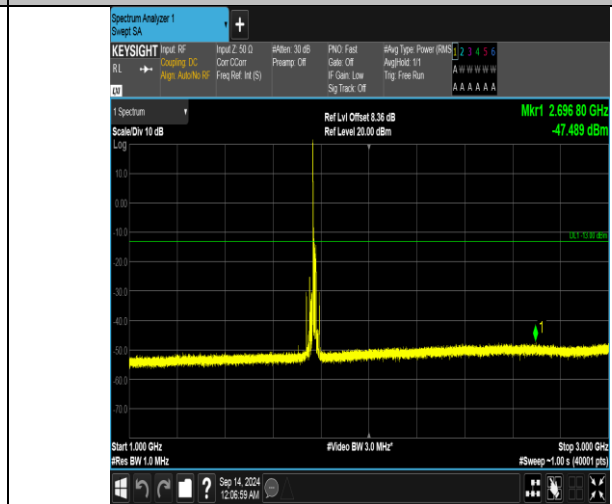
Band66_15MHz_QPSK_132597_1RB#0_1000~3000_1000~3000
