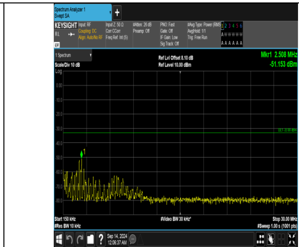
Band66_15MHz_QPSK_132597_1RB#0_0.15~30_0.15~30
