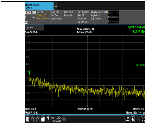
Band66_15MHz_QPSK_132597_1RB#0_0.009~0.15_0.009~0.15
