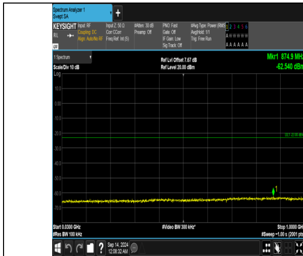
Band66_15MHz_QPSK_132597_1RB#74_30~1000_30~1000
