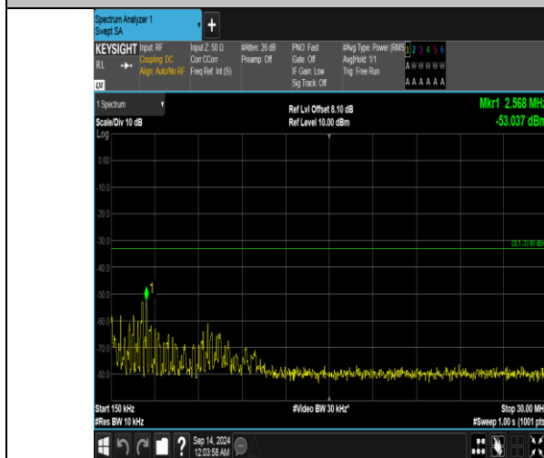
Band66_15MHz_16QAM_132322_1RB#74_0.15~30_0.15~30
