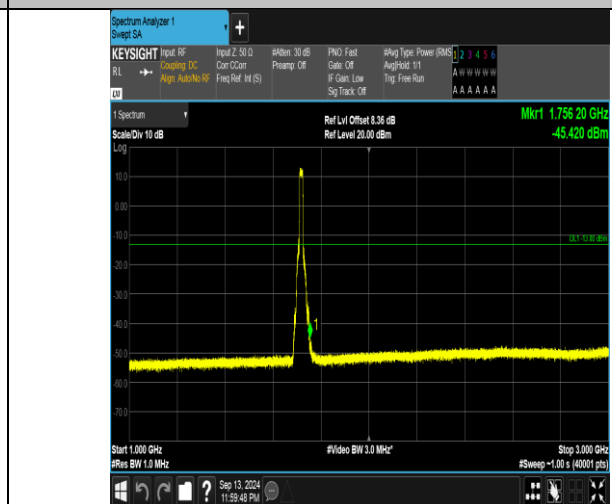
Band66_15MHz_QPSK_132047_75RB#0_1000~3000_1000~3000
