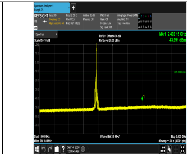
Band66_15MHz_QPSK_132597_1RB#74_1000~3000_1000~3000
