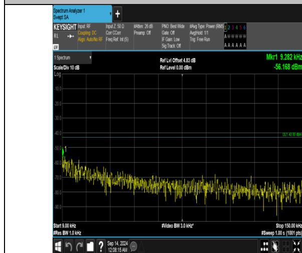
Band66 15MHz QPSK 132597 1RB#74 0.009~0.15 0.009~0.15
