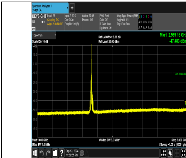
Band66_15MHz_16QAM_132047_1RB#74_1000~3000_1000~3000
