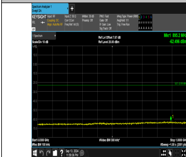
Band66_15MHz_QPSK_132047_75RB#0_30~1000_30~1000
