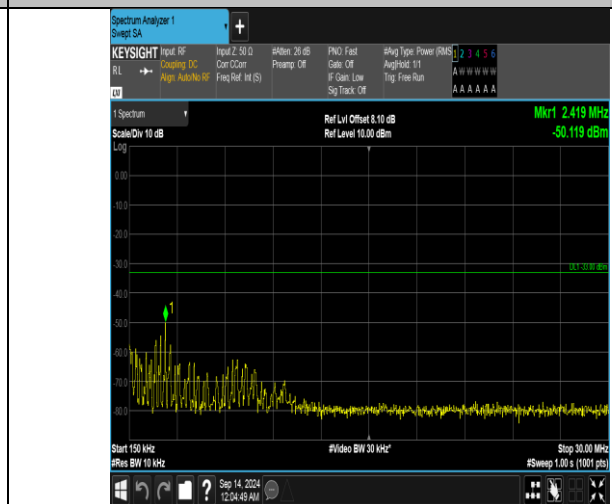
Band66_15MHz_QPSK_132322_75RB#0_0.15~30_0.15~30
