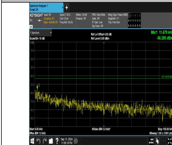
Band66_15MHz_QPSK_132047_75RB#0_0.009~0.15_0.009~0.15
