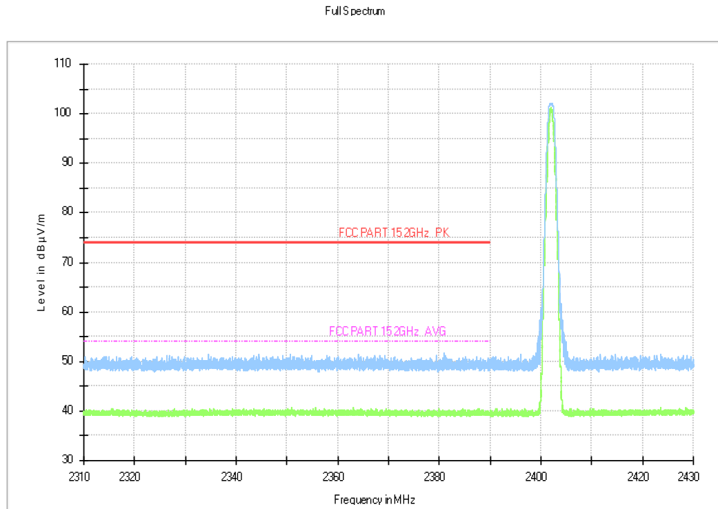
Fig.18. Frequency Band Edges: GFSK, 2402 MHz, Hopping Off, 2.31 GHz – 2.43GHz
