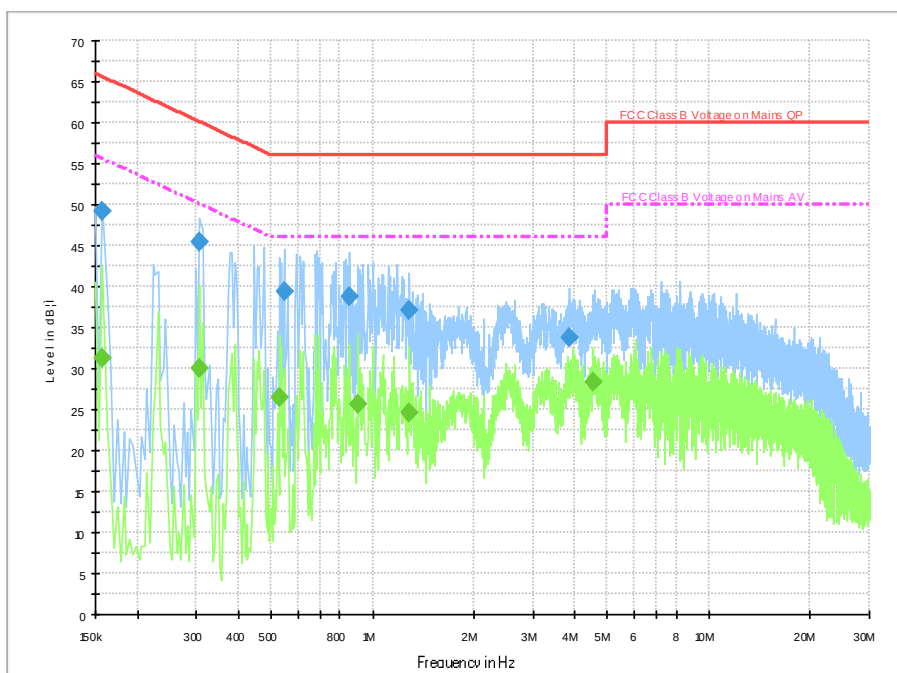
Fig.B.8.1 AC Powerline Conducted Emission-blutetooth
