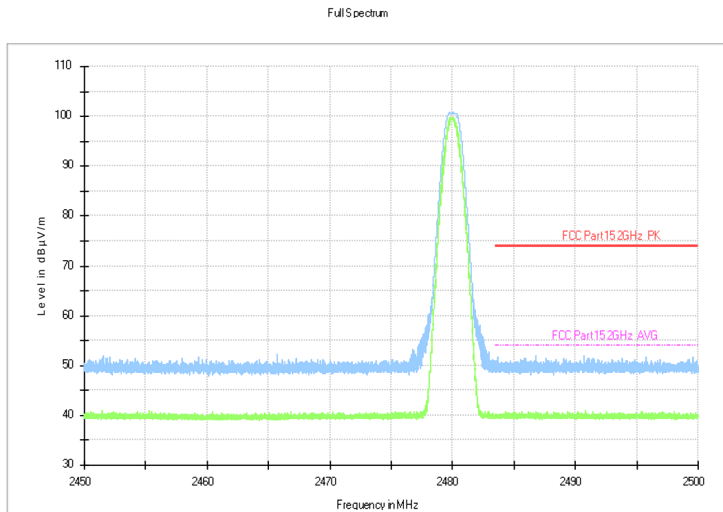
Fig.19. Frequency Band Edges: GFSK, 2480 MHz, Hopping Off, 2.45 GHz - 2.50GHz
