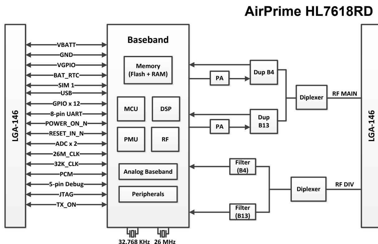
Figure 1. Architecture Overview
