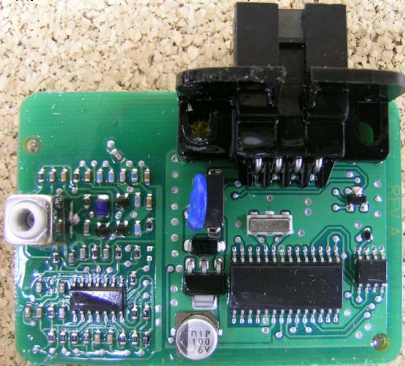
PCB (top)
