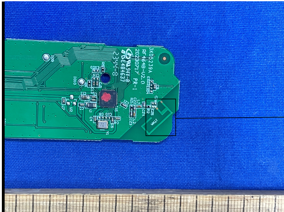
PCB Antenna
