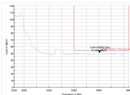
802.11a-Channel 48: Average
