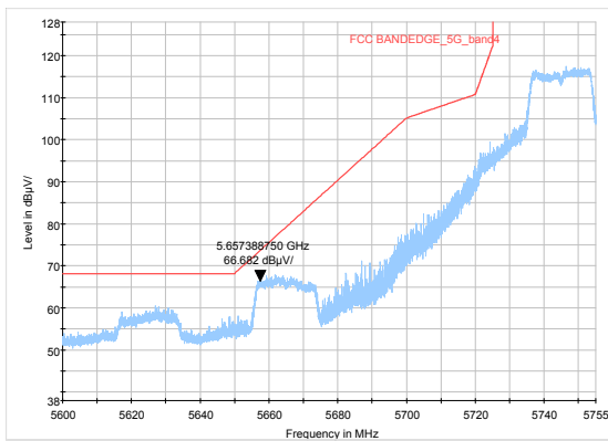
802.11a-Channel 149: Peak
