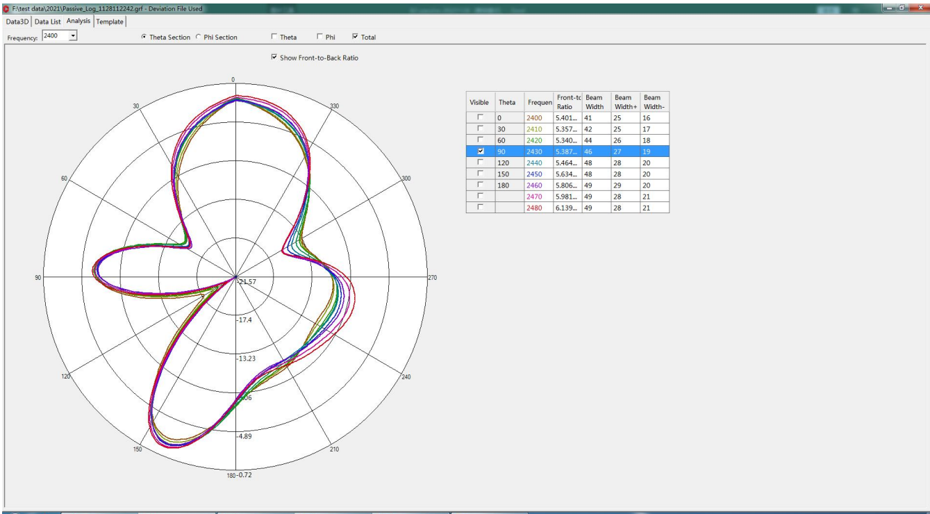
2D辐射图(2D radiation chart) Theta 90°
