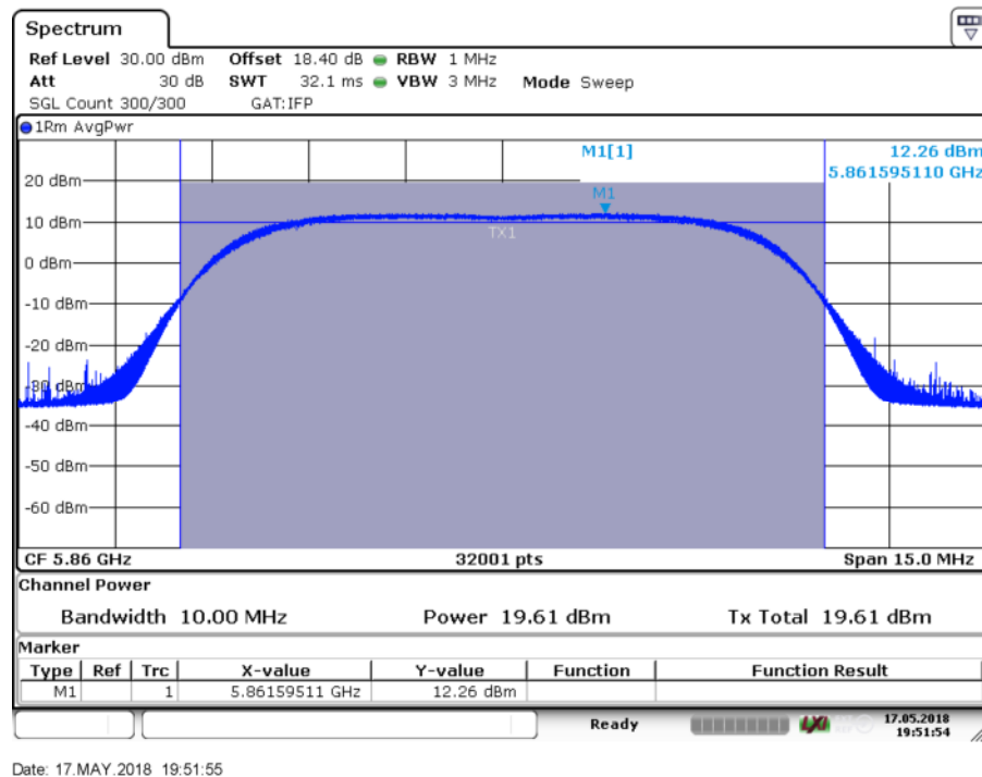
Antenna 2, Ch. 172
