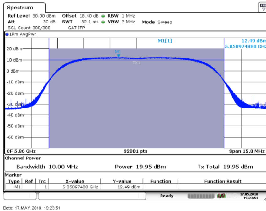
Antenna 1, Ch. 172
