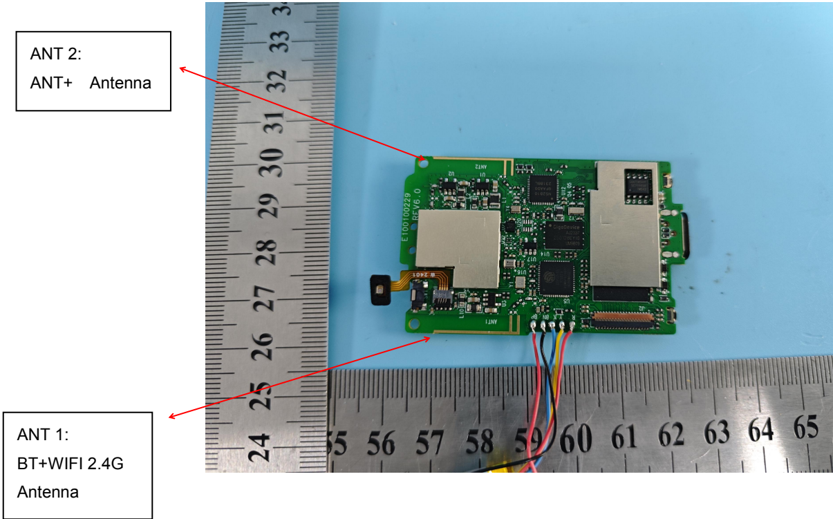
INTERNAL PHOTO OF SAMPLE PCB
