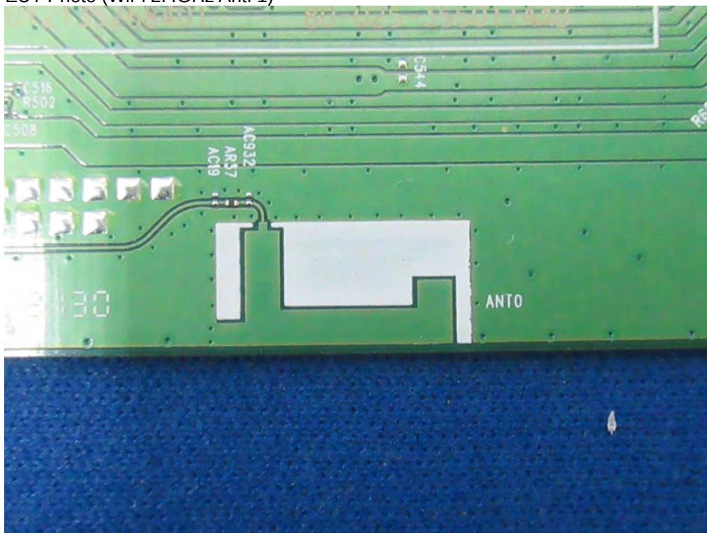
(16) EUT Photo (WiFi 2.4GHz Ant. 1)
