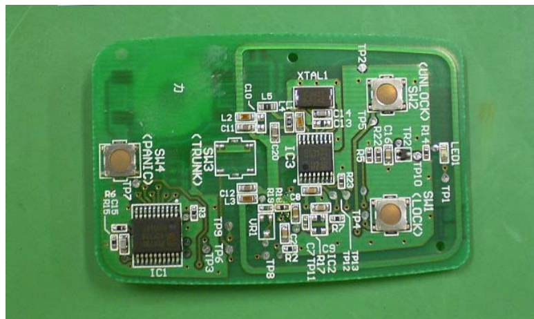
Figure 8.12 G8D-640M-KEY-N PCB assy (back view)
