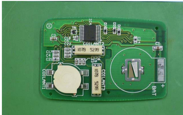
Figure 8.11 G8D-640M-KEY-N PCB assy (front view)
