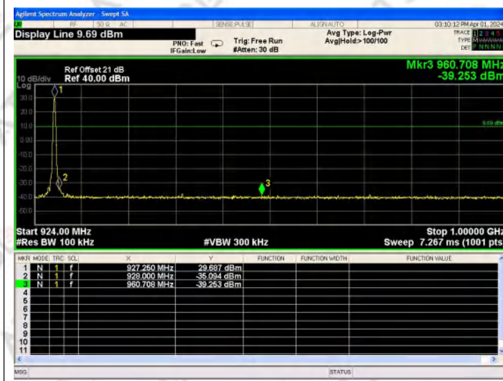
CH50 bandedge
