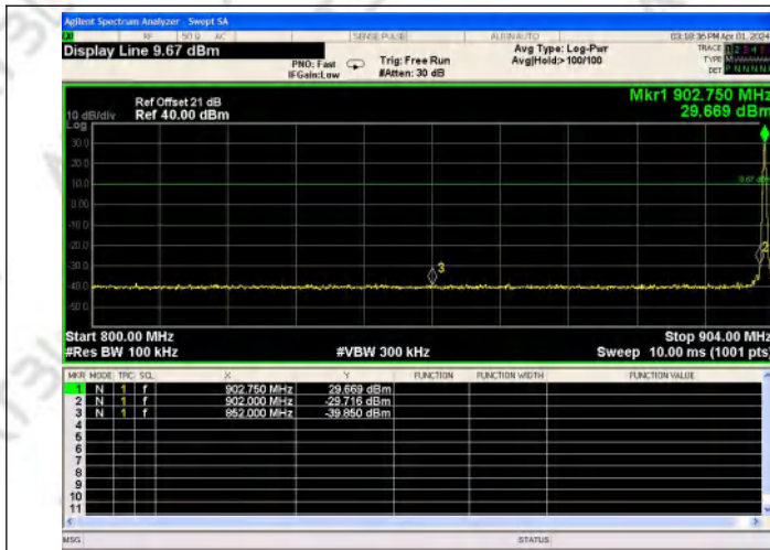
CH0 bandedge
