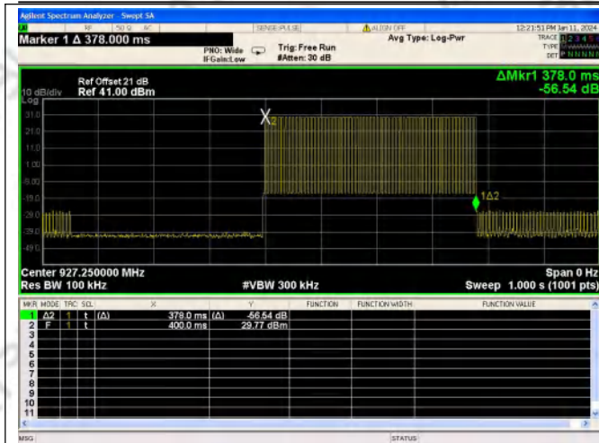
Dense reader CH50 Single pulse
