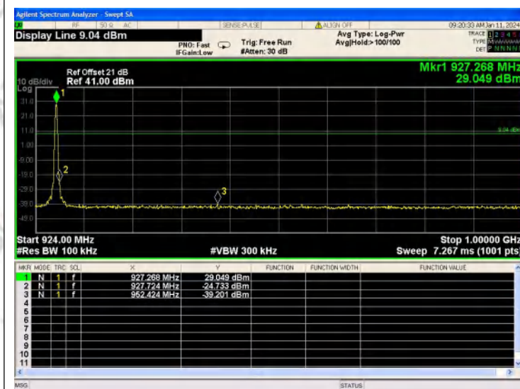
CH50 bandedge
