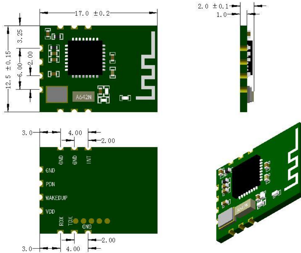
Fig4. Module Size Diagram
