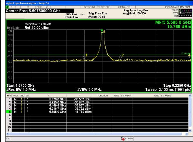
Out Of Band Emission IEEE 802.11n_Channel 120_20MHz_Antenna 0
