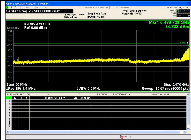
Spurious Emission:30.0~5470 MHz IEEE 802.11n_Channel 100_20MHz_Antenna 0
