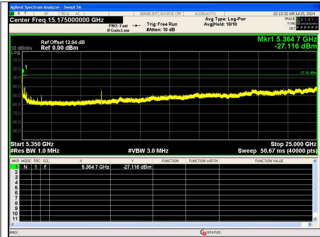
Spurious Emission:5350~25000.0 MHz IEEE 802.11n_Channel 64_20MHz_Antenna 0
