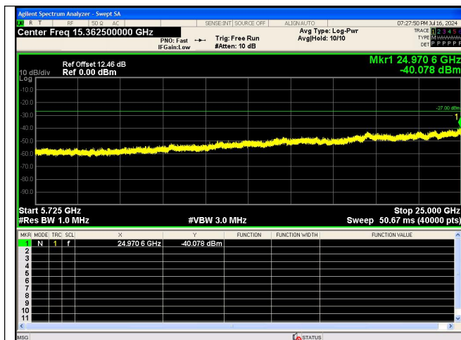
Spurious Emission:5725~25000.0 MHz IEEE 802.11a_Channel 140_20MHz_Antenna 0
