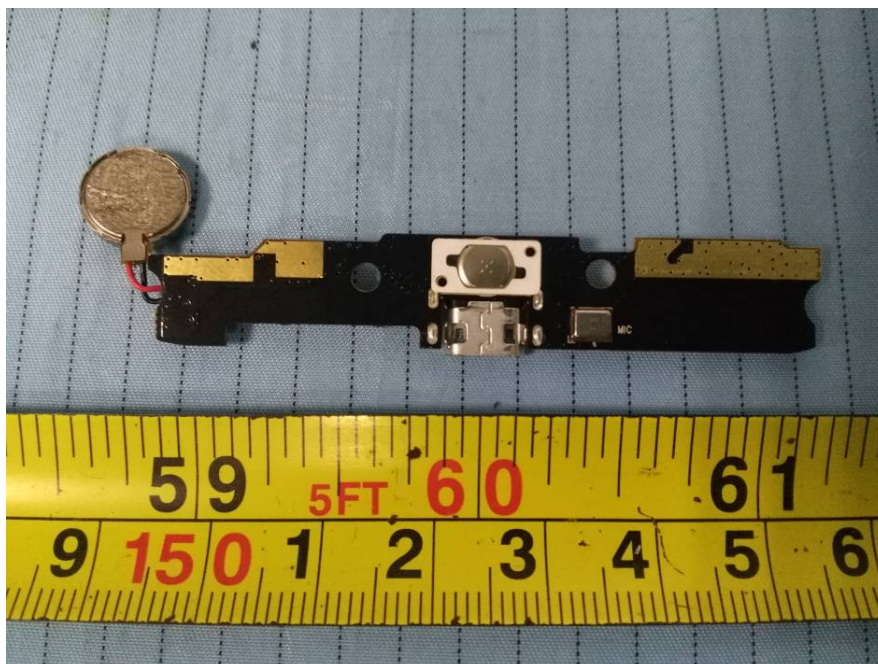
EUT – USB Mainboard Bottom View
