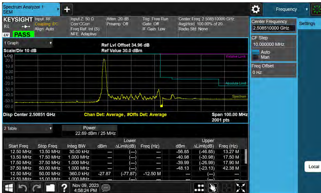
Sub6 n41. Low Channel Edge Plot (25 MHz Ch.501702 BPSK_RB 1)-2
