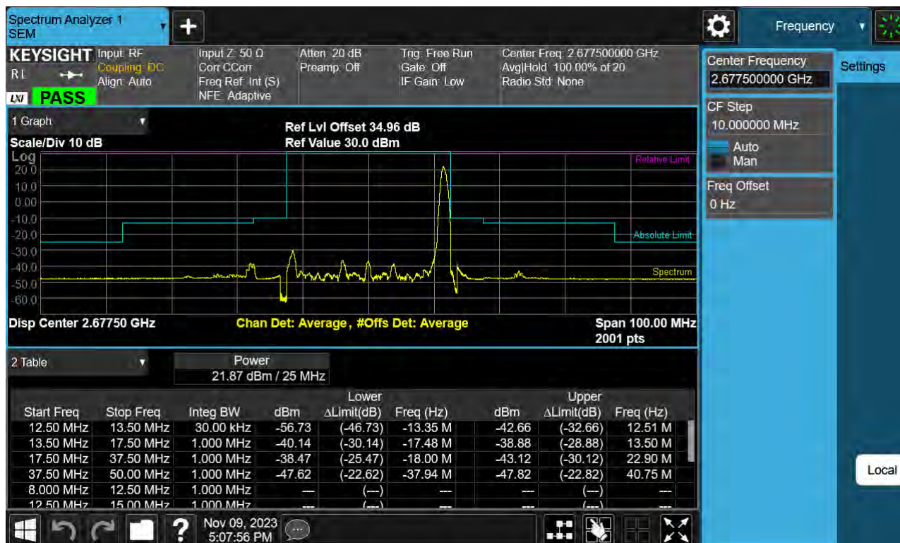
Sub6 n41. High Channel Edge Plot (25 MHz Ch.535500 BPSK RB 1)
