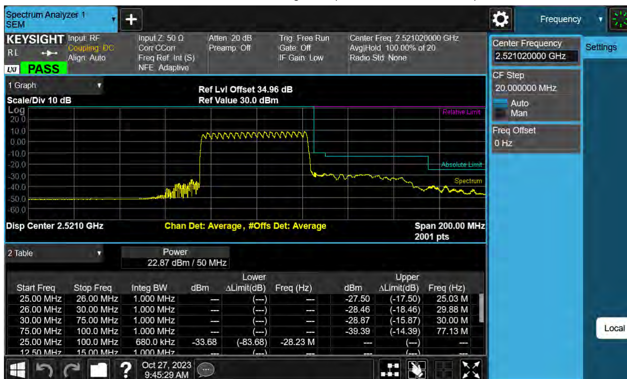
Sub6 n41. Low Channel Edge Plot (50 MHz Ch.504204 BPSK)-2
