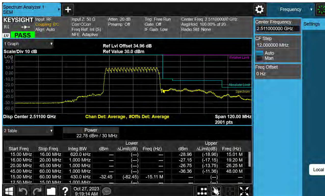
Sub6 n41. Low Channel Edge Plot (30 MHz Ch.502200 BPSK)-2
