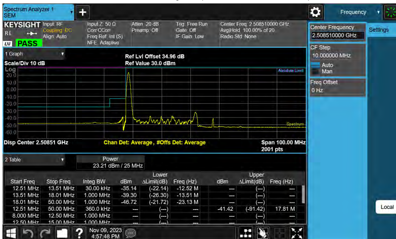
Sub6 n41. Low Channel Edge Plot (25 MHz Ch.501702 BPSK RB 1)-1
