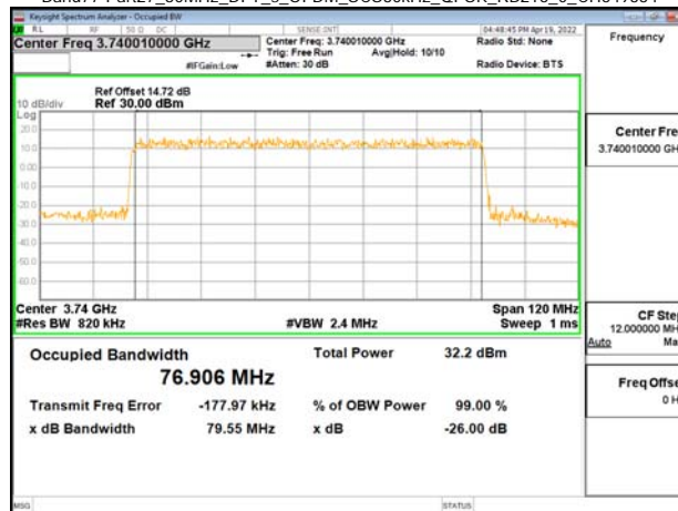
Band77-Part27_80MHz_DFT_s_OFDM_SCS30kHz_QPSK_RB216_0_CH649334
