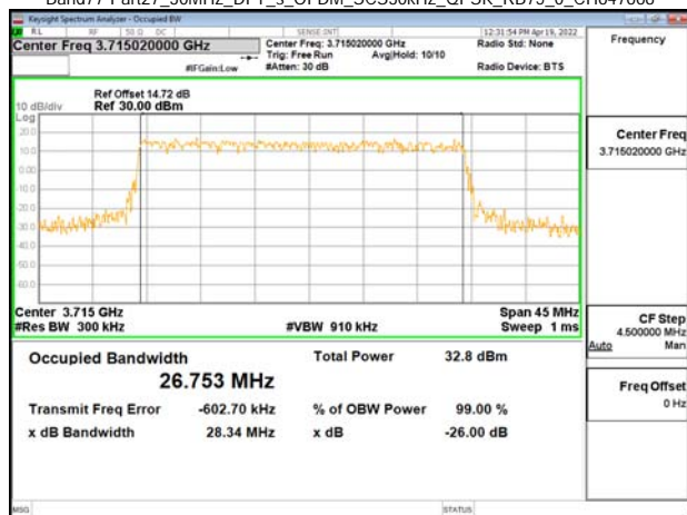
Band77-Part27_30MHz_DFT_s_OFDM_SCS30kHz_QPSK_RB75_0_CH647668
