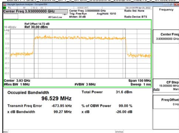
Band77-Part27_100MHz_DFT_s_OFDM_SCS30kHz_256QAM_RB270_0_CH662000
