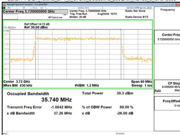
Band77-Part27_40MHz_DFT_s_OFDM_SCS30kHz_256QAM_RB100_0_CH648000
