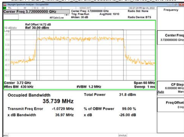
Band77-Part27_40MHz_DFT_s_OFDM_SCS30kHz_BPSK_RB100_0_CH648000
