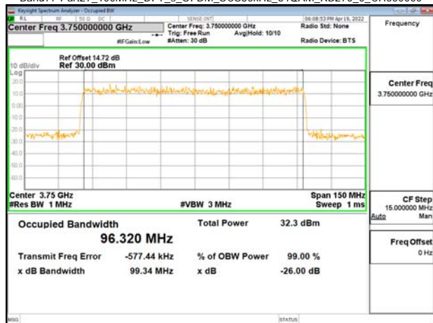
Band77-Part27_100MHz_DFT_s_OFDM_SCS30kHz_64QAM_RB270_0_CH650000
