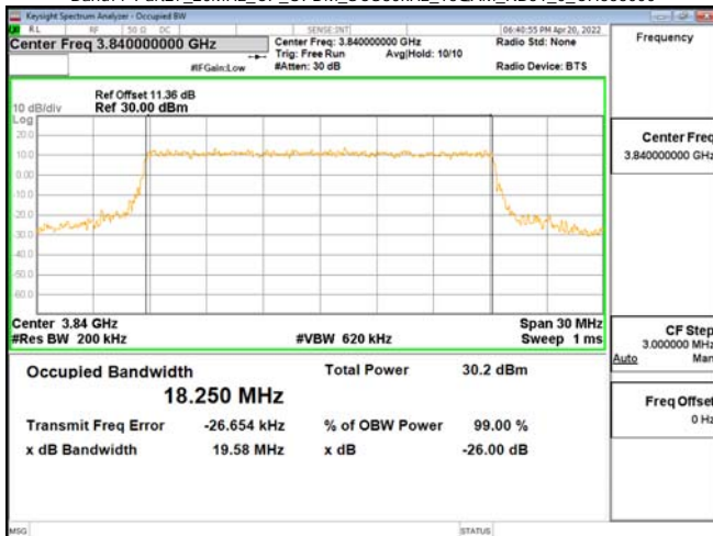
Band77-Part27_20MHz_CP_OFDM_SCS30kHz_16QAM_RB51_0_CH656000
