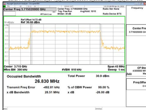
Band77-Part27_30MHz_DFT_s_OFDM_SCS30kHz_256QAM_RB75_0_CH647668
