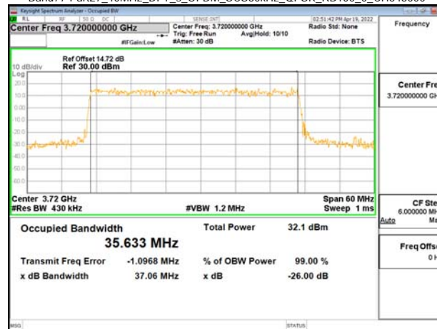
Band77-Part27_40MHz_DFT_s_OFDM_SCS30kHz_QPSK_RB100_0_CH648000
