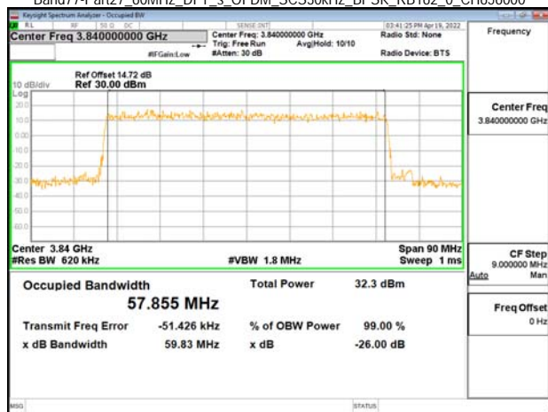
Band77-Part27_60MHz_DFT_s_OFDM_SCS30kHz_BPSK_RB162_0_CH663332
