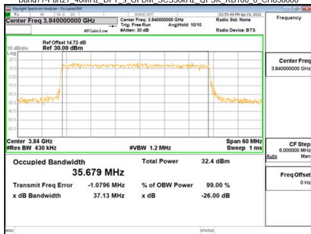
Band77-Part27_40MHz_DFT_s_OFDM_SCS30kHz_QPSK_RB100_0_CH646000
