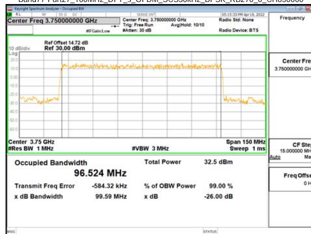
Band77-Part27_100MHz_DFT_s_OFDM_SCS30kHz_BPSK_RB270_0_CH650000
