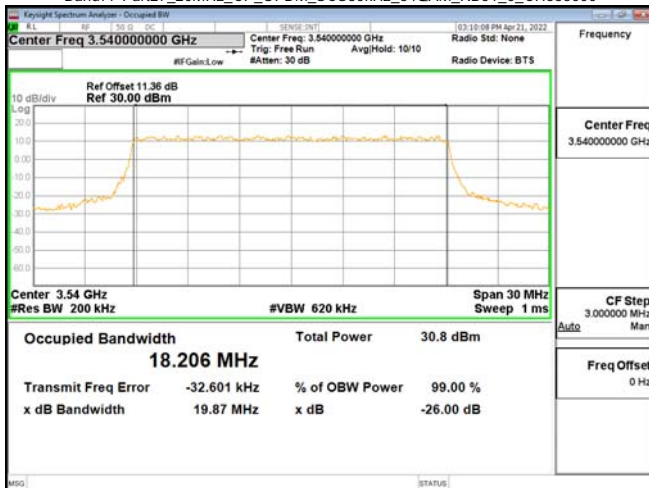
Band77-Part27_20MHz_CP_OFDM_SCS30kHz_64QAM_RB51_0_CH636000
