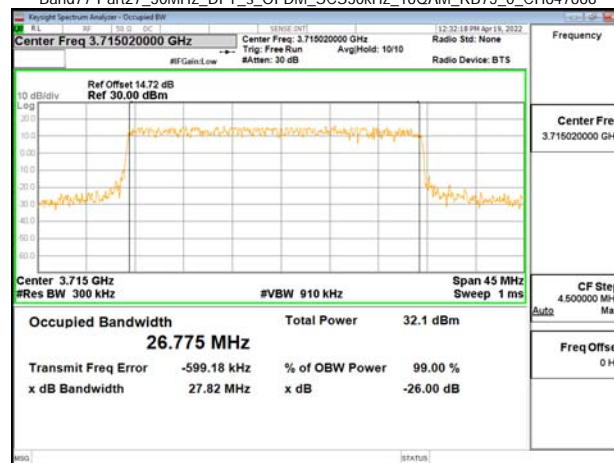
Band77-Part27_30MHz_DFT_s_OFDM_SCS30kHz_16QAM_RB75_0_CH647668
