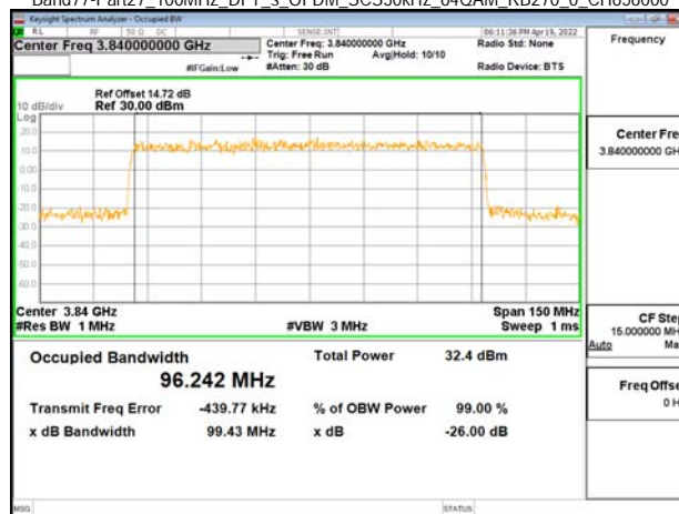
Band77-Part27_100MHz_DFT_s_OFDM_SCS30kHz_64QAM_RB270_0_CH656000
