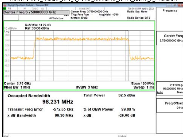
Band77-Part27_100MHz_DFT_s_OFDM_SCS30kHz_QPSK_RB270_0_CH650000
