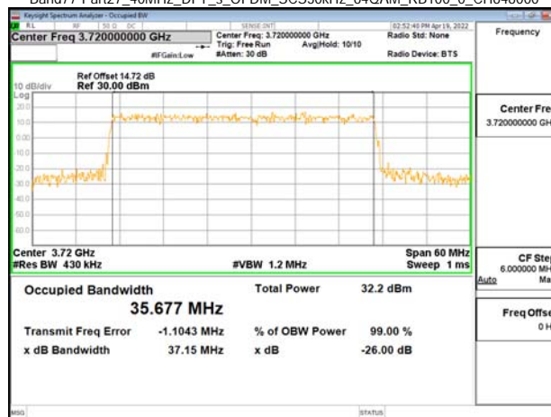
Band77-Part27_40MHz_DFT_s_OFDM_SCS30kHz_64QAM_RB100_0_CH648000
