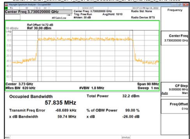
Band77-Part27_60MHz_DFT_s_OFDM_SCS30kHz_BPSK_RB162_0_CH648668
