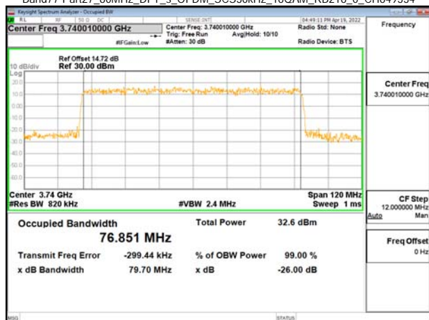
Band77-Part27_80MHz_DFT_s_OFDM_SCS30kHz_16QAM_RB216_0_CH649334
