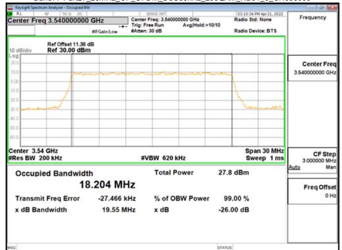
Band77-Part27_20MHz_CP_OFDM_SCS30kHz_256QAM_RB51_0_CH636000
