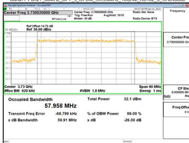
Band77-Part27_60MHz_DFT_s_OFDM_SCS30kHz_16QAM_RB162_0_CH648668
