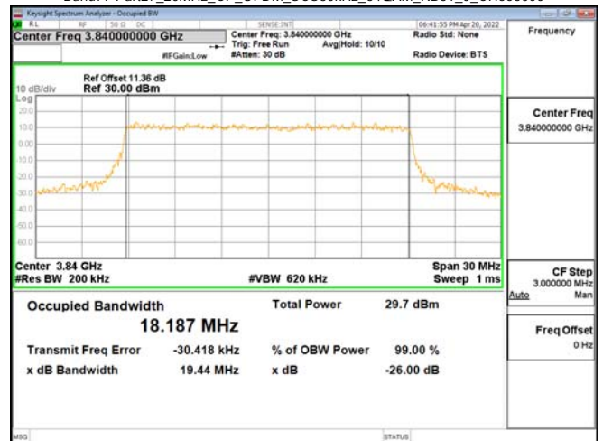
Band77-Part27_20MHz_CP_OFDM_SCS30kHz_64QAM_RB51_0_CH656000
