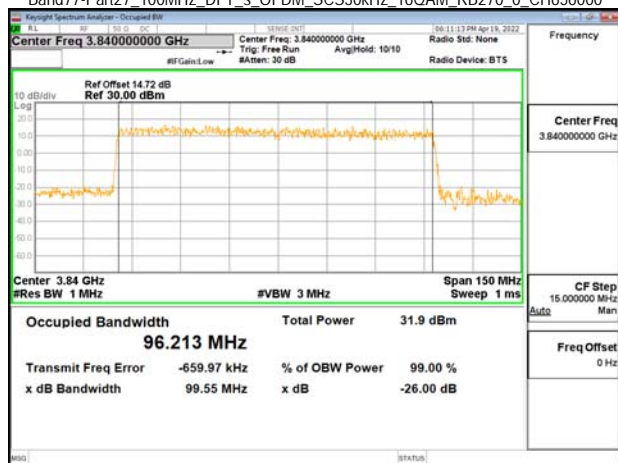
Band77-Part27_100MHz_DFT_s_OFDM_SCS30kHz_16QAM_RB270_0_CH656000
