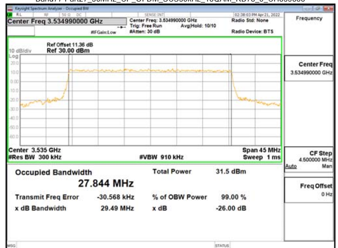
Band77-Part27_30MHz_CP_OFDM_SCS30kHz_16QAM_RB78_0_CH635666
