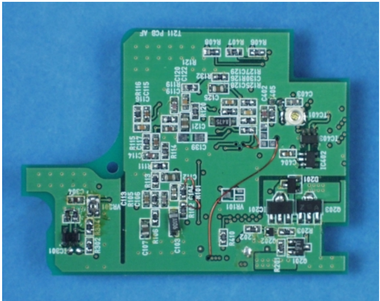
Sub PCB – Track Side
