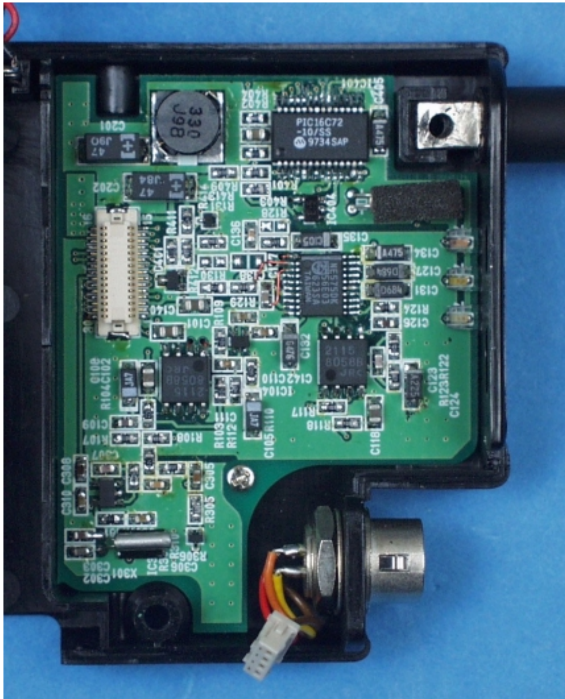
Sub PCB – Component Side
