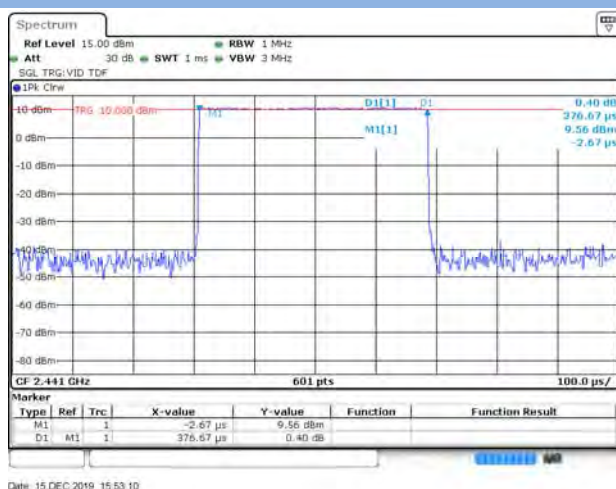
GFSK DH1
