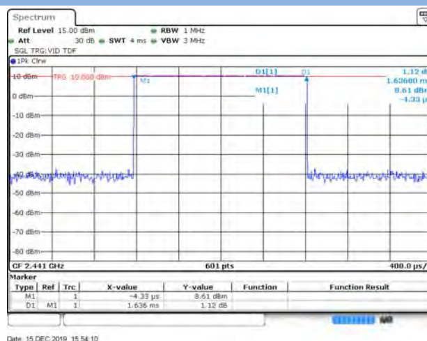
GFSK DH3
