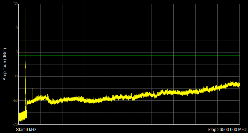
Band5 16QAM BW=5MHz Channel=20425 RB Size=1 Position=#0
