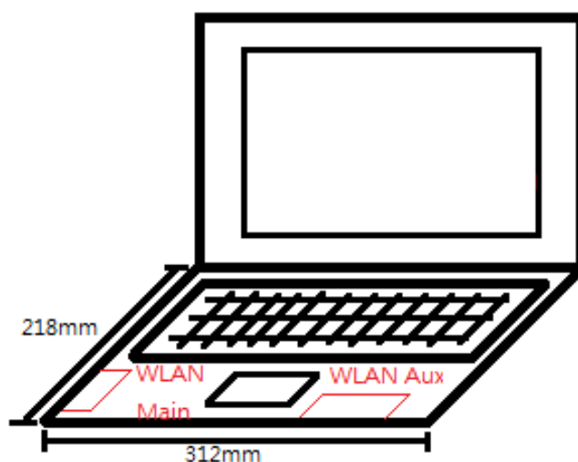
Photograph 15. Antenna position of EUT (Notebook mode)
