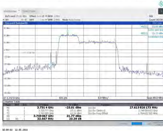
43-43-10MHz-20MHz-QPSK-QPSK-44996-45140-50RB#0-100RB#0
