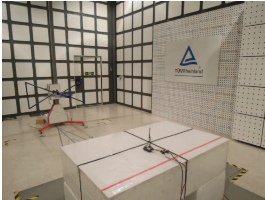
Photograph 3: Set-up for Spurious Emissions (Front View 2)- RFA-02-5-C7H1-ANT
