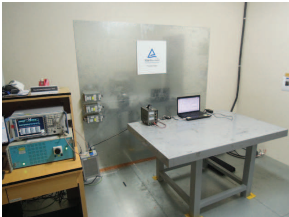
Photograph 27: Set-up for Mains Conducted testing (Front View)
