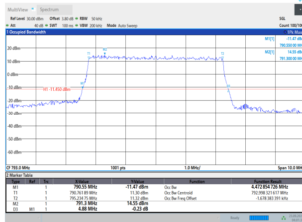
Band14-5MHz-QPSK-23330-25RB#0
