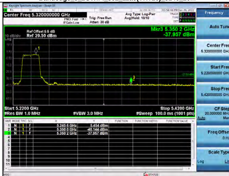
Bandedge_5_2GWiFi_802_11ac(VHT20)_5240_20M
