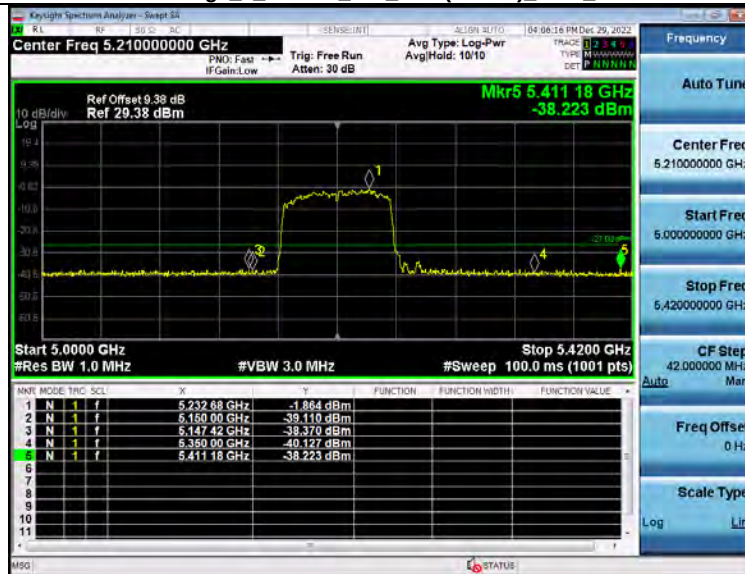
Bandedge_5_2GWiFi_802_11ac(VHT80) 5210_80M
