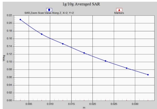
Fig.A.1- 19 Z-Scan at power reference point (LTE band71)
