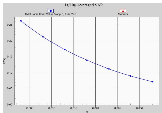
Fig.A.1- 20 Z-Scan at power reference point (LTE band71)
