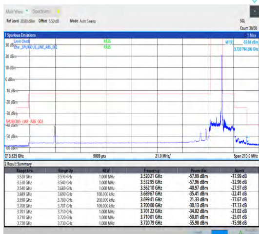
Band43_10MHz_QPSK_44540_1RB#49
