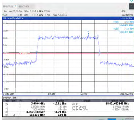
Band43-20MHz-16QAM-44090-100RB#0-PASS
