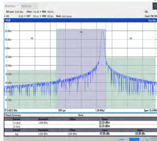
43(3600-3700)-5MHz-QPSK-43615-1RB#24-PASS
