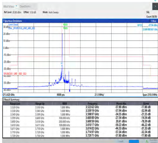
Band43_10MHz_QPSK_43640_1RB#0
