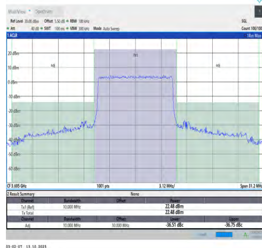
43(3600-3700)-10MHz-QPSK-44540-50RB#0-PASS
