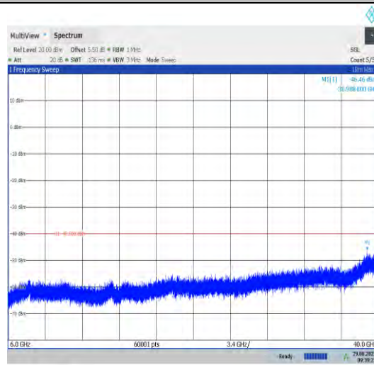
Band43_20MHz_QPSK_44090_1RB#0_6000~40000_6000~40000
