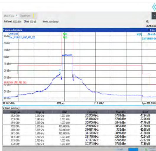
Band43_15MHz_QPSK_43665_75RB#0
