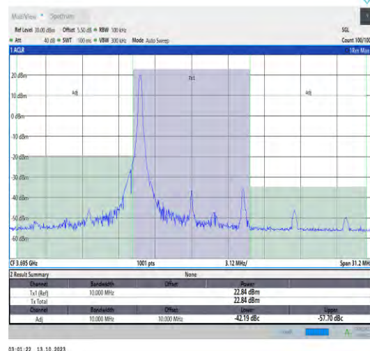
43(3600-3700)-10MHz-QPSK-44540-1RB#0-PASS
