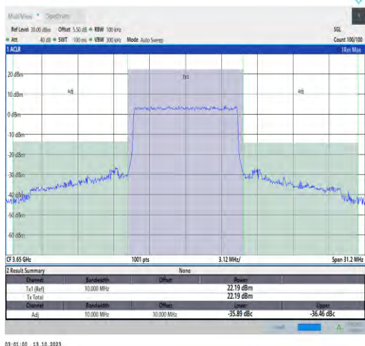
43(3600-3700)-10MHz-QPSK-44090-50RB#0-PASS
