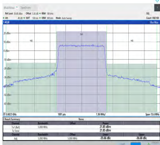
43(3600-3700)-5MHz-QPSK-43615-25RB#0-PASS
