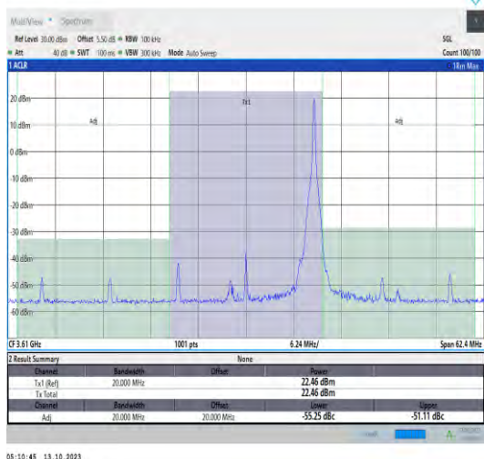
43(3600-3700)-20MHz-QPSK-43690-1RB#99-PASS
