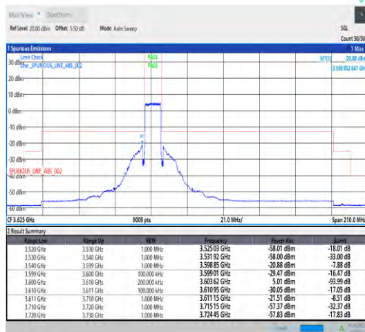
Band43_10MHz_QPSK_43640_50RB#0
