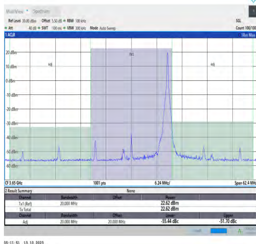
43(3600-3700)-20MHz-QPSK-44090-1RB#99-PASS
