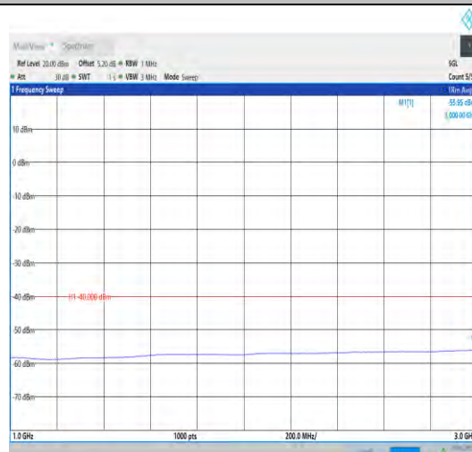
Band43_20MHz_QPSK_43690_1RB#0_1000~3000_1000 ~3000
