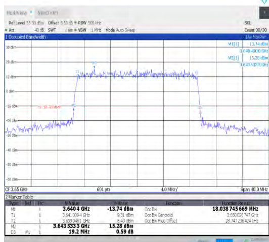
Band43-20MHz-QPSK-44090-100RB#0-PASS
