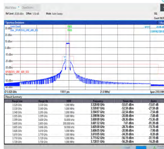
Band43 5MHz QPSK 43615 25RB#0
