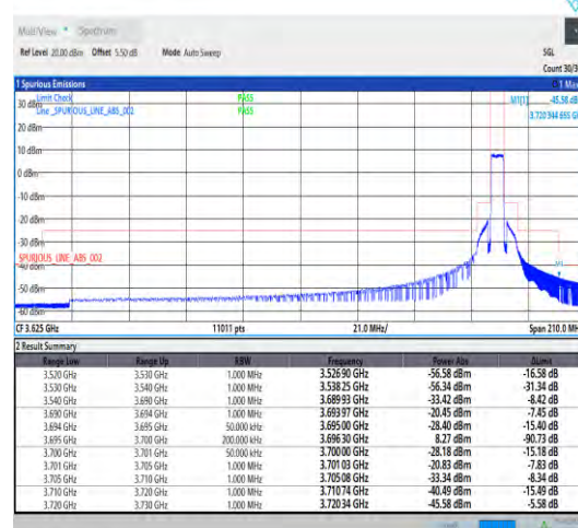
Band43 5MHz QPSK 44565 25RB#0
