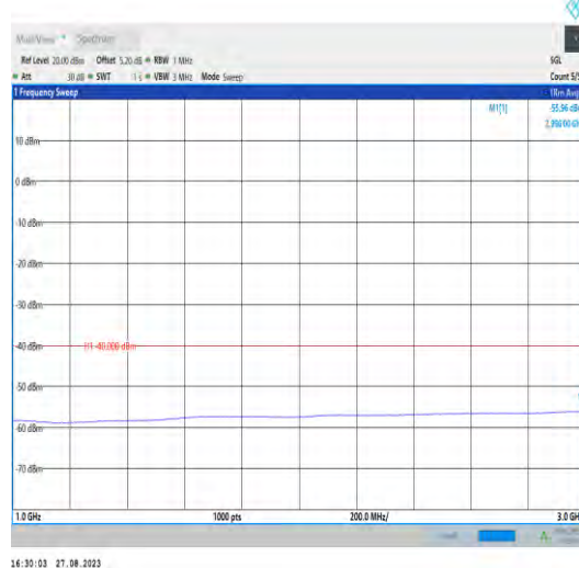
Band43_20MHz_QPSK_44090_1RB#0_1000~3000_1000~3000
