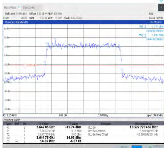
Band43-15MHz-QPSK-44090-75RB#0-PASS
