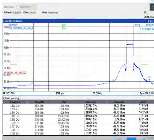
Band43_10MHz_QPSK_44540_50RB#0
