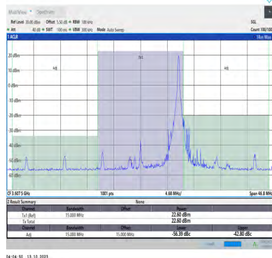
43(3600-3700)-15MHz-QPSK-43665-1RB#74-PASS
