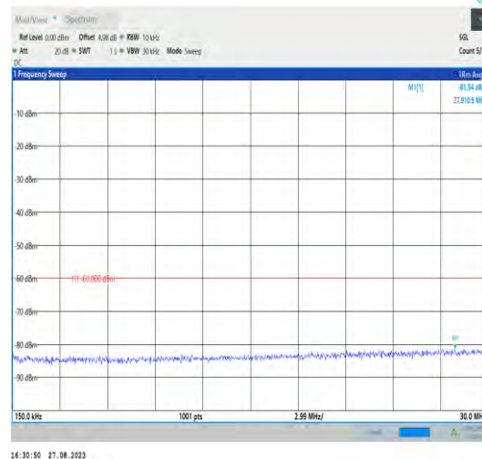
Band43_20MHz_QPSK_44490_1RB#0_0.15~30_0.15~30
