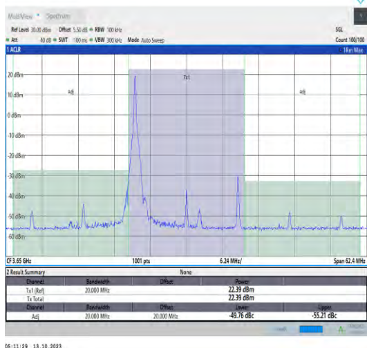
43(3600-3700)-20MHz-QPSK-44090-1RB#0-PASS
