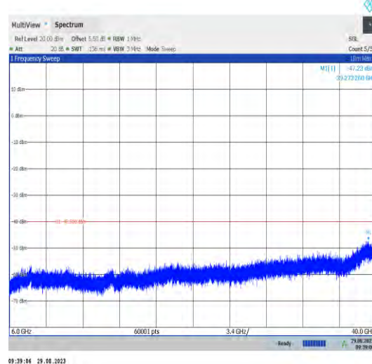
Band43_20MHz_QPSK_43690_1RB#0_6000~40000_6000~40000
