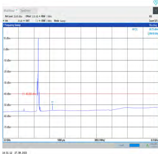
Band43_20MHz_QPSK_44490_1RB#0_3000~6000_30 00~6000
