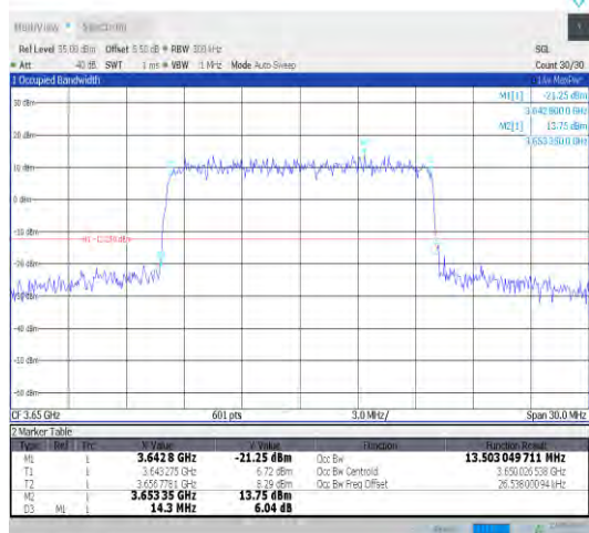
Band43-15MHz-16QAM-44090-75RB#0-PASS
