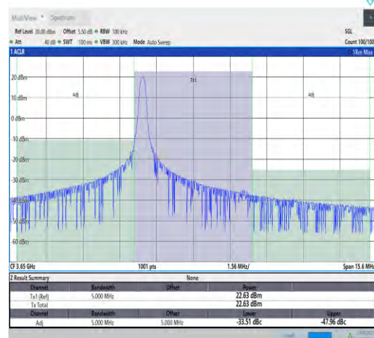
43(3600-3700)-5MHz-QPSK-44090-1RB#0-PASS
