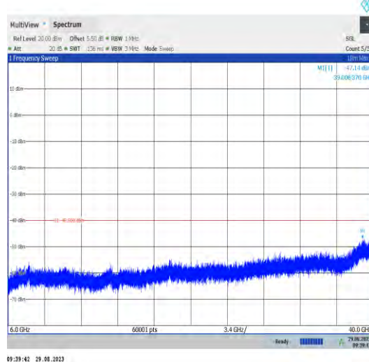
Band43_20MHz_QPSK_44490_1RB#0_6000~40000_600 0~40000
