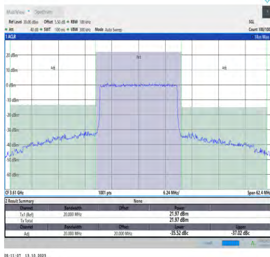
43(3600-3700)-20MHz-QPSK-43690-100RB#0-PASS
