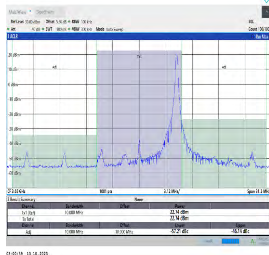
43(3600-3700)-10MHz-QPSK-44090-1RB#49-PASS
