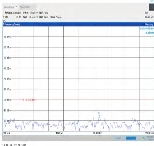
Band43_20MHz_QPSK_43690_1RB#0_0.009~0.15_0.0 09~0.15
