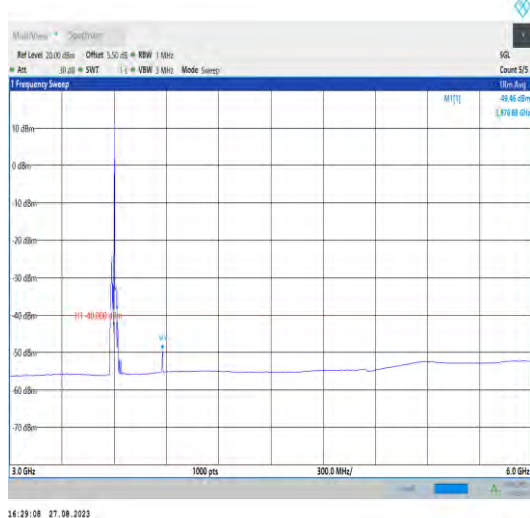
Band43_20MHz_QPSK_43690_1RB#0_3000~6000_3000~6000
