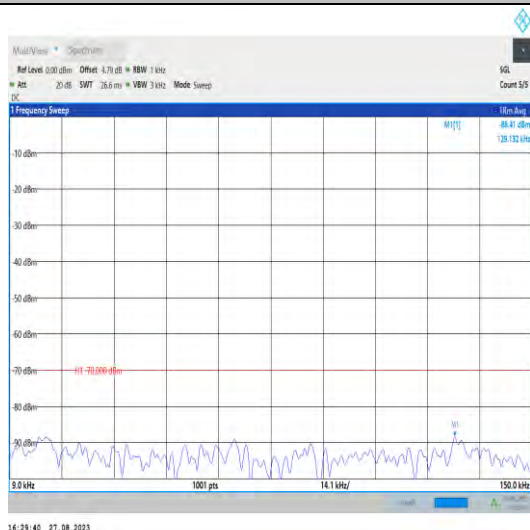
Band43_20MHz_QPSK_44090_1RB#0_0.009~0.15_0.009~0.15
