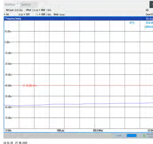
Band43_20MHz_QPSK_44490_1RB#0_1000~3000_1000~3000
