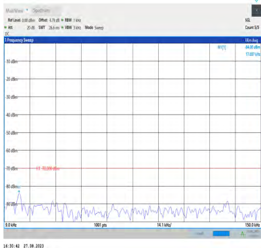
Band43_20MHz_QPSK_44490_1RB#0_0.009~0.15_0.09~0.15
