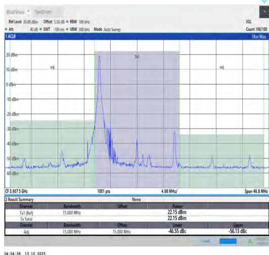
43(3600-3700)-15MHz-QPSK-43665-1RB#0-PASS
