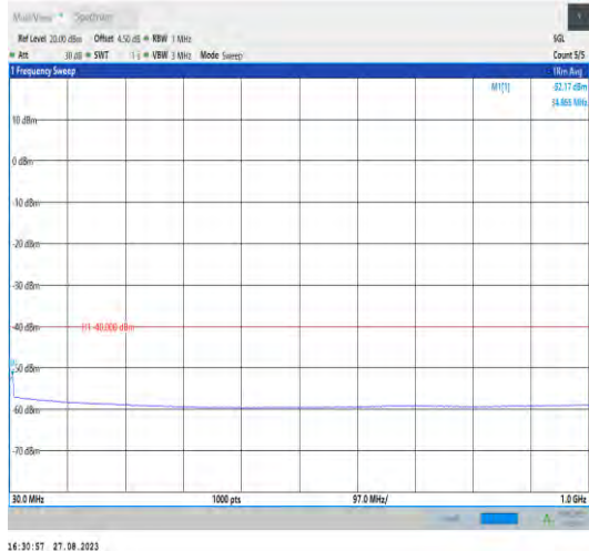
Band43_20MHz_QPSK_44490_1RB#0_30~1000_30~1000
