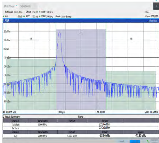
43(3600-3700)-5MHz-QPSK-43615-1RB#0-PASS
