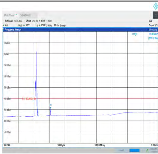
Band43_20MHz_QPSK_44090_1RB#0_3000~6000_3000~6000
