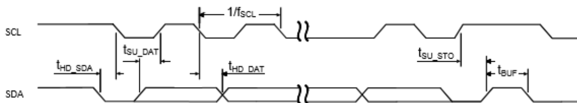
Figure 5: SCL/SDA timing
